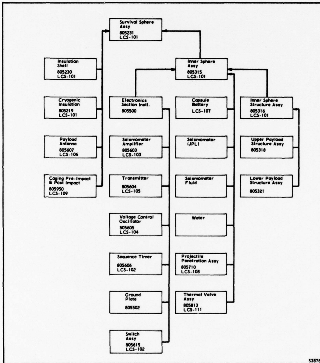
FIGURE 3.3 SURVIVAL SPHERE ASSEMBLY FLOW CHART
