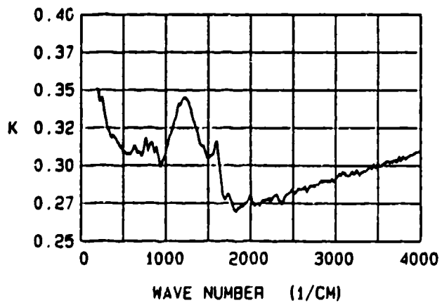
Figure 26. The infrared (180-4,000 \text{cm}^{-1} ) reflectance, refractive index N , and extinction coefficient K spectra of (NMSU) heated Diesel soot pellet.
