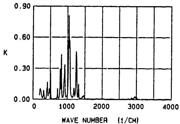
Figure 44. The infrared (180-4,000 \text{cm}^{-1} ) reflectance, refractive index N , and extinction coefficient K spectra of DMMP. The N and K spectra are from Kramers-Kronig analysis of the reflectance spectrum.
