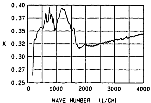
Figure 24. The infrared (180-4,000 \text{cm}^{-1} ) reflectance, refractive index N, and extinction coefficient K spectra of (NMSU) unheated Diesel soot pellet .
