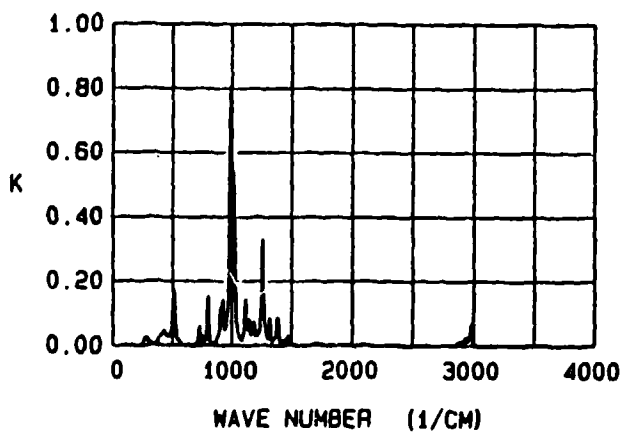
Figure 46. The infrared (180-4,000 \text{cm}^{-1} ) reflectance, refractive index N , and extinction coefficient K spectra of DIMP. The N and K spectra are from Kramers-Kronig analysis of the reflectance spectrum.
