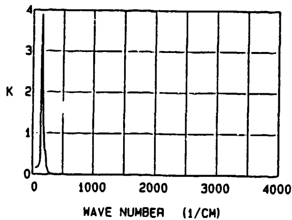
Figure 3. The infrared (60-4,000 \text{cm}^{-1} ) reflectance, refractive index N , and extinction coefficient K for potassium chloride.
