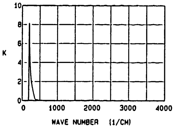
Figure 9. The infrared ( 60-4,000 \text{ cm}^{-1} ) reflectance, refractive index N , and extinction coefficient K for barium fluoride.
