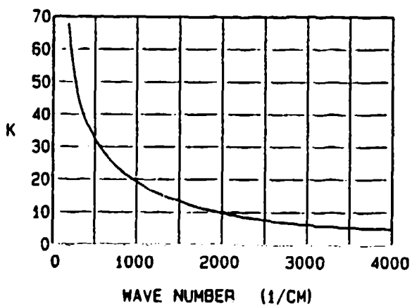
Figure 36. The infrared (180-4,000 \text{cm}^{-1} ) reflectance, refractive index N, and extinction coefficient K spectra of zirconium .
