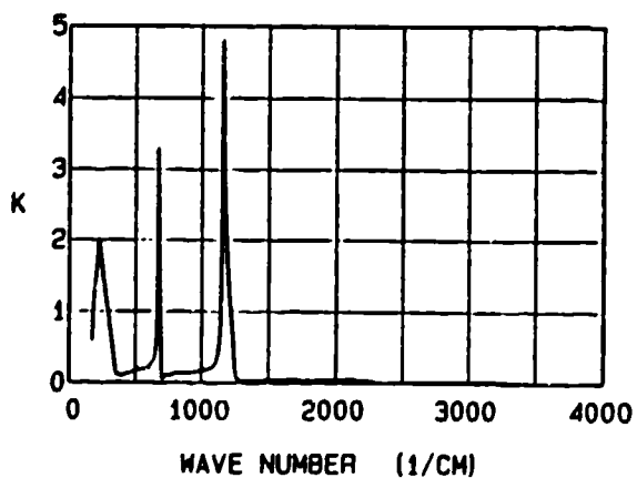
Figure 29. The infrared (180-4,000 \text{cm}^{-1} ) reflectance, refractive index N, and extinction coefficient K spectra of anhydrite, E//X.
