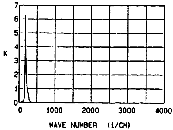
Figure 1. The Infrared (60-4,000 \text{cm}^{-1} ) reflectance, refractive index N, and extinction coefficient K for sodium chloride.
