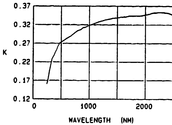
Figure 25. The uv-vis-nir (220-2,500 nm) reflectance, refractive index N, and extinction coefficient K spectra of (NMSU) unheated Diesel soot pellet.
