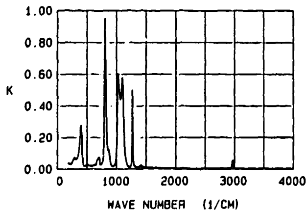
Figure 42. The infrared (180-4,000 \text{cm}^{-1} ) reflectance, refractive index N , and extinction coefficient K spectra of SF-96. N and K were determined by Kramers-Kronig analysis of the reflectance spectra .
