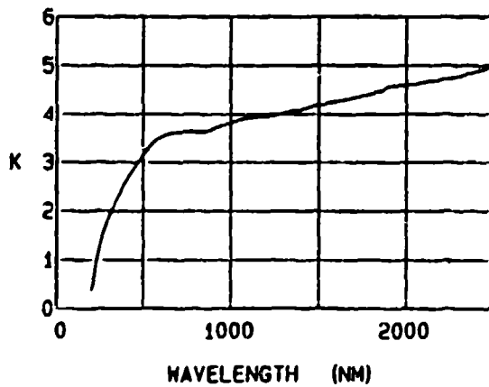
Figure 37. The uv-vis-nir (200-2,500 nm) reflectance, refractive index N, and extinction coefficient K spectra of zirconium .
