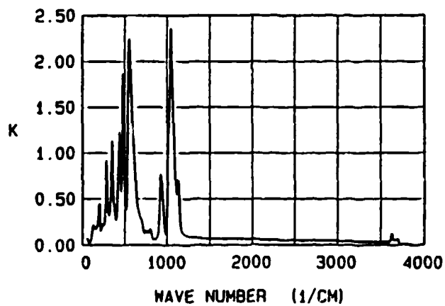
Figure 17. The infrared (50-4,000 \text{cm}^{-1} ) reflectance, refractive index N, and extinction coefficient K spectra for colloidal kaolin pellets.
