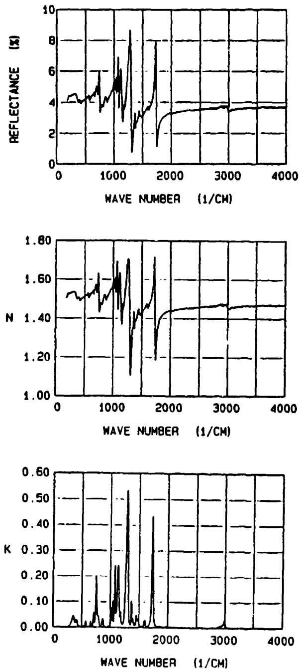
Figure 48. The infrared ( 180\text{--}4,000\text{ cm}^{-1} ) reflectance, refractive index N , and extinction coefficient K spectra of DEP. The N and K spectra are from Kramers-Kronig analysis of the reflectance spectrum.
