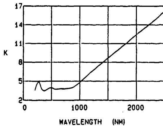
Figure 35. The uv-vis-nir (200-2,500 nm) reflectance, refractive index N, and extinction coefficient K spectra of molybdenum.
