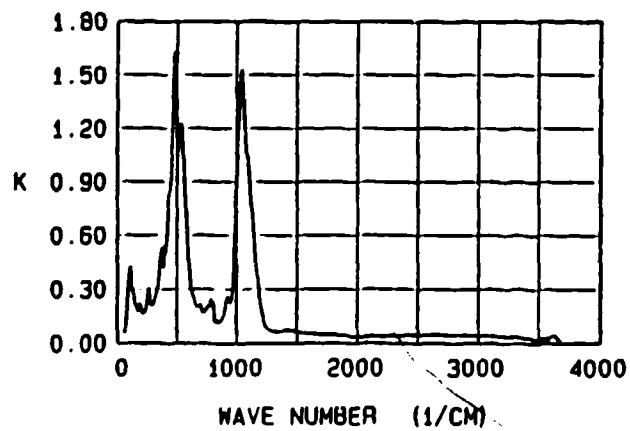
Figure 19. The infrared (50-4,000 \text{cm}^{-1} ) reflectance, refractive index N, and extinction coefficient K spectra for colloidal illite pellet .
