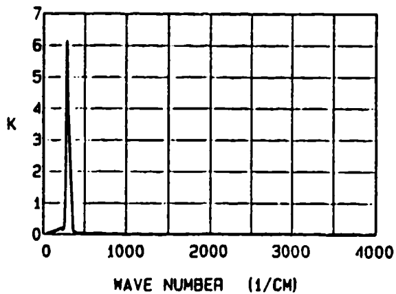
Figure 11. The infrared (60-4,000 \text{cm}^{-1} ) reflectance, refractive index N, and extinction coefficient K for zinc sulfide.
