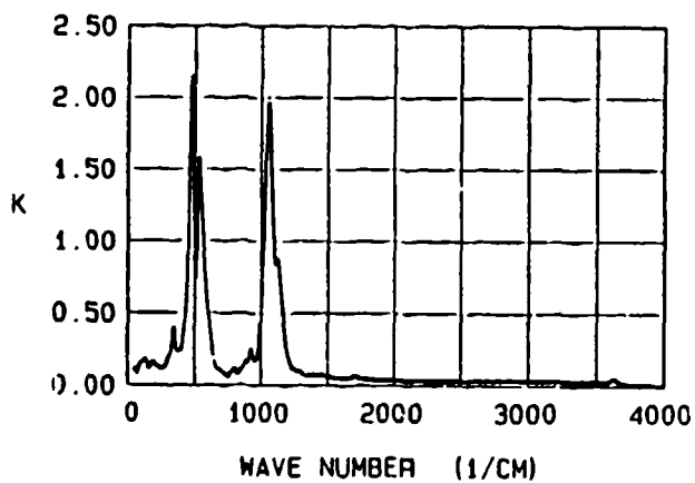
Figure 15. The infrared (50-4,000 \text{cm}^{-1} ) reflectance, refractive index N, and extinction coefficient K for colloidal montmorillonite pellets .
