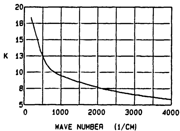
Figure 38. The infrared (180-4,000 \text{cm}^{-1} ) reflectance, refractive index N, and extinction coefficient K spectra of manganese .
