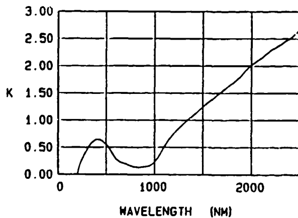
Figure 41. The uv-vis-nir (200-2,500 nm) reflectance and tentative values of refractive index N and extinction coefficient K spectra of zinc .
