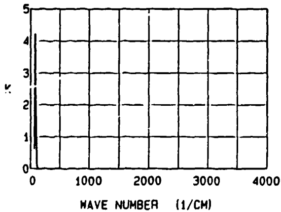
Figure 7. The infrared ( 67-4,000 \text{ cm}^{-1} ) reflectance, refractive index N , and extinction coefficient K for cesium bromide .
