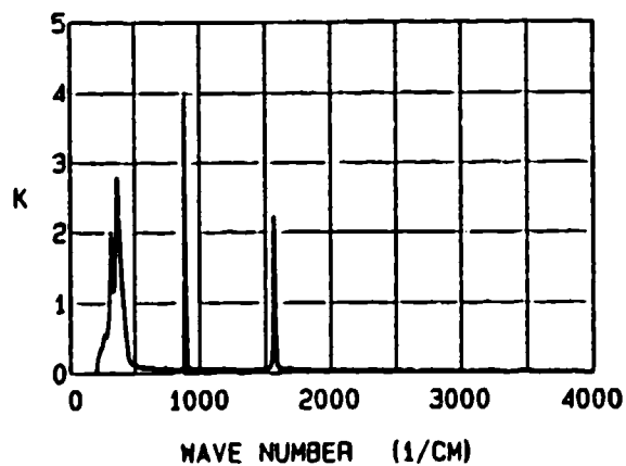
Figure 32. The infrared ( 180-4,000 \text{ cm}^{-1} ) reflectance, refractive index N , and extinction coefficient K spectra of dolomite, E/C.
