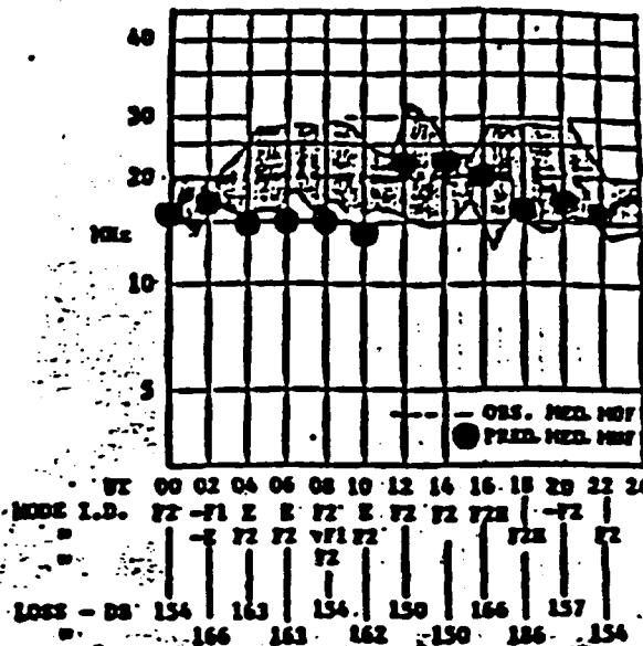
FIGURE 11b- AMBCOM PREDICTION FOR ANDOYA-COLLEGE PATH, MAY, 1964
