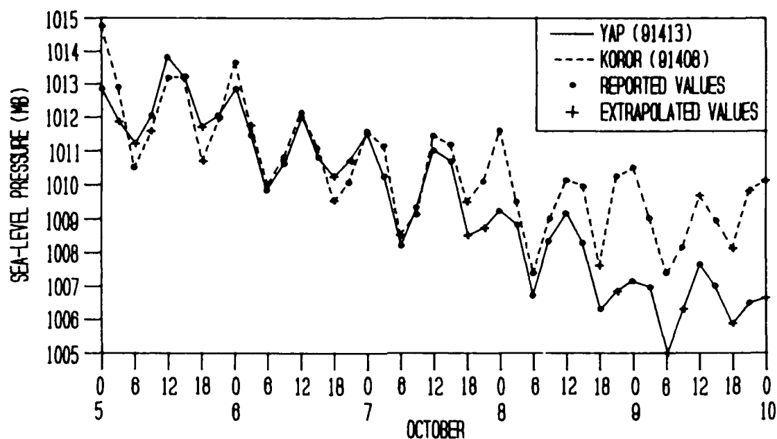
Figure 3-19-2. A plot of the surface pressures for Yap and Koror for the time period 050000Z to 100000Z October (missing values are extrapolated for continuity purposes). Although pressures were dropping at both stations, the lower surface pressures and more rapid falls at Yap indicated the low pressure center was passing close by.
