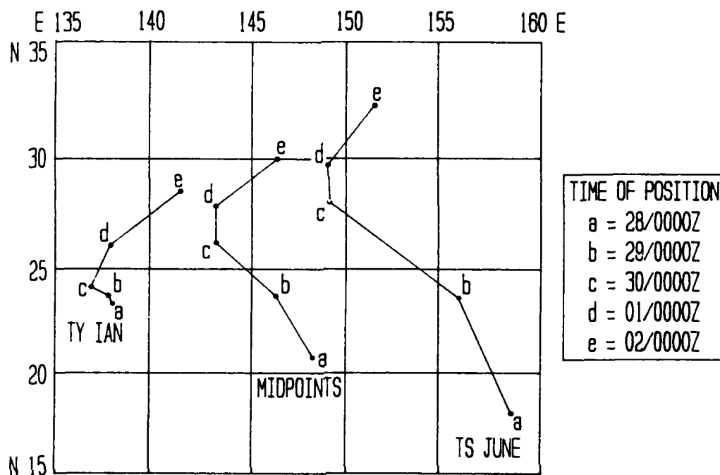
Figure 3-16-4. Plot of the slight binary interaction between Ian and June (18W) showing their individual tracks and the path of the midpoints.
