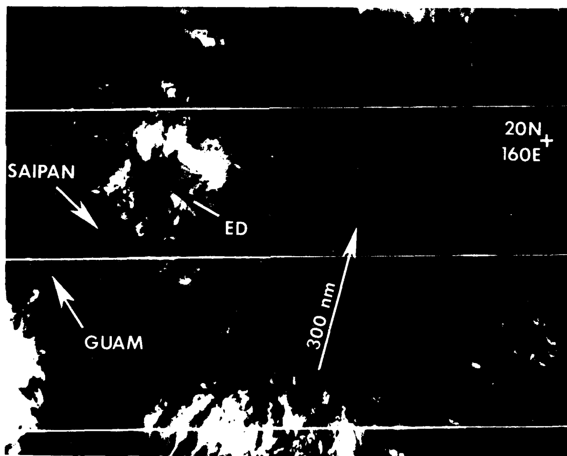
Figure 3-12-3. Tropical Storm Ed (12W) after the system had shed its central dense overcast (270445Z August NOAA visual imagery).
