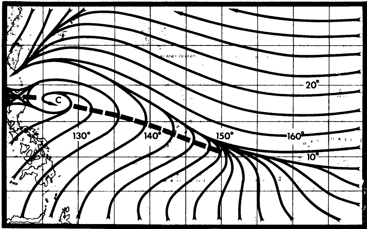
Figure 3-15-1. Gradient-level wind climatology for September (Sadler, et al, 1987).
