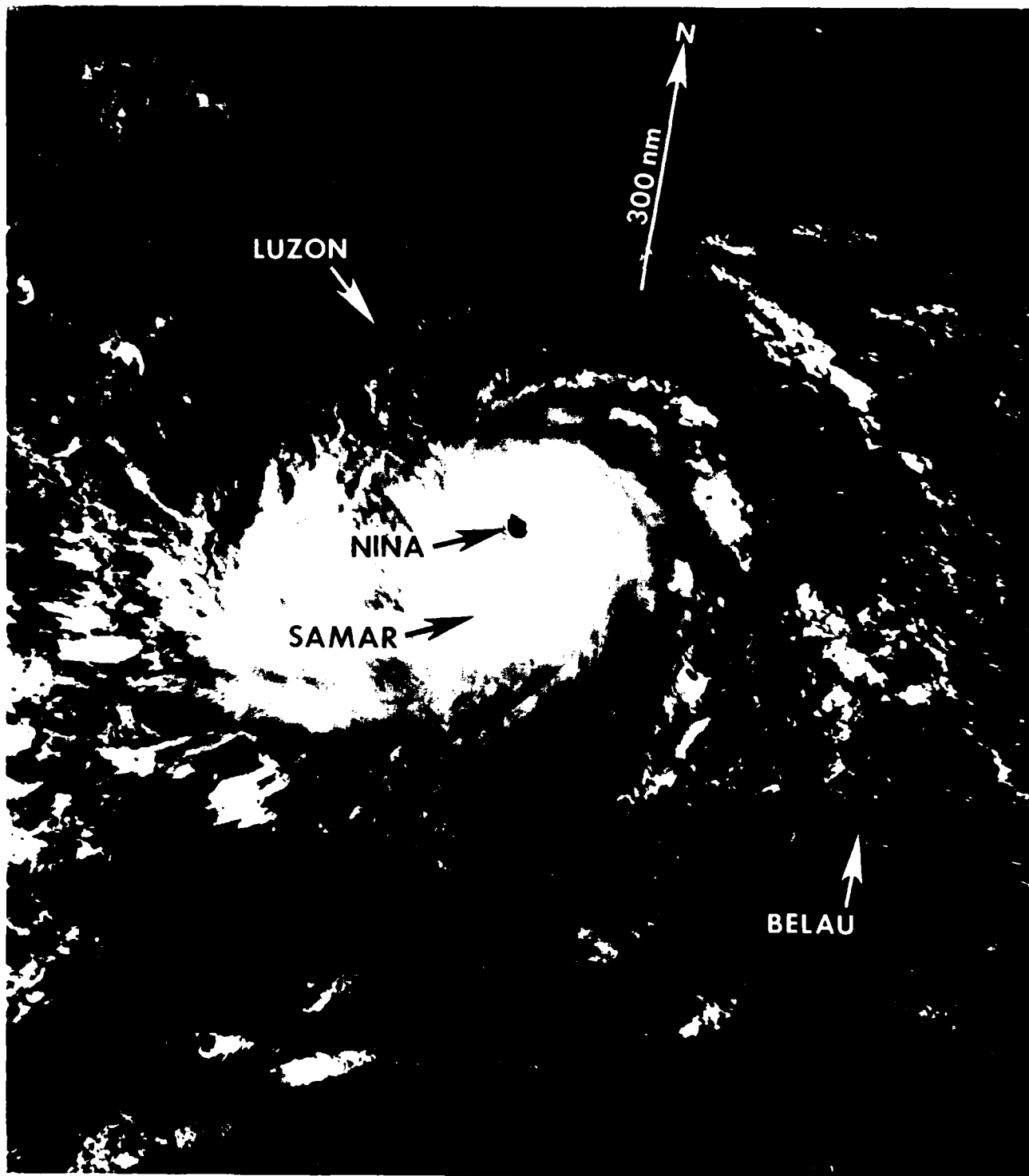
Figure 3-22-6. Matching infrared image for visual in Figure 3-22-5 (250701Z November NOAA infrared imagery).
