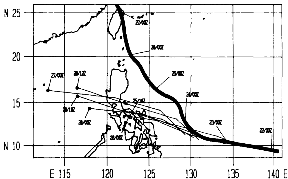
Figure 3-08-4. Initial OTCM 72-hour guidance for Alex indicated the system would remain south of the subtropical ridge and move across the Philippine Islands. Alex's best track is also shown for comparison.
