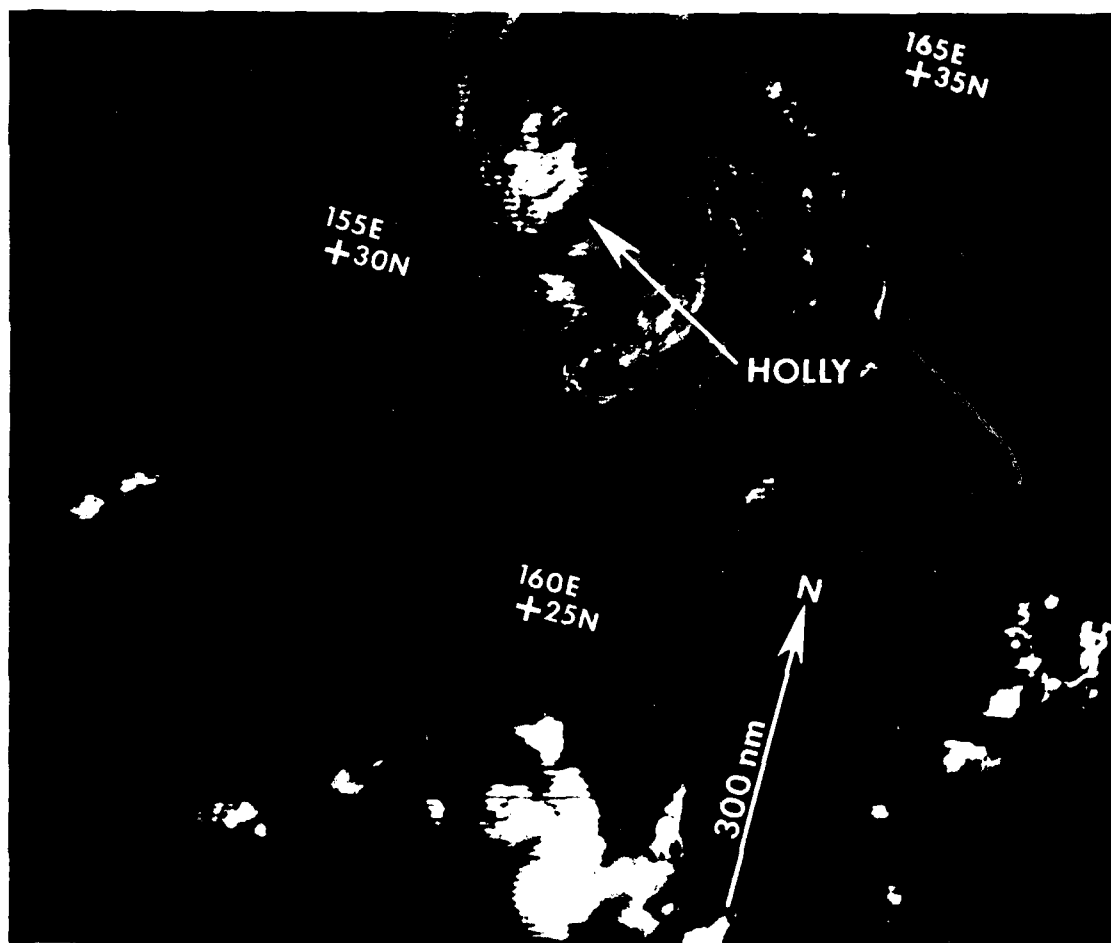
Figure 3-15-6. The subtropical remains of Holly (162227Z September DMSP visual imagery).
