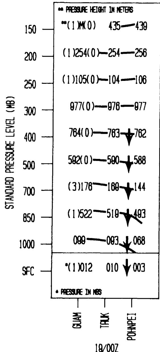
Figure 3-22-1. Heights of the standard pressure levels and surface pressure at Pohnpei (WMO 91348), Truk (WMO 91334) and Guam (WMO 91217) at 190000Z. At this time, Nina was 230 nm (426 km) southeast of the island of Pohnpei. In comparison with Truk and Guam, the lower heights at Pohnpei (WMO 91348) at the 400 mb level and below are due to the approaching tropical cyclone.
