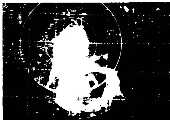
Figure 3-08-8. The tightly curved rainband and eye wall of Typhoon Alex as seen by radar from Hualien, Taiwan (WMO 46699) at 261400Z July (Photograph courtesy of Central Weather Bureau, Taipei,
