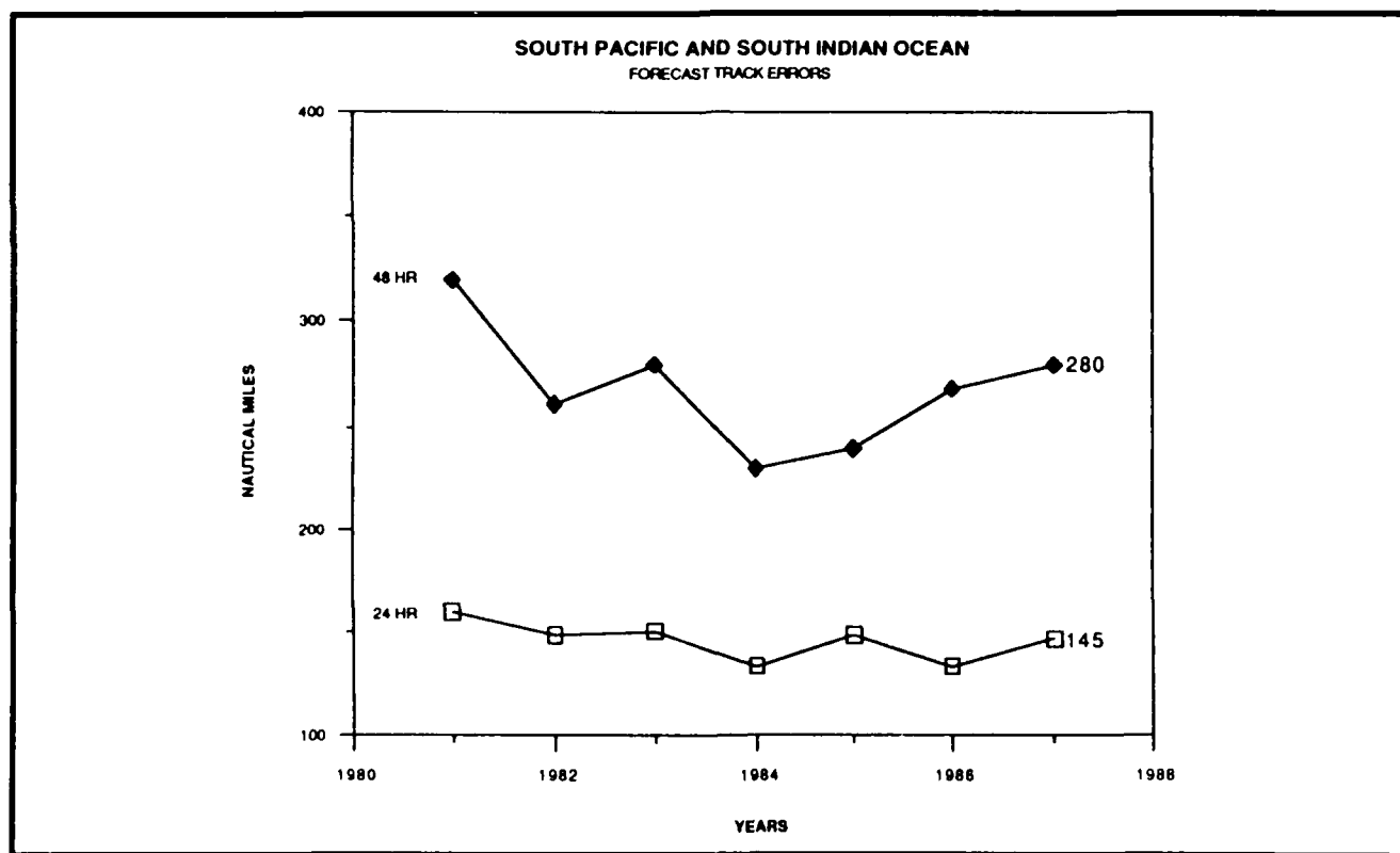
Figure 5-5. Annual mean forecast errors (in nm) for all tropical cyclones in the South Pacific and South Indian Oceans.
