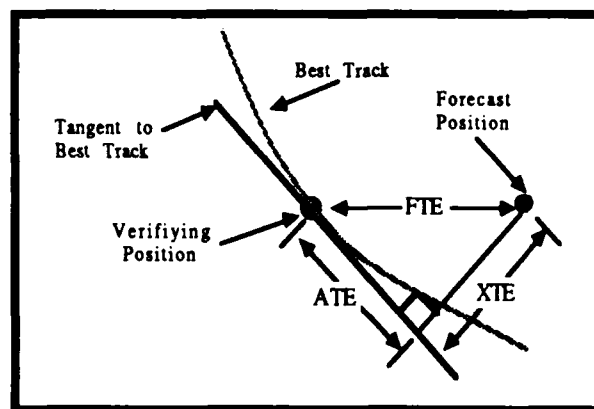
Figure 5-1. Definition of cross-track error (XTE), along-track error (ATE), and forecast track error (FTE). In this example, the XTE is positive (to the right of the Best Track) and the ATE is negative (behind or slower than the Best Track)..
