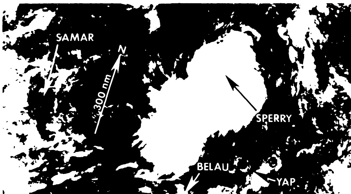
Figure 3-04-2 Typhoon Sperry with an intensity of 65 kt (33 m/sec) just prior to peaking (280047Z June DMSP satellite imagery).
