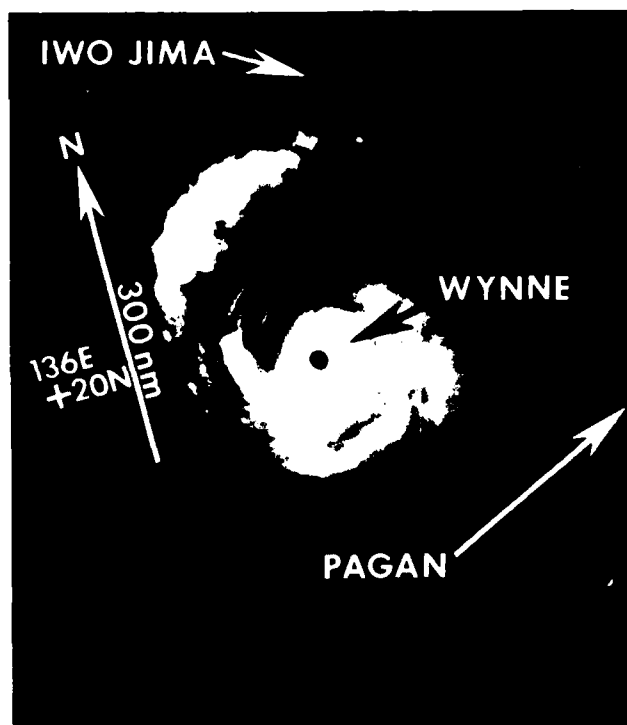
Figure 3-07-4. Midget Typhoon Wynne near maximum intensity. Note the well-defined 15 nm (28 km) eye (261815Z July NOAA infrared imagery).
