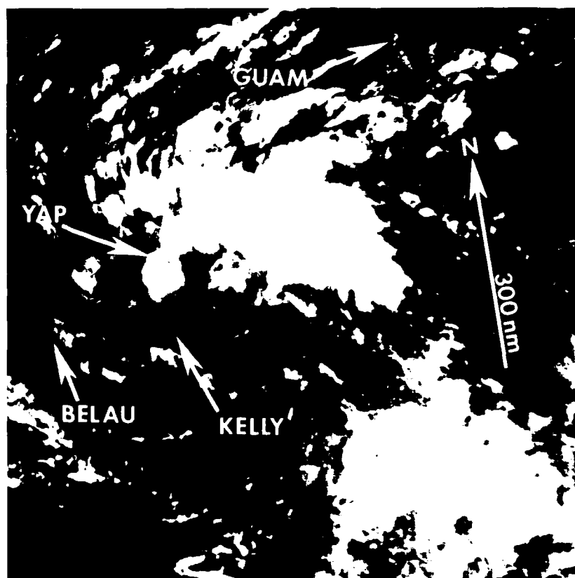
Figure 3-19-1. Moonlight visual imagery showing Typhoon Kelly at an early stage of development (071243Z October DMSP visual imagery).
