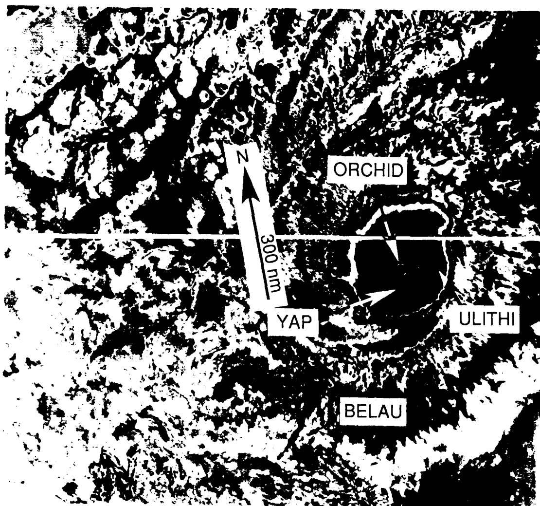
Figure 3-01-4. Enhanced infrared (EIR) imagery of Typhoon Orchid (01W) near maximum intensity. Note the small well-defined eye (102259Z January NOAA infrared imagery).
