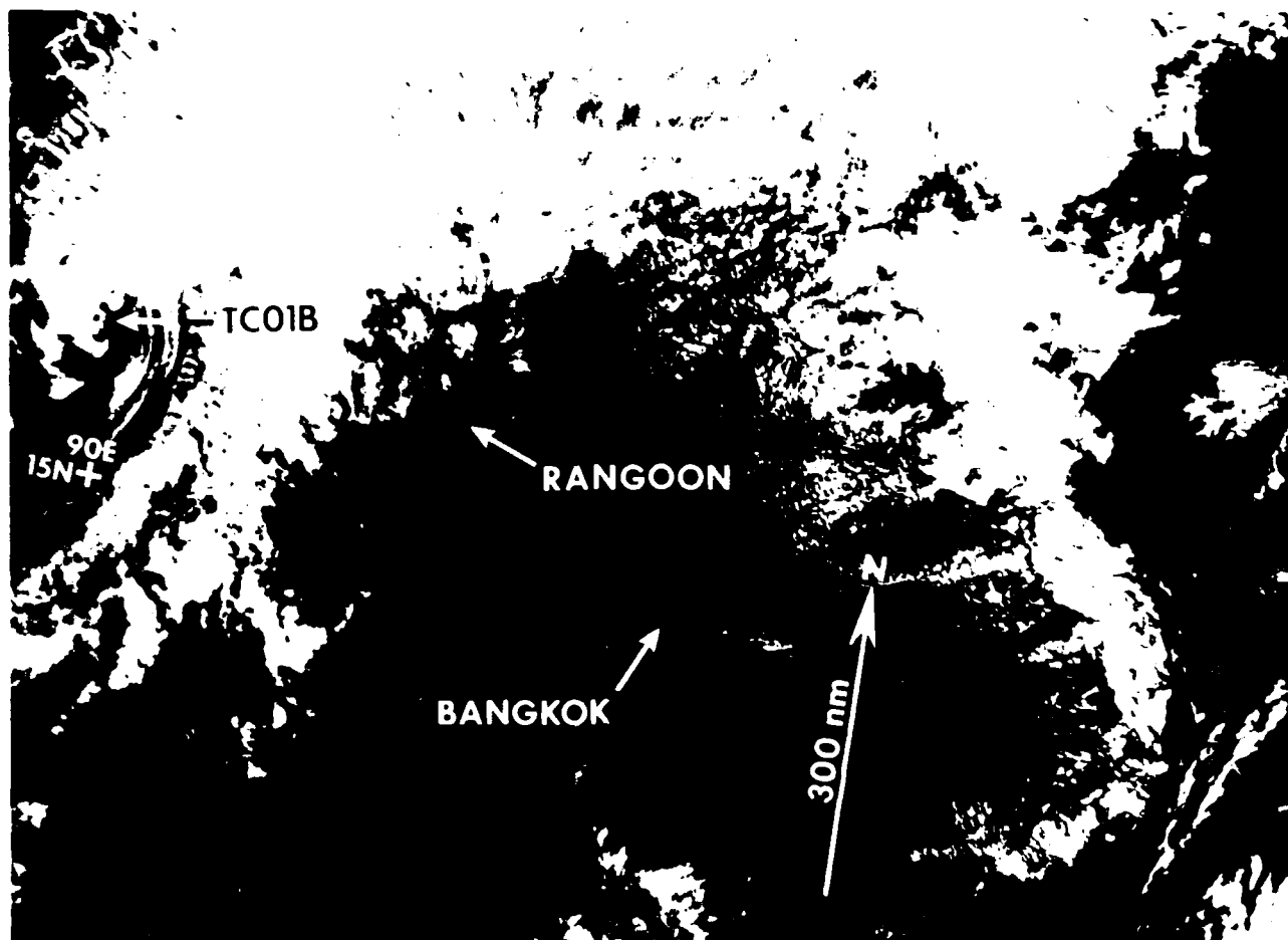
Figure 3-01B-1. Tropical Cyclone 01B was the first significant tropical cyclone to form in the Bay of Bengal during 1987. It was detected as an amorphous area of convection about 500 nm (926 km) east of Sri Lanka on the 29th of January and was noted on the 301800Z Significant Tropical Weather Advisory (ABIO TGTW). Satellite imagery at that time showed upper-level anticyclonically curved outflow over a weak, low-level circulation. Within the next 24 hours, the organization and amount of convection steadily increased. A Tropical Cyclone Formation Alert was issued at 311900Z. Satellite imagery showed convective banding had continued to increase, but sparse synoptic data showed no low surface pressures. At 0000Z on February 1st, the first warning was issued with the appearance of a central dense overcast and unrestricted outflow in all quadrants. The system then tracked steadily northeastward. The intensity peaked at 55 kt (28 m/sec) at 020600Z as the system began interaction with upper-level southwesterlies, which sent a long plume of cirrus northeastward across Burma. A partially exposed low-level circulation center became apparent at 030000Z, as increased vertical wind shear from the southwesterlies aloft stripped away the central cloudiness. Six hours later the low-level vortex was fully exposed (see above imagery). At 031200Z, JTWC issued the final warning on the 30 kt (15 m/sec) weakening tropical cyclone. The remnants of Tropical Cyclone 01B continued to track toward the northeast and dissipation occurred after it made landfall on February 4th over the northwest coast of Burma (030805Z February NOAA visual imagery).
