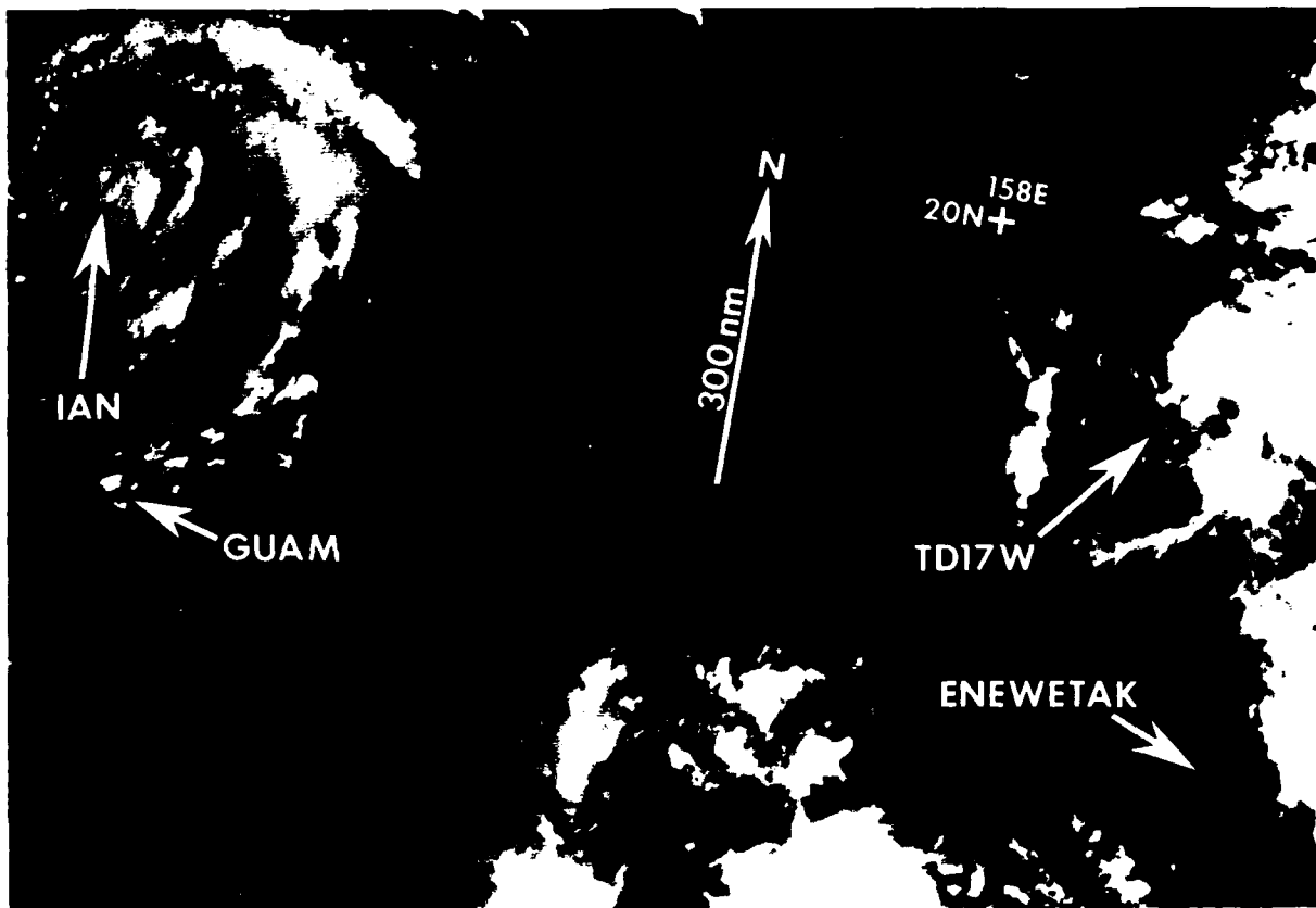
Figure 3-17-1. Tropical Depression 17W slowly developed from a tropical disturbance 250 nm (463 km) north of the Marshall Islands during the same period JTWC was warning on Typhoon Ian (16W). It was first detected on satellite imagery on the 23rd of September and mentioned on the Significant Tropical Weather Advisory (ABPW TGTW) as a new suspect area at 0600Z. JTWC issued a Tropical Cyclone Formation Alert nearly 24-hours later at 240330Z when this system displayed increased convective organization. Maximum sustained surface winds, at that time, were estimated at 15 to 25 kt (8 to 13 m/sec). The first warning on Tropical Depression 17W was issued at 241800Z based on satellite intensity estimate (Dvorak, 1984) of 35 kt (18 m/sec) winds at the surface. A well-established mid-level ridge was located to the northeast of Tropical Depression 17W. At the same time, an eastward-progressing, mid-latitude trough to the north was beginning to influence the system. This trough continued to suppress Tropical Depression 17W's development even after it had passed to the northeast of the disturbance. Concurrently, Typhoon Ian's (16W) upper-level outflow (at the left of the image) restricted Tropical Depression 17W's outflow in the northwest quadrant. This combination of factors appears to have stopped further intensification and induced dissipation over water. The last warning was issued on the 26th of September at 0600Z. The satellite image above shows Tropical Depression 17W shortly before the second warning was issued, while it was at its maximum intensity of 30 kt (15 m/sec) and 960 nm (1778 km) east-southeast of Typhoon Ian (16W). A partially exposed low-level circulation is visible slightly west of the heaviest convection (242305Z September DMSP visual imagery).
