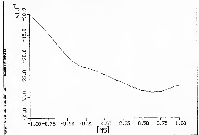
Figure D.18. e'_{32} At ZREF = - 7.524 cm
