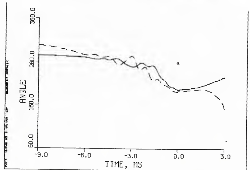
Figure D.4. Phase Angle, deg.
