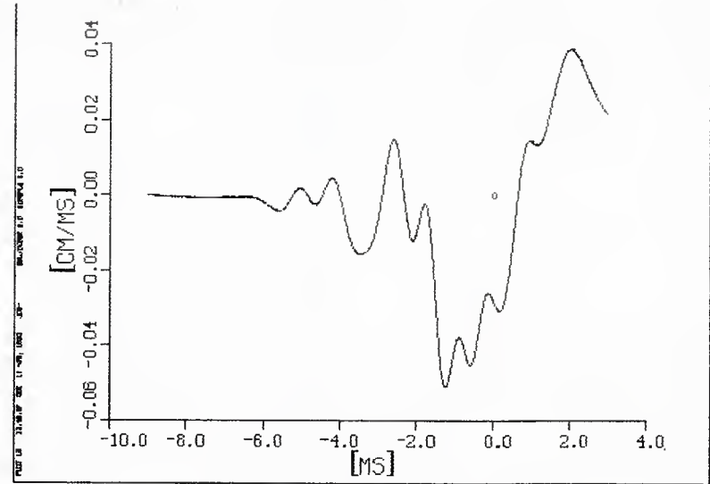
Figure D.15. Vertical Velocity At ZREF = .0, cm/ms
