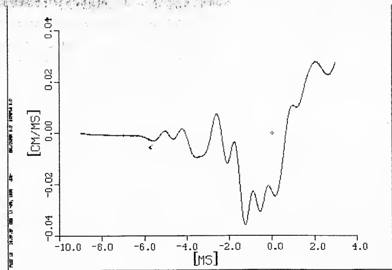
Figure D.24. e'_{32} At ZREF = - 7.524 cm
