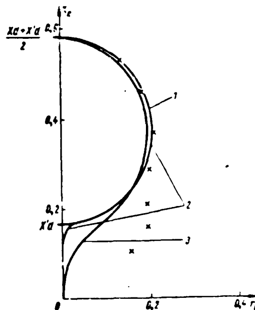
Fig. 2. Comparison of theoretical and determined (experimentally) boundaries of self-excitation for a generator with parameters: (x_d = 1; x'_d = 0.17; T_2 = \omega 0.12) e.s; 1 - T_2 = (10-100) e.s; 2 - T_2 = \omega e.s; 3 - T_2 = 0.1 e.s; 4 - T_2 = 0.01 e.s.
