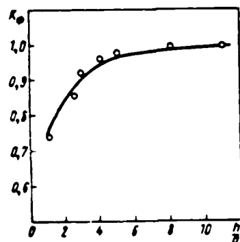
Fig. 1. Dependence of k_\varphi = f(\frac{h}{a}) when b/a=2.6 ; ———— - calculation curve.
