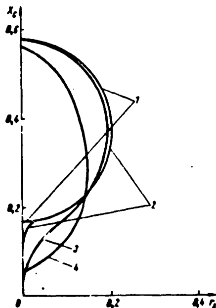
Fig. 1. Regions of self-excitation plotted according to the characteristic equation (2) for a machine having the following parameters: 1 - T_2 = (10-100) e.s; 2 - T_2 = \omega e.s; 3 - T_2 = 0.1 e.s; 4 - T_2 = 0.01 e.s.
