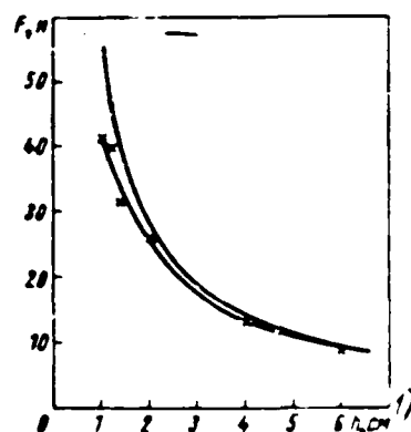
Fig. 2. Curves of forces for b/a=2.6 and current of 3 kA. Key: 1) cm.
