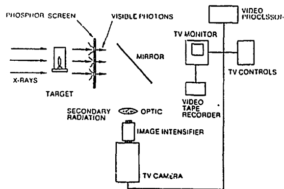
Fig. 4 Schematic of real time radiography test facility.
