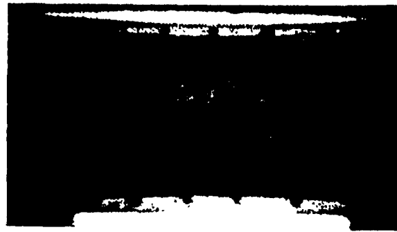
Fig. 10 Radiograph of closed LMC showing dense product separation at t=150 s.
