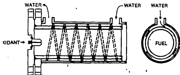
Fig. 1 Liquid metal combustor. Components as noted. Coolant flow paths are indicated.
