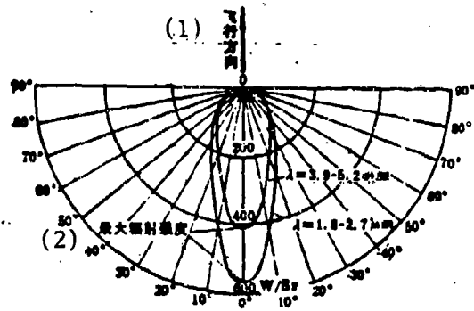
Fig. 9 Infrared radiation characteristics of a certain jet plane Key: (1) Flight direction; (2) Maximum radiation intensity.
