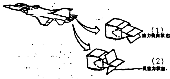
Fig. 2 Double-throat type twin-nozzle Key: (1) Propulsion in direction-changing state; (2) Counter-propulsion state
