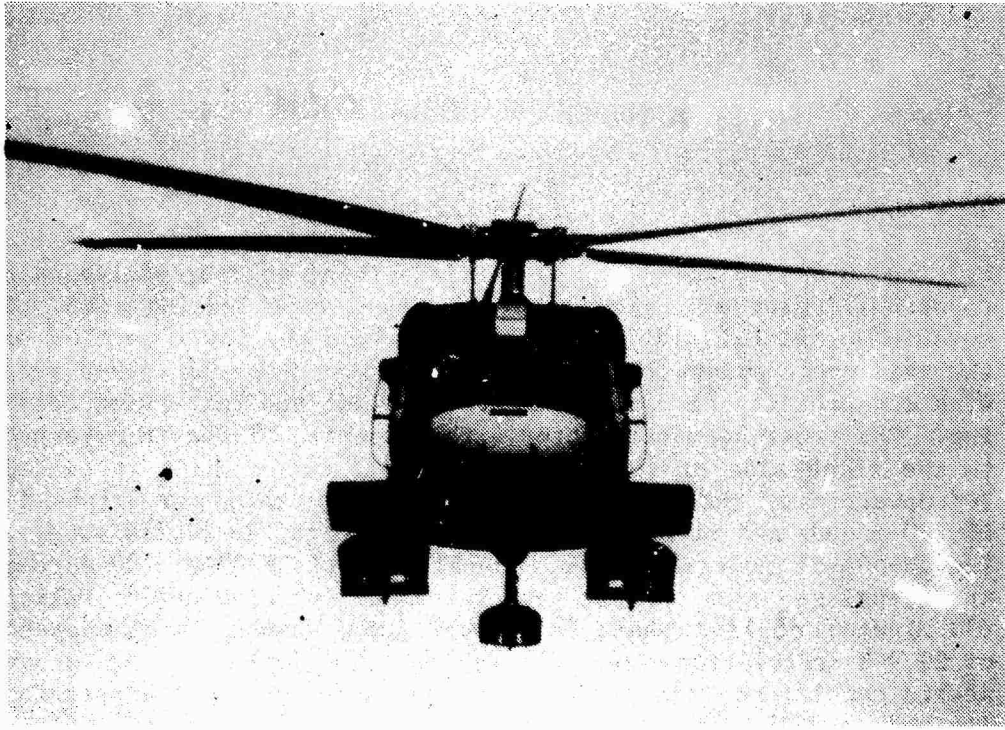
Photo 1. Front View - UH-60A Helicopter with Skis Installed
