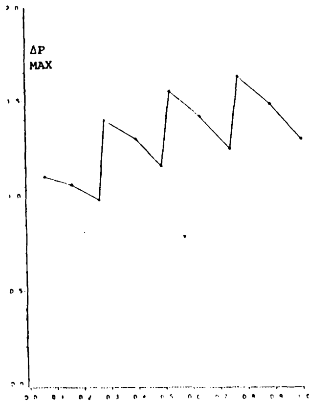
Figure 1: Pressure Residue vs. the Global Iteration Number.
