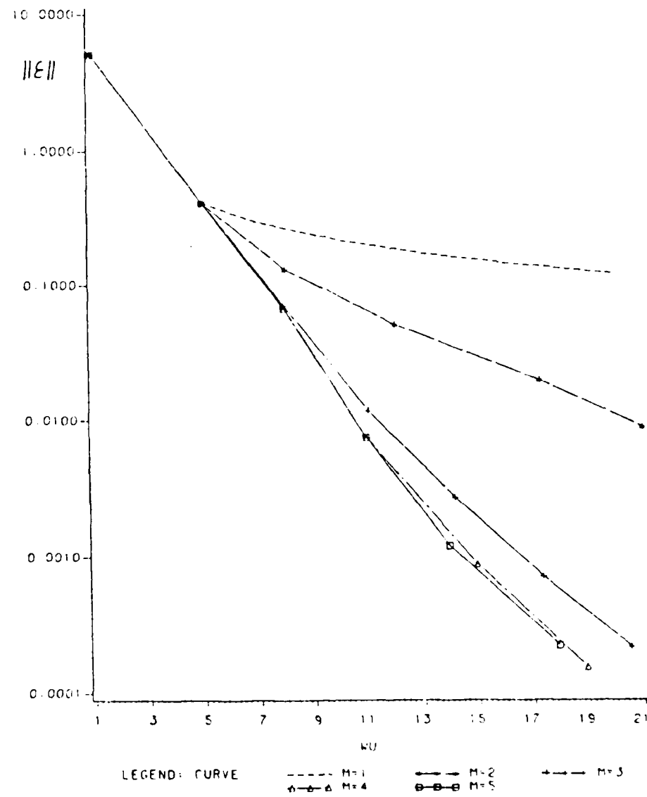
Figure 7: Convergence history, semi-infinite flat plate.
