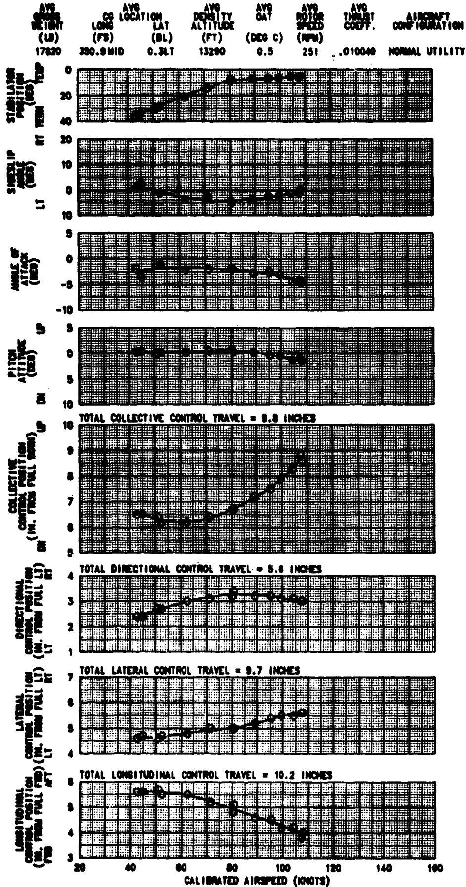
FIGURE 12 CONTROL POSITIONS IN TRIMMED FORWARD FLIGHT UN-00A USA S/N 84-23883
