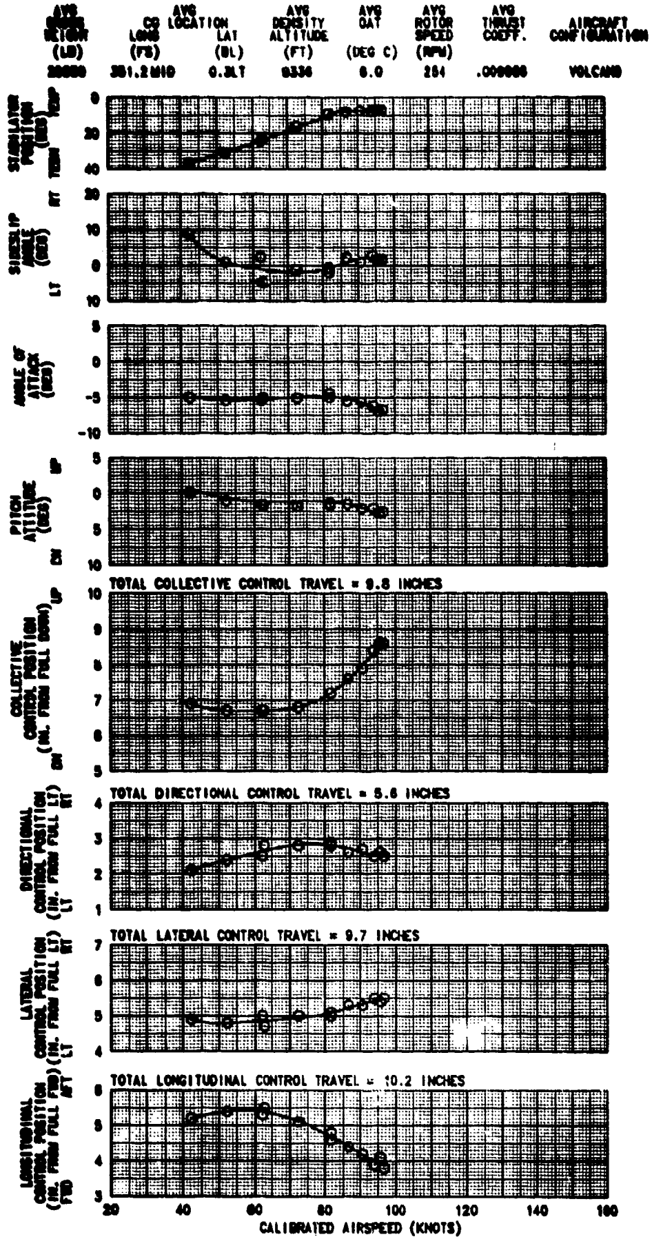
FIGURE 15 CONTROL POSITIONS IN TRIMMED FORWARD FLIGHT UH-60A USA S/N 84-23063
