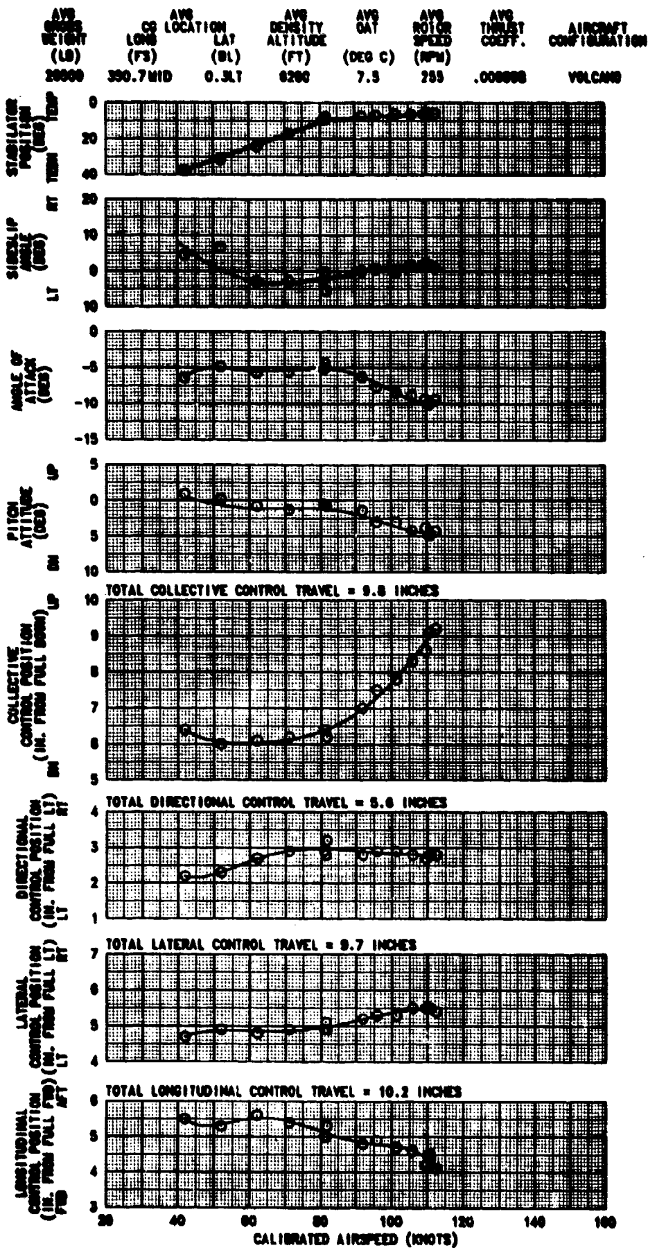
FIGURE 14 CONTROL POSITIONS IN TRIMMED FORWARD FLIGHT UH-60A USA S/N 84-23983
