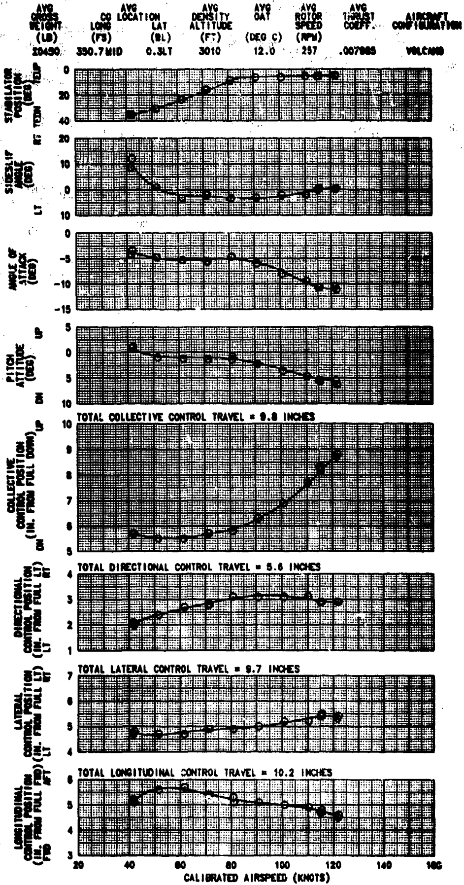
FIGURE 13 CONTROL POSITIONS IN TRIMMED FORWARD FLIGHT UH-60A USA S/N 84-23933
