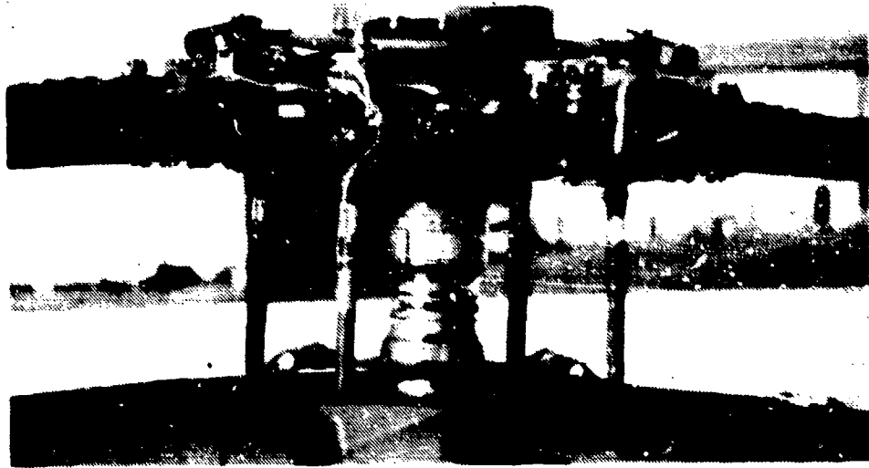
Photo 23. Main Rotor Instrumentation and Slip Ring Installation
