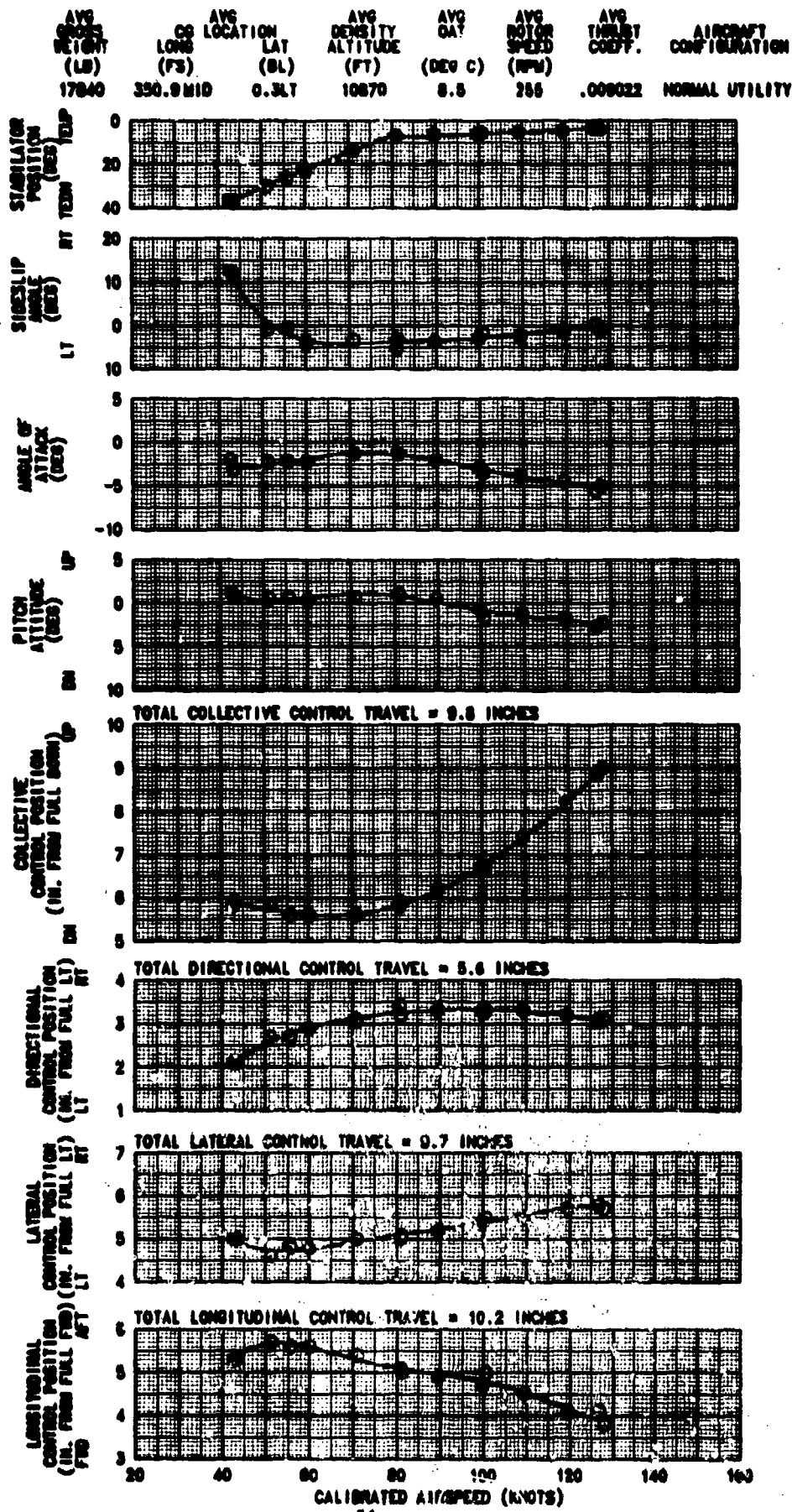
FIGURE 11 CONTROL POSITIONS IN TRIMMED FORWARD FLIGHT UH-60A USA S/N 84-23963
