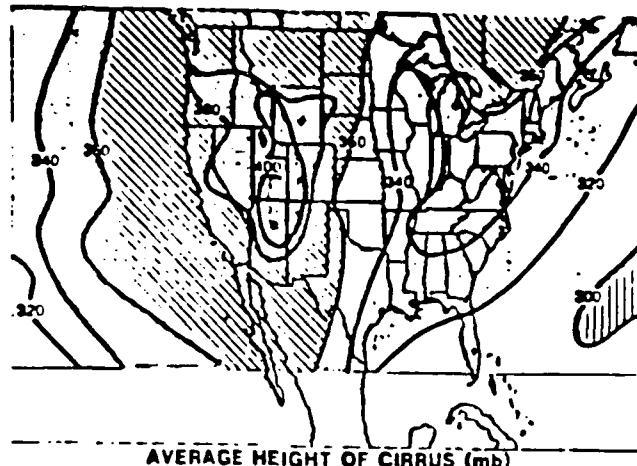
AVERAGE HEIGHT OF CIRRUS (mb)
