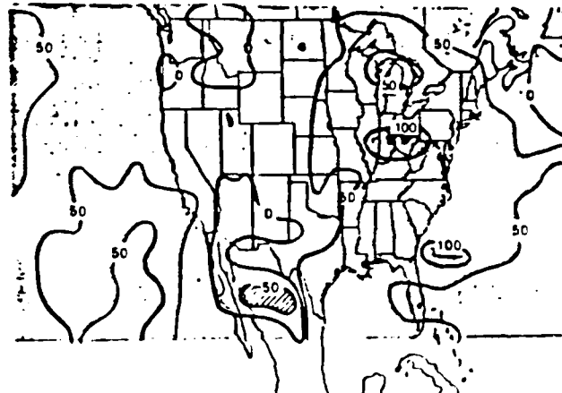
SEASONAL CHANGE IN HEIGHT OF CIRRUS (mb)
