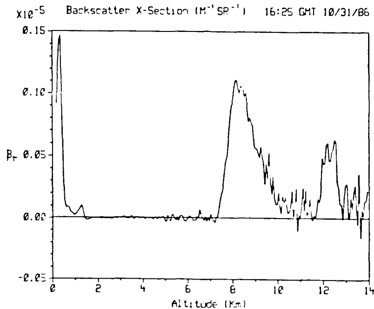
Fig. 1 Autumn "warr sector" cirrus backscatter cross section profile. The two layer structure is often observed in this type of formation.
