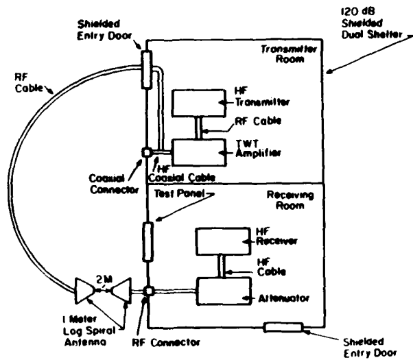
REFERENCE MEASUREMENT TEST SETUP FOR I METER LOG SPIRAL ANTENNA
