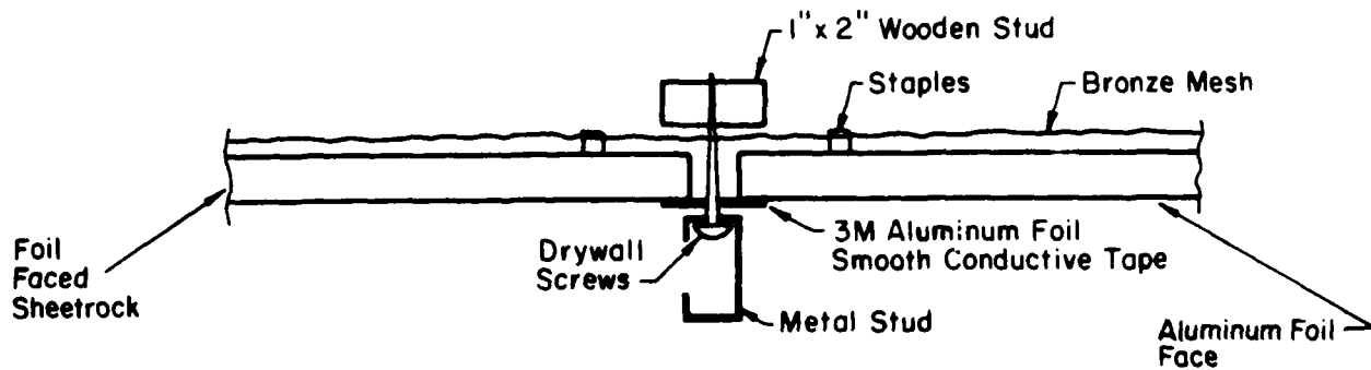
Figure 12. Diagram of seam design #1.
