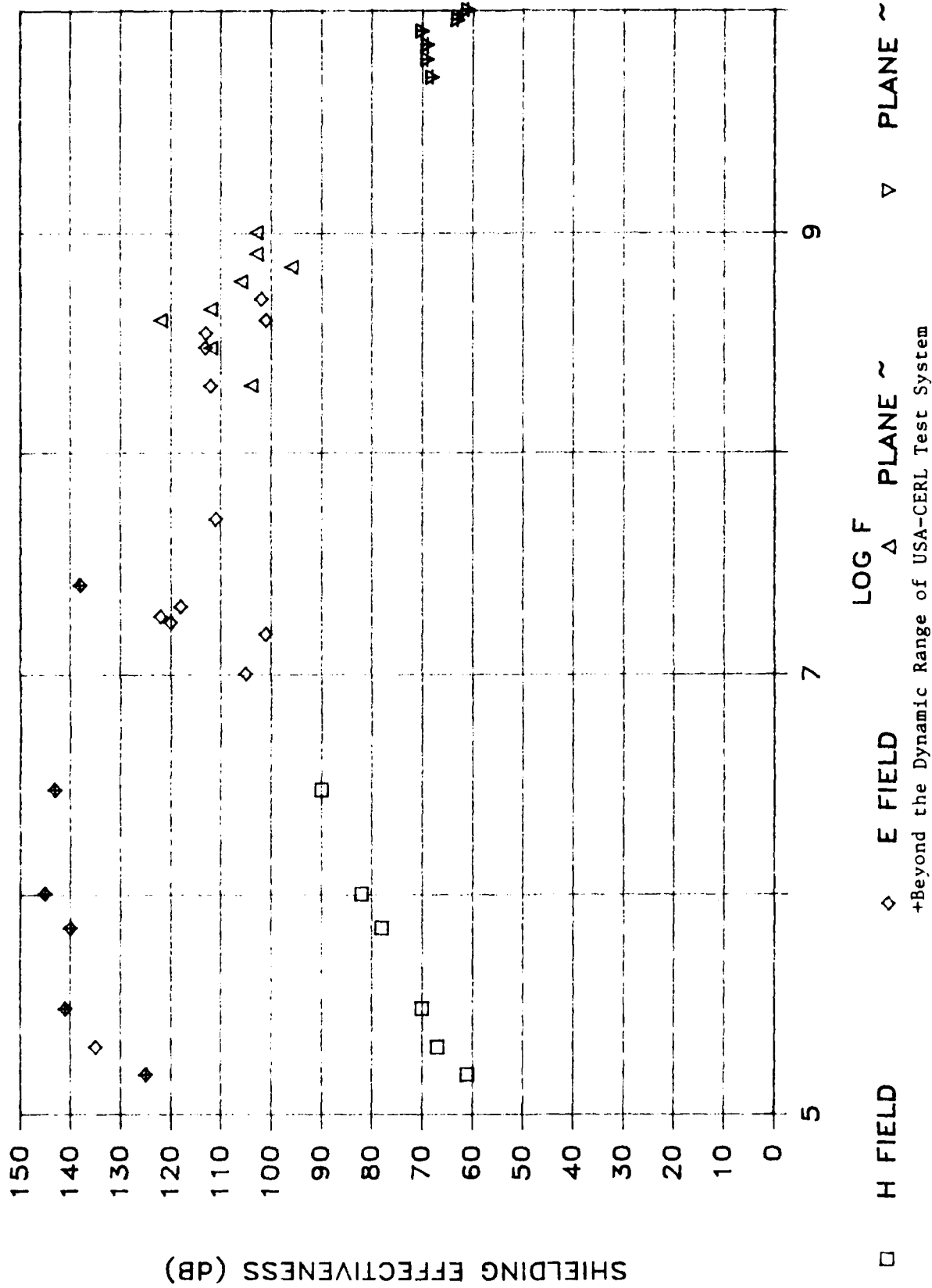
Figure A5. Shielding effectiveness vs. log of frequency for bronze mesh composite.
