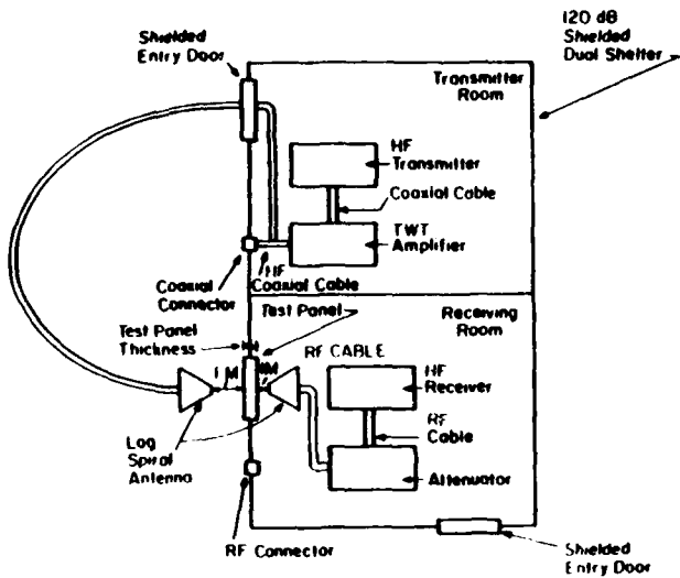
SIGNAL MEASUREMENT TEST SETUP FOR I METER LOG SPIRAL ANTENNA
