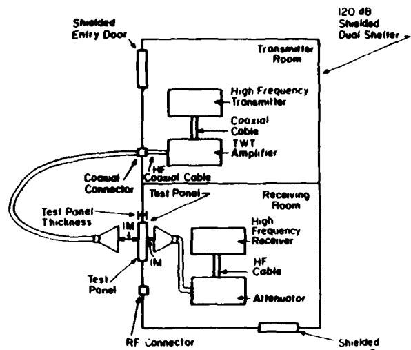
SIGNAL MEASUREMENT TEST SETUP FOR X-BAND HORN ANTENNA
