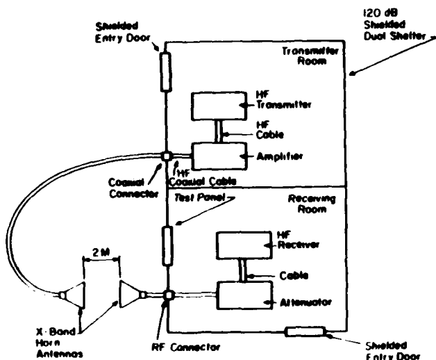
REFERENCE FOR MEASUREMENT TEST SETUP
