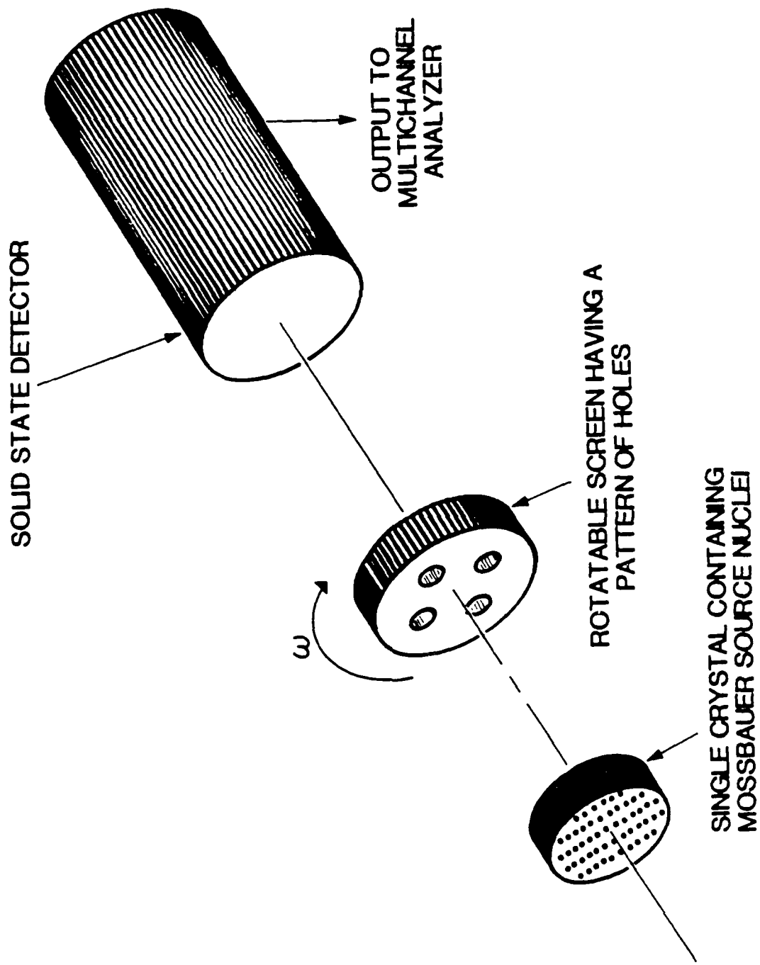
Fig. 8. Schematic representation of a possible experimental configuration to observe multibeam Borrmann modes.
