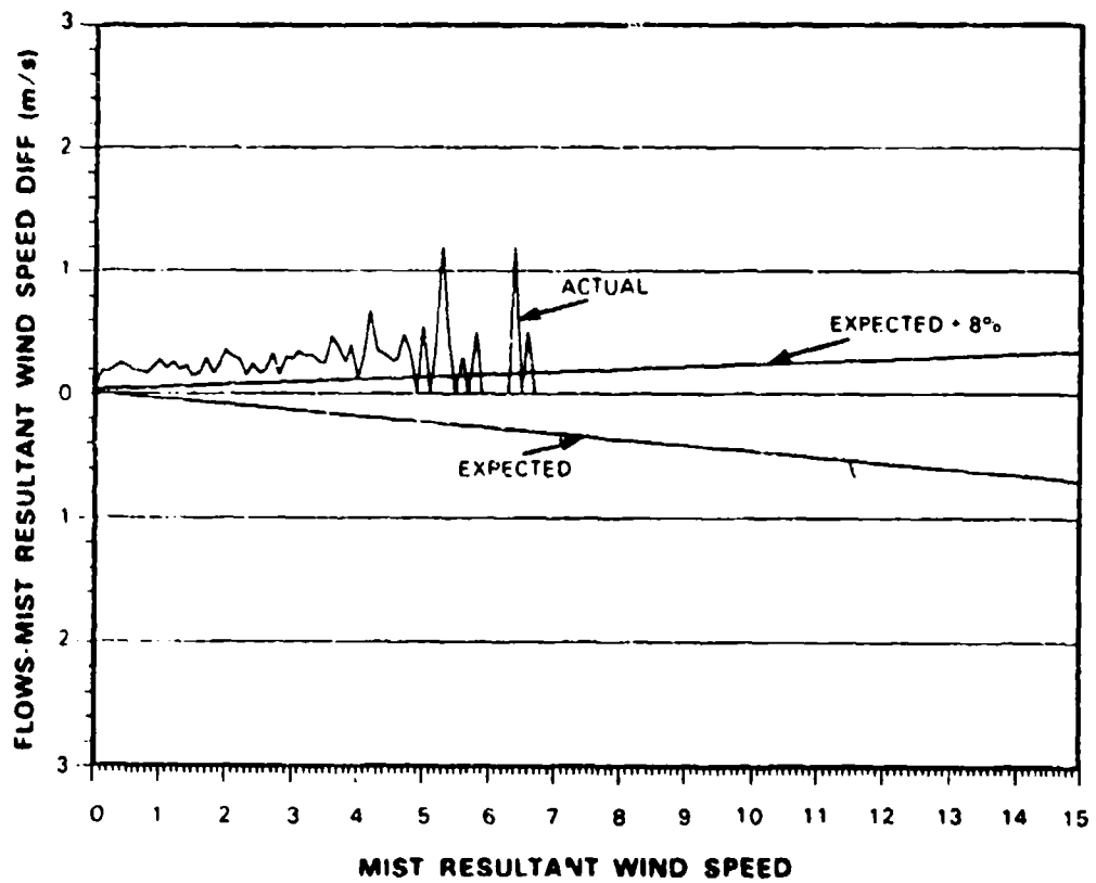
Figure 7. Network average wind speed difference vs. MIST average wind speed.
