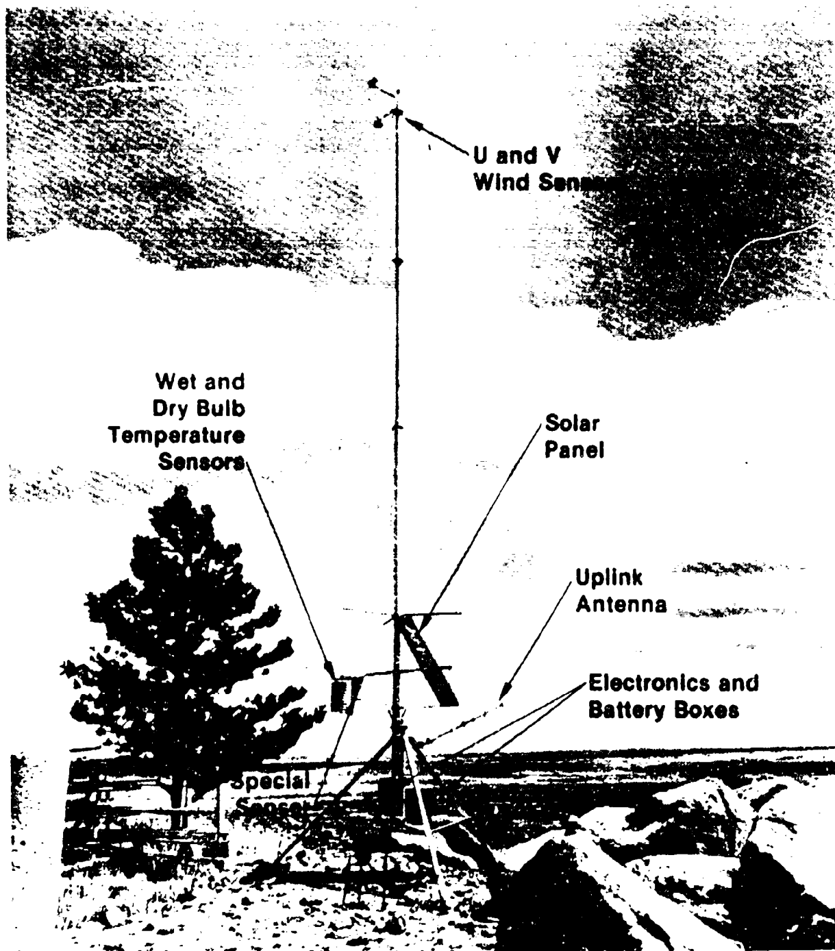
Figure 2. Photograph of a remote AM-II station. Taken from Brock, et al., (1986).
