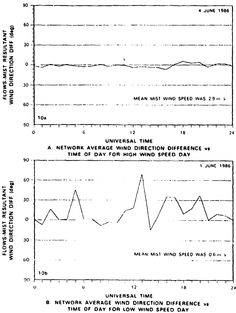
Figure 10. Difference between FLOWS and MIST network average wind direction vs. time of day (GMT) for a high wind speed day and a low wind speed day.
