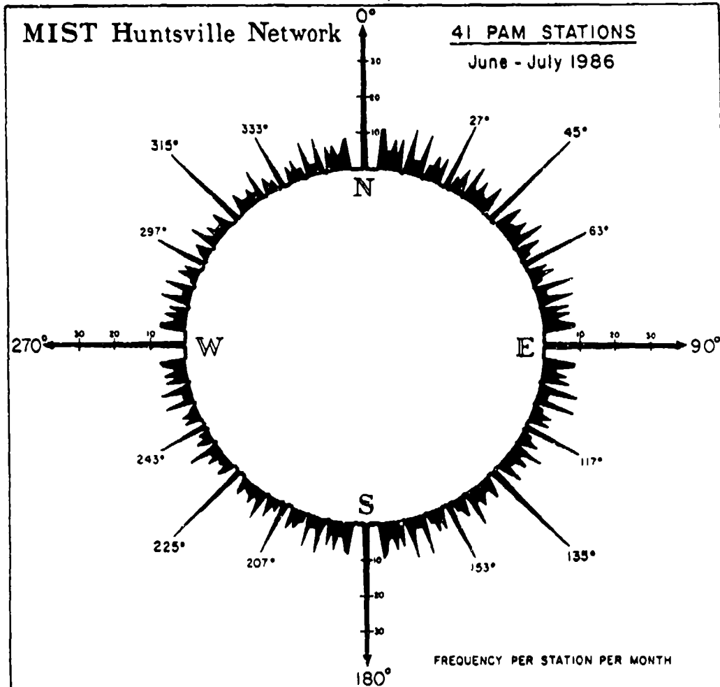
Figure 11. Azimuthal frequency of 0.0 - 0.5 m/s winds normalized per station per month for all 41 PAM stations during COHMEX (Fujita, 1987).
