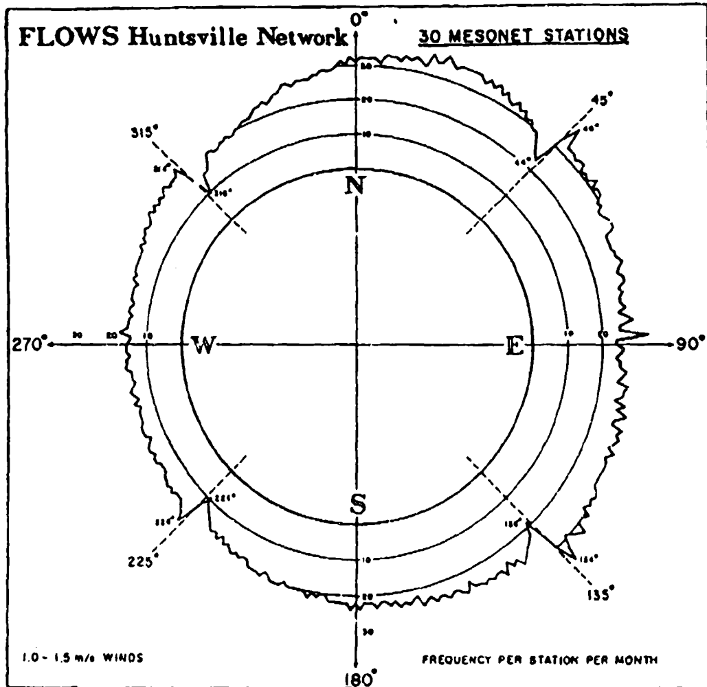
Figure 12. Azimuthal frequency of 1.0 - 1.5 m/s winds normalized per station per month for all 30 FLOWS stations during COHMEX (Fujita, 1987).
