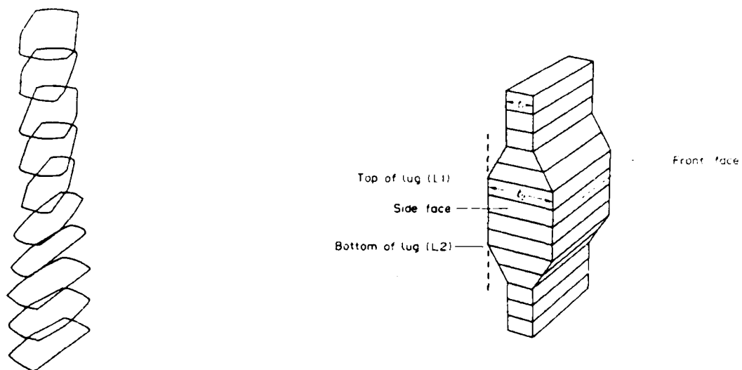
Figure 4-8: Three-dimensional reconstructions
