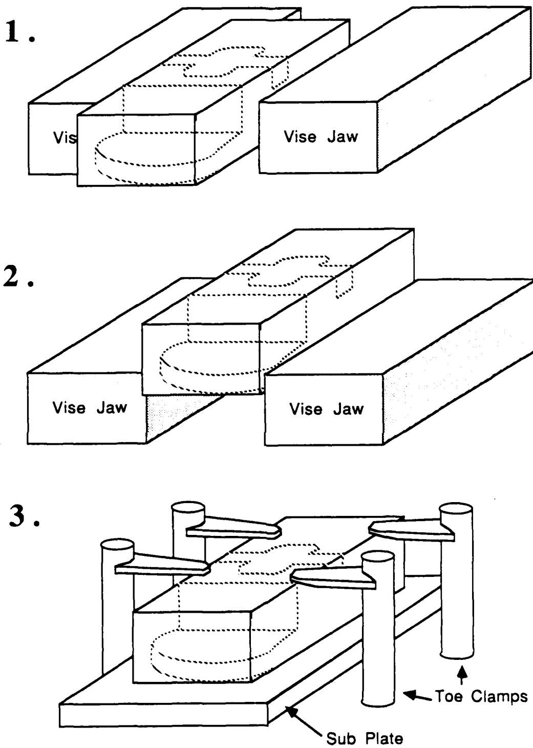
Figure 3-3: Three alternative ways of clamping the part to cut ears.
