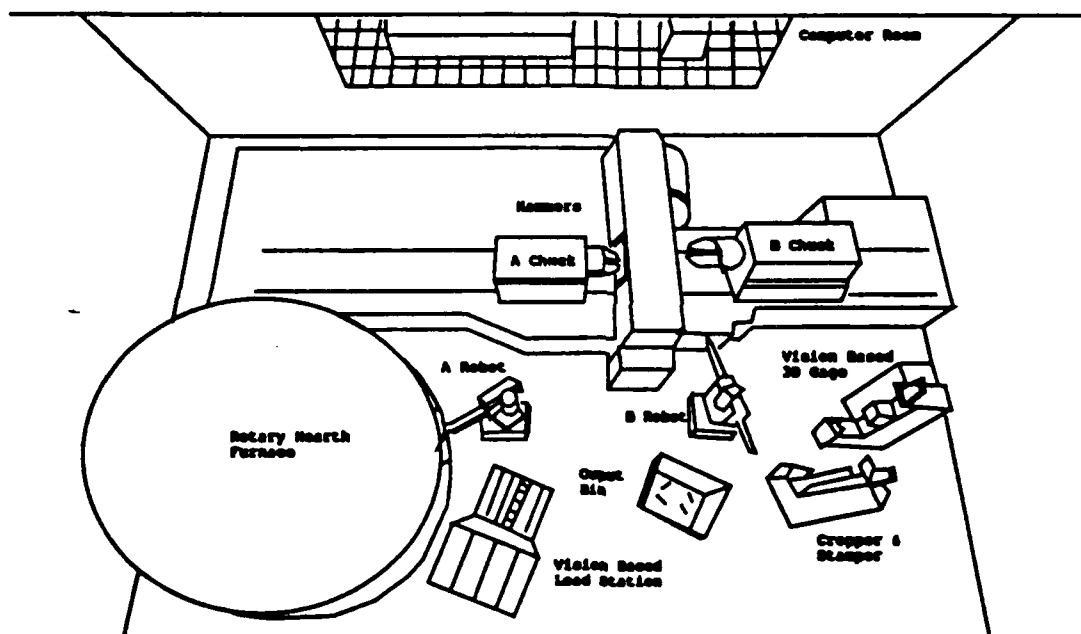
Figure 2-5: The GFM Manufacturing Cell for Making Pre-form Turbine Blades
