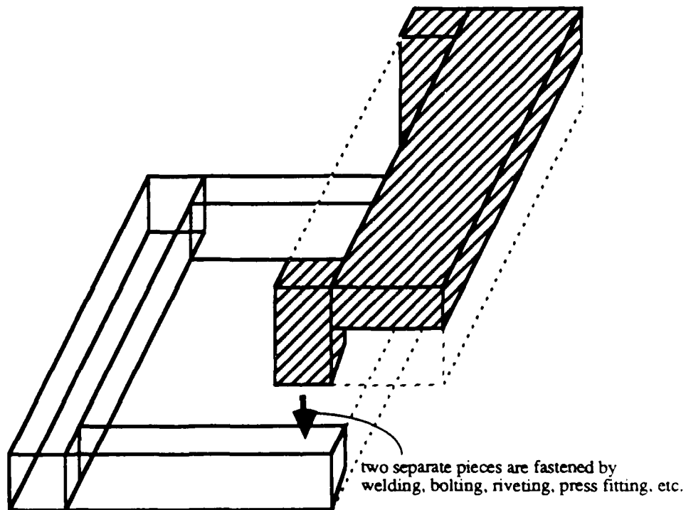
Figure 5-4: Redesign of part in Table 5-5, Guide A for clamping and machining
