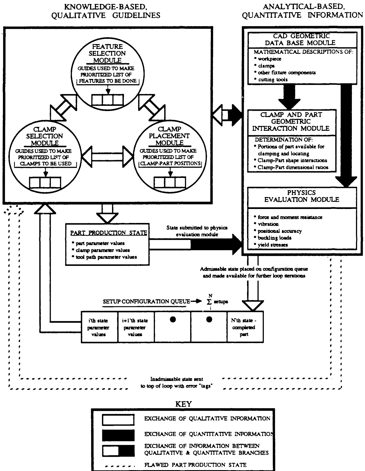
Figure 5-1: Control Structure for Part Process Planning System
