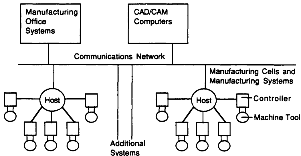
Figure 2-1: The Factory Hierarchy
