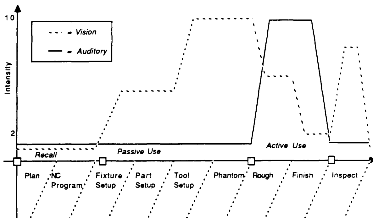
Figure 4-4: The use of visual and auditory monitoring during machining
