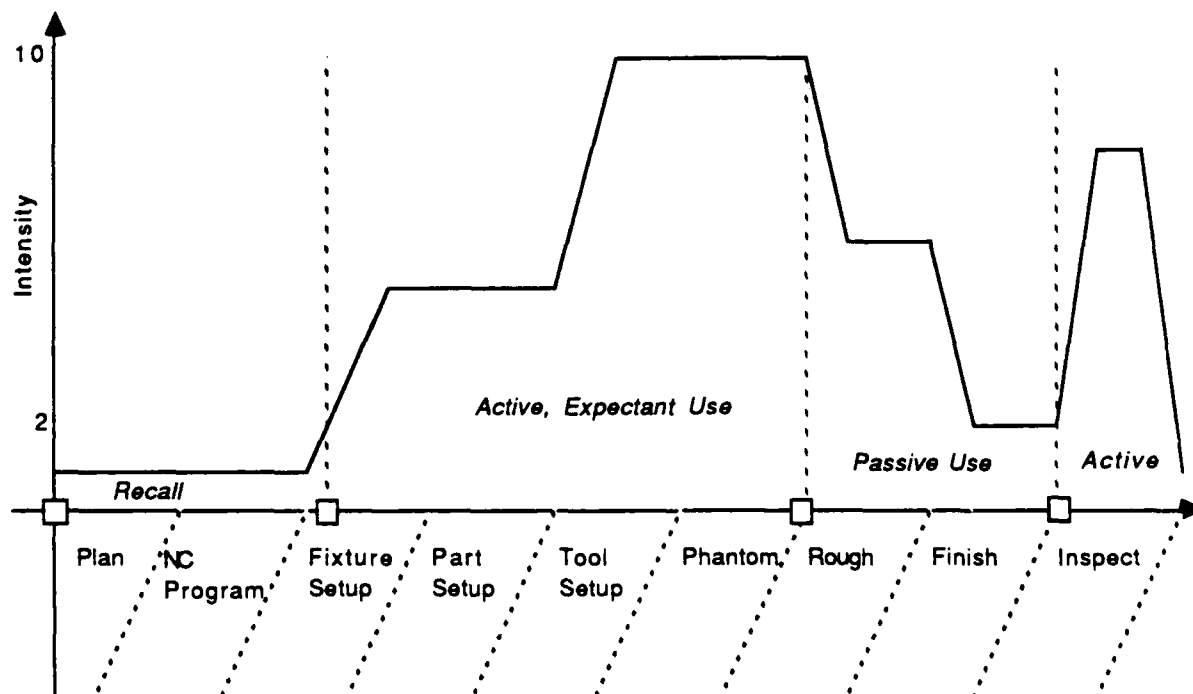
Figure 4-2: The use of visual monitoring during machining
