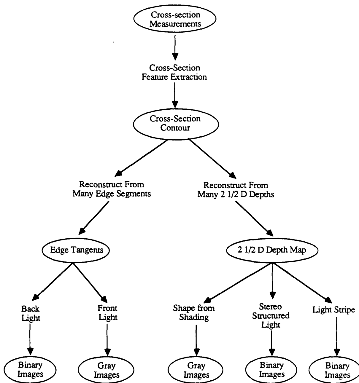
Figure 4-20: Vision plan tree for the preform gauging example
