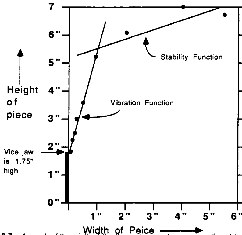
Figure 3-7: A graph of the width of the piece against maximum allowable height. Depth of Piece fixed at six inches.
