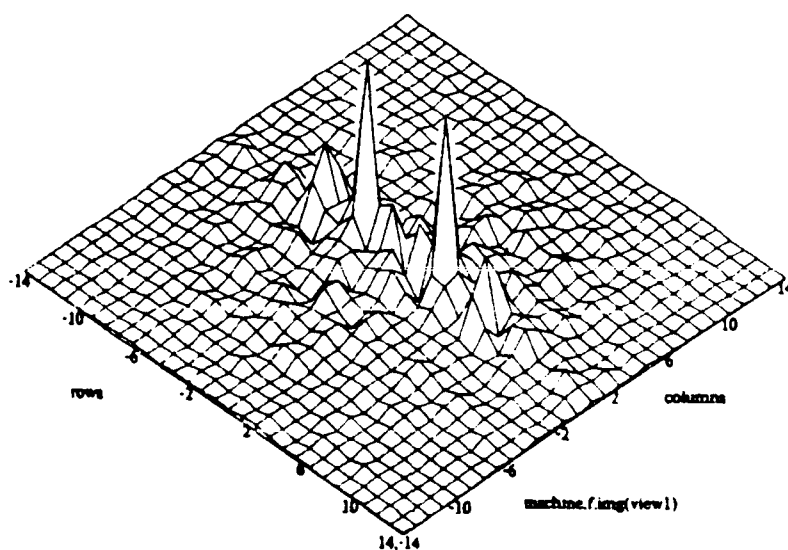
Figure 4-11: Images and 2-D FFT's of rolled, sawcut and machined surfaces
