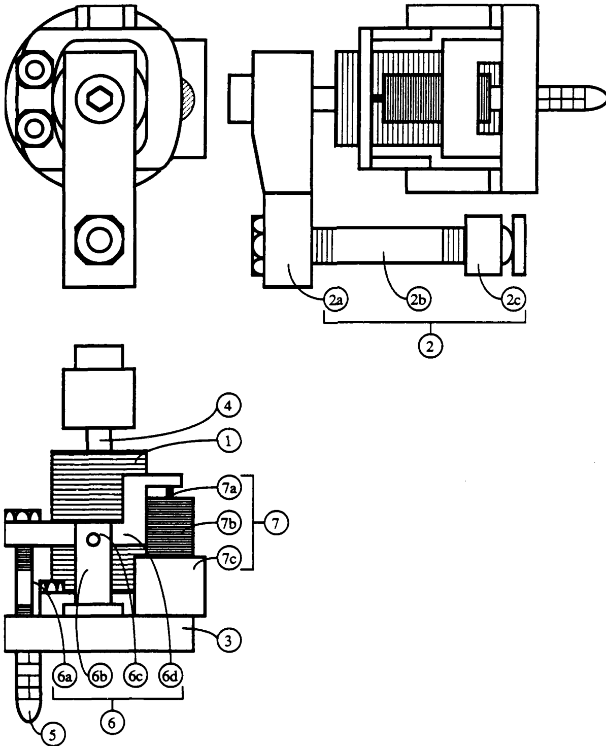
Figure 6-4: Hydraulic FLECS swing arm clamps
