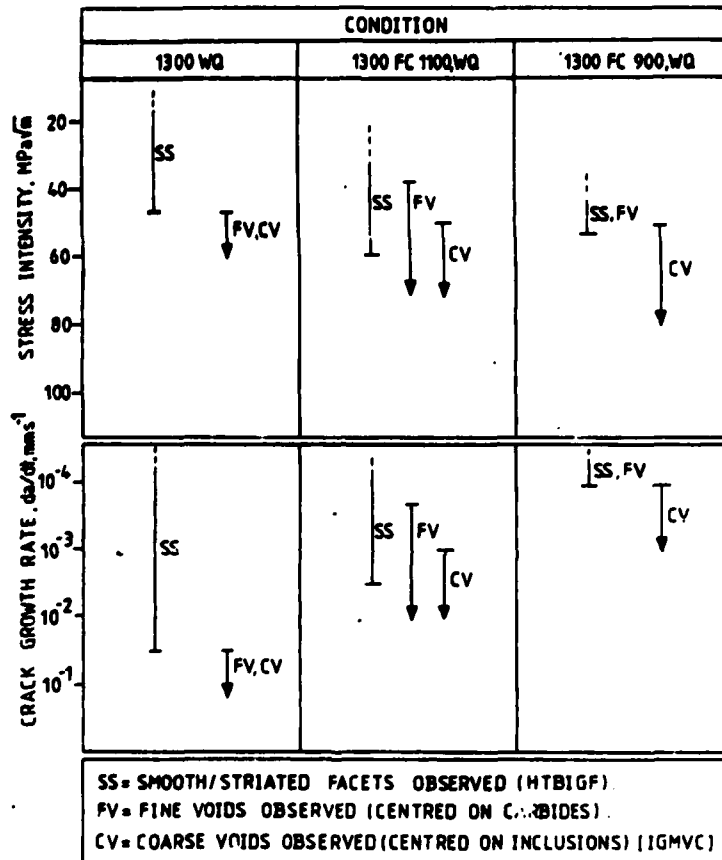
AERE R 12464 Fig. 12 Summary of observed dependence of fractographic features on (a) stress intensity and (b) crack growth rate
