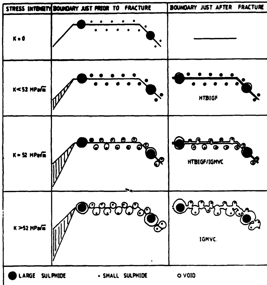
AERE R 12484 Fig. 15 Schematic representation of mechanisms of intergranular crack growth
