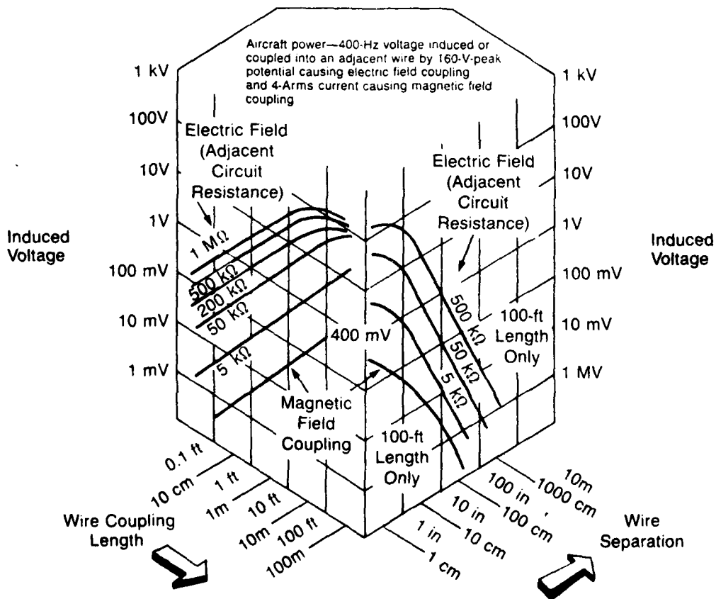
Figure 4.1-11 Coupling Versus Separation
