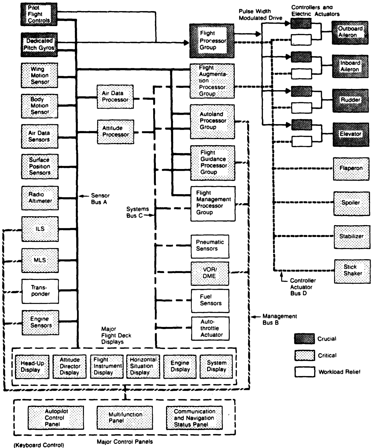
Figure 2.3-3 Projected Criticalities
