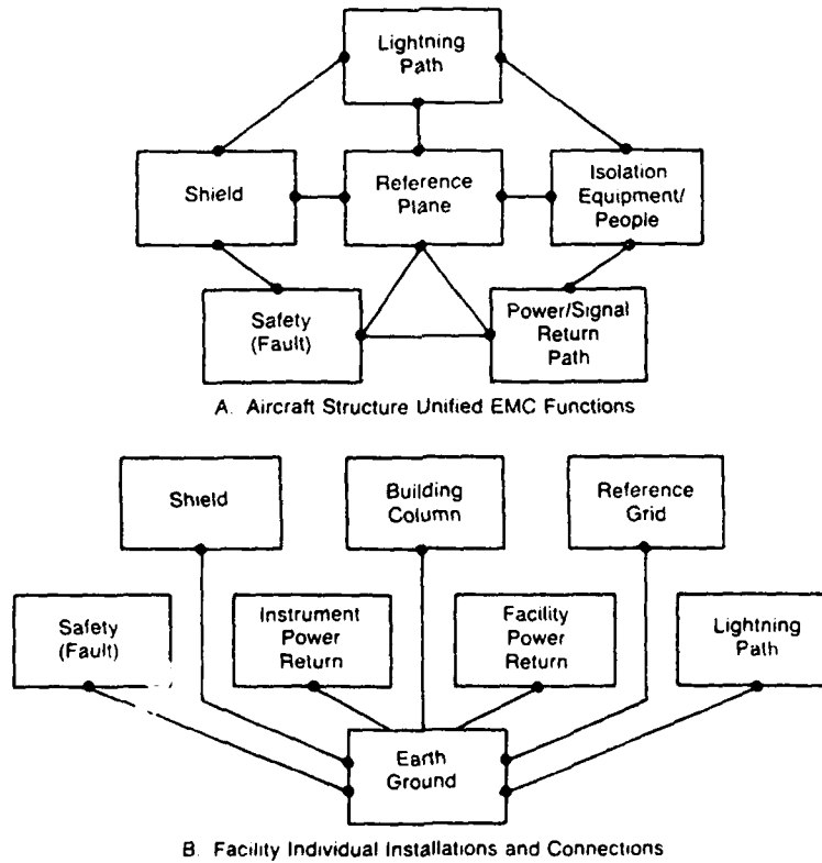
Figure 3.5-5 EMC Anatomy Block Diagram
