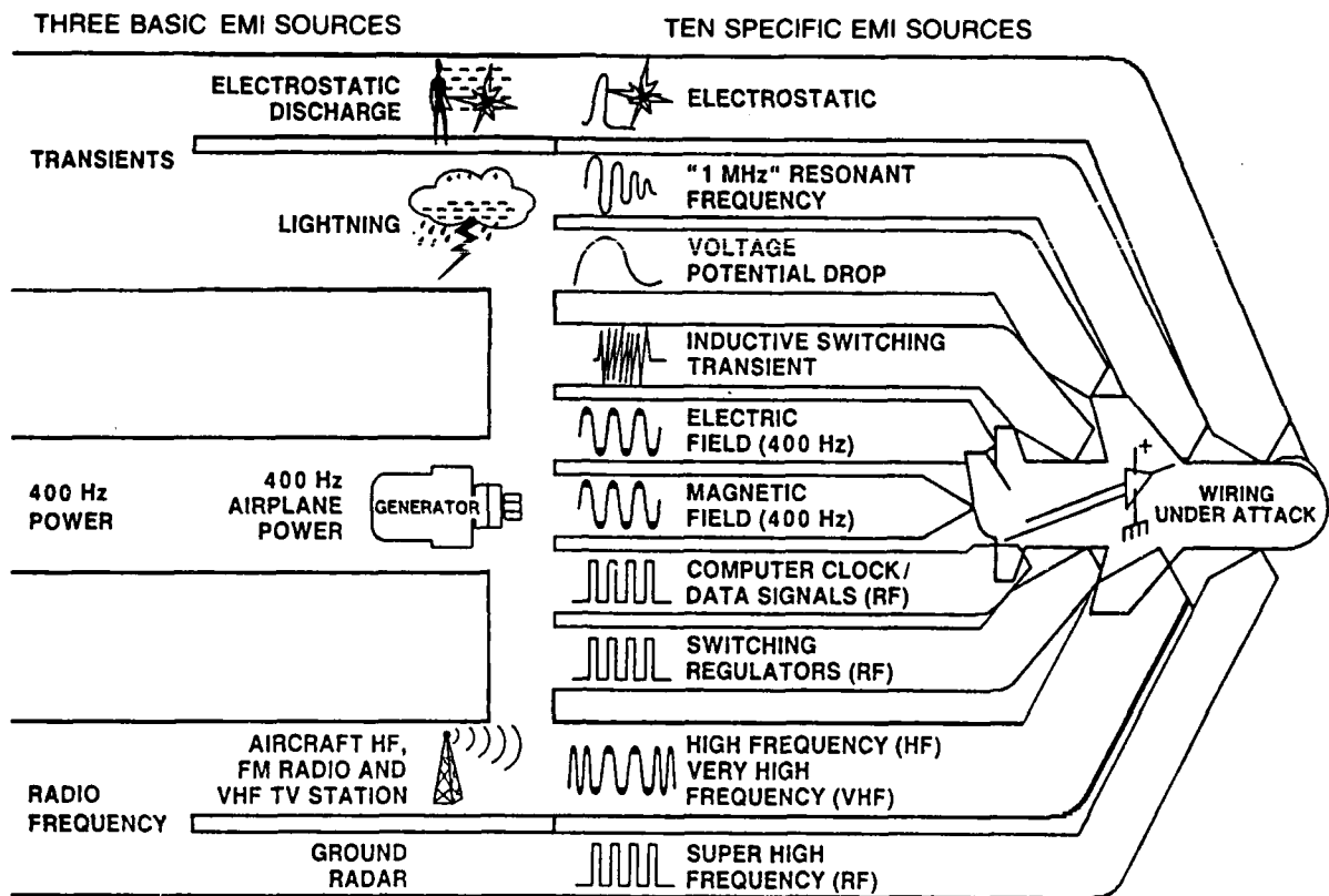
Figure 1.1-1 Representative EMI Sources
