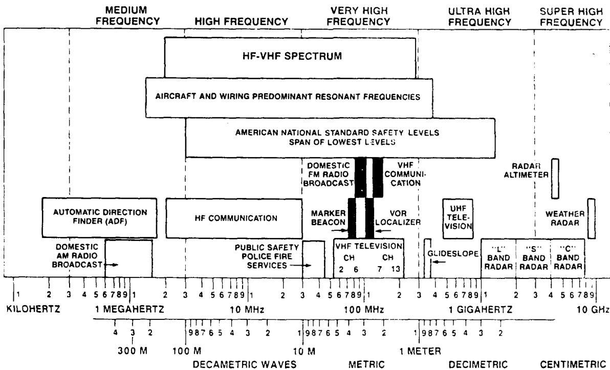
Figure 4.1-1 HF-VHF Range
