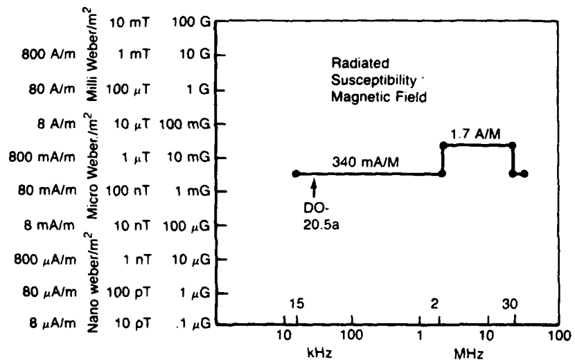
Figure B1. EMI Test Limits (Continued)
