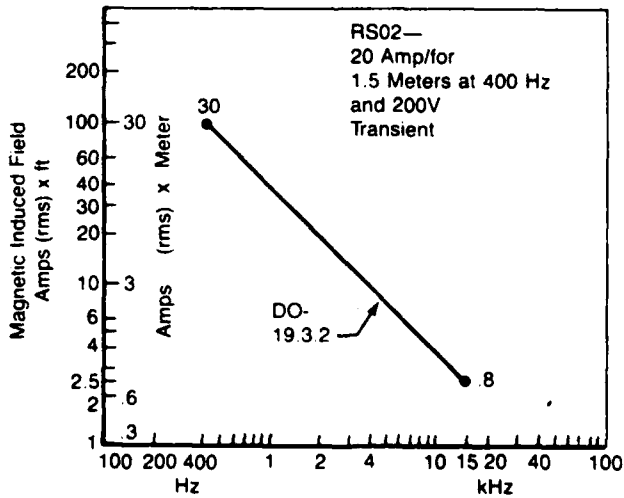
Figure B1. EMI Test Limits (Continued)
