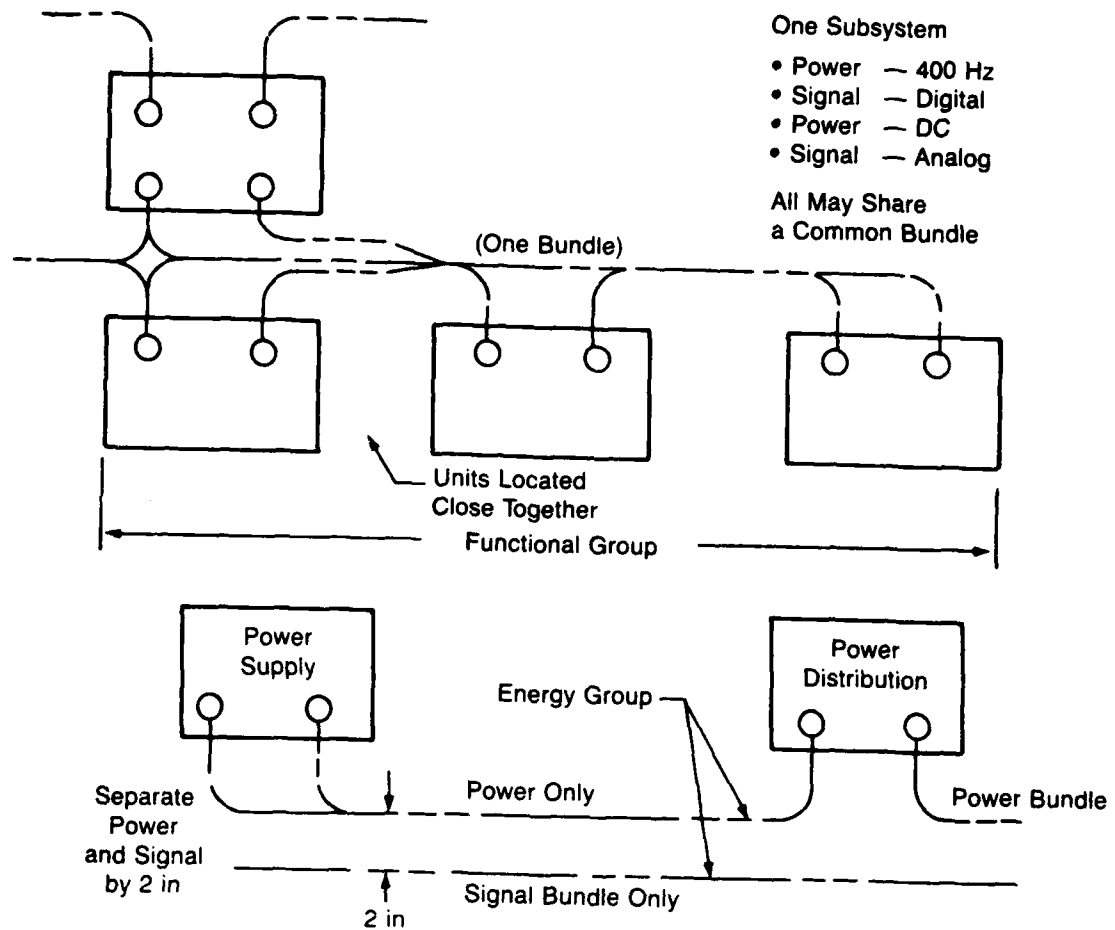
Figure 3.4-2 Wiring Categories
