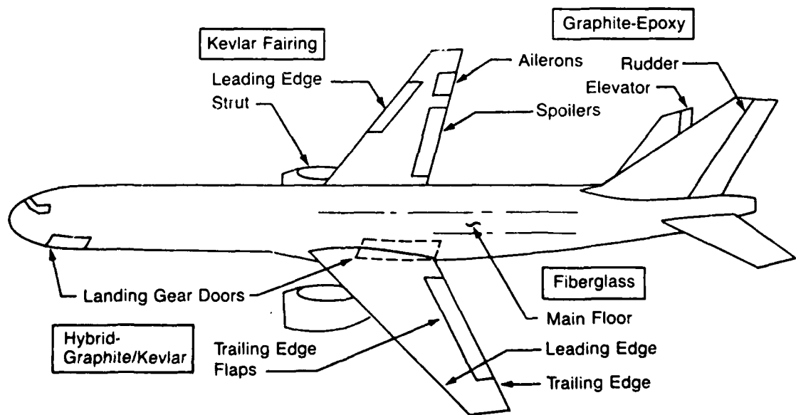
Figure 2.1-8 Nonmetallic Interfaces
