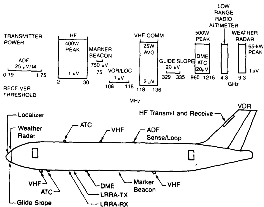
Figure 2.1-12 Transmitters-Receivers
