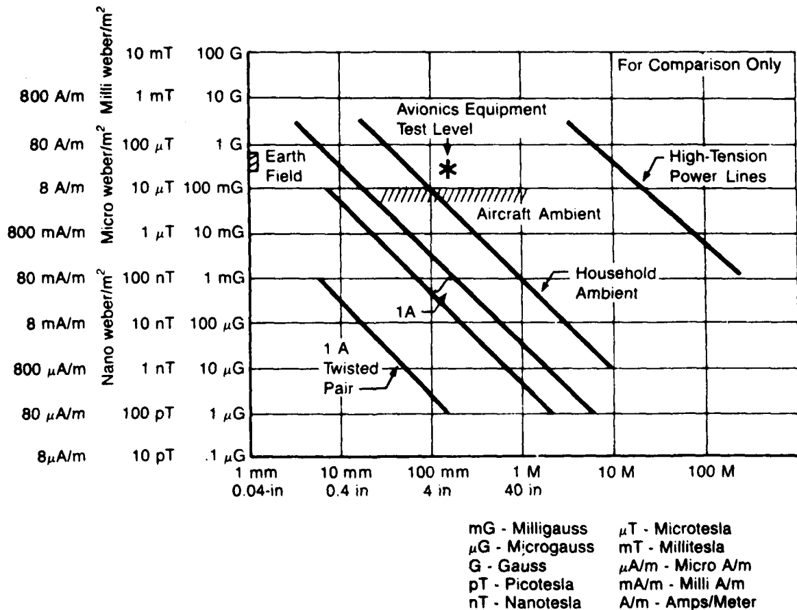
Figure 4.1-12 Magnetic Fields
