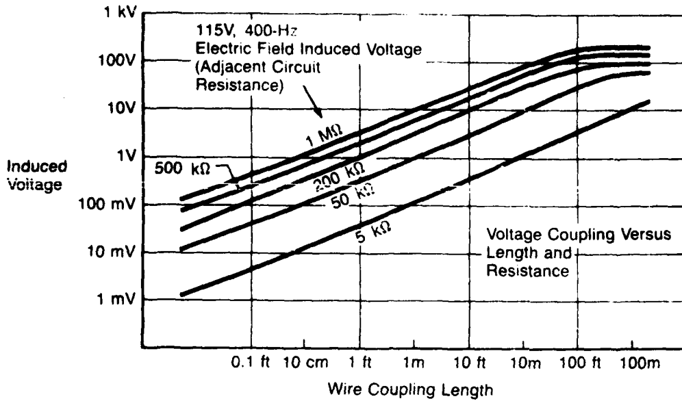
Figure 4.1-10 "E" Field Coupling
