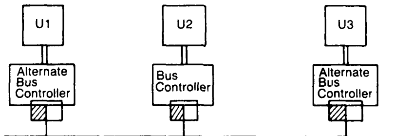
(b) MIL-STD-1553B
