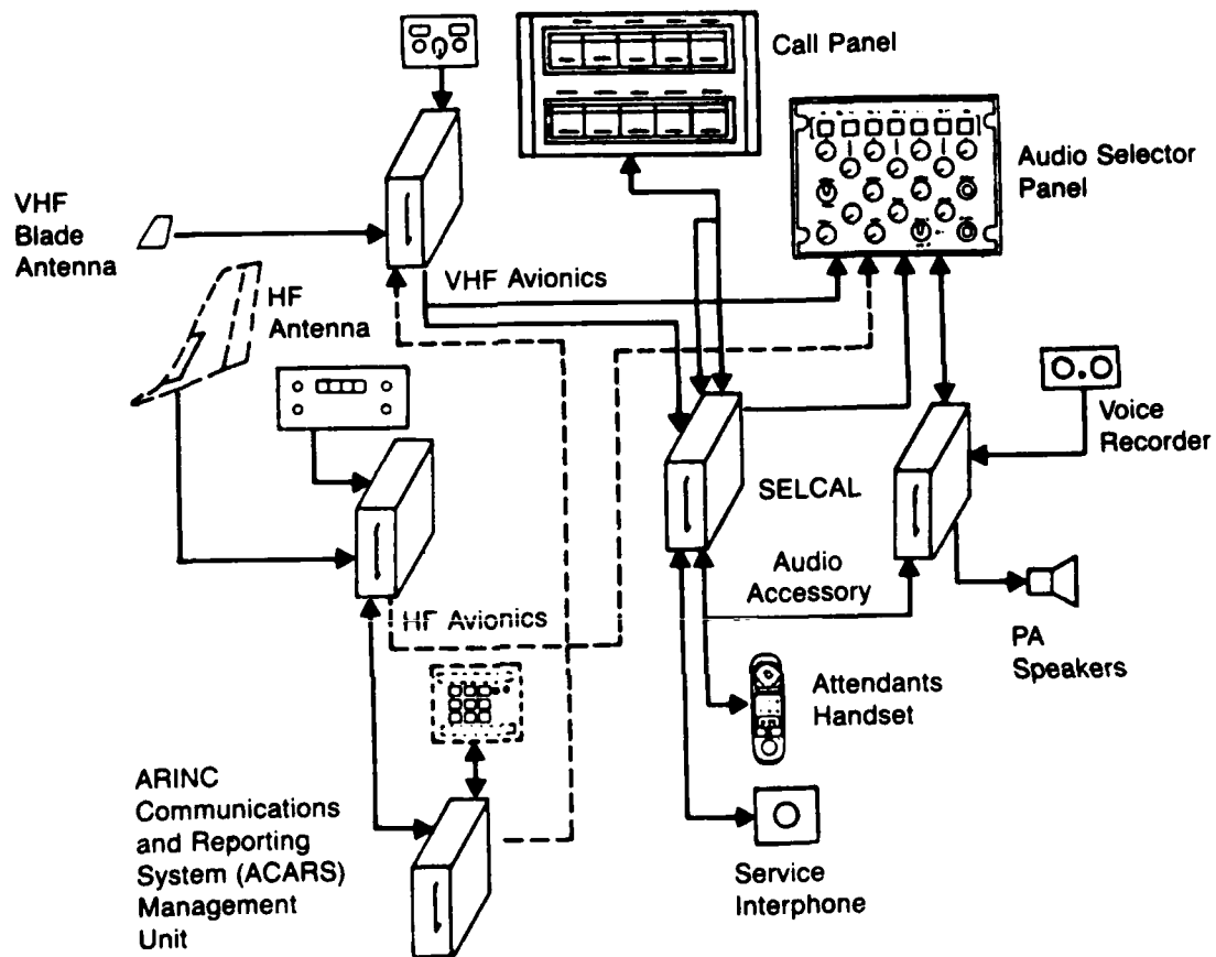
Figure 2.1-16 Communication
