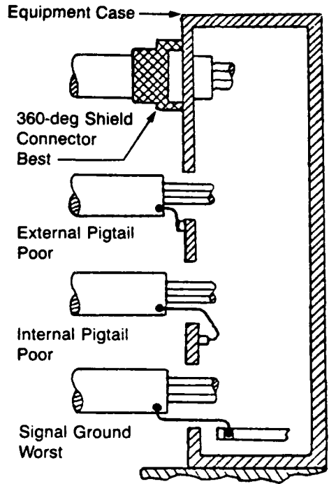
Figure 3.4-6 Shield Ties
