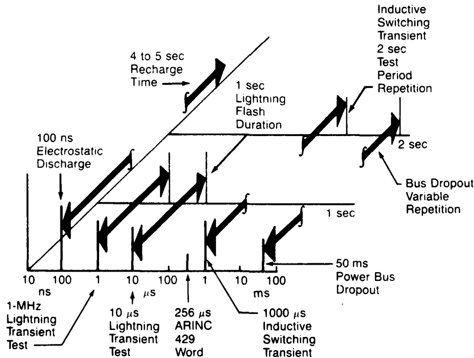
Figure 3.2-1. Transient Events
