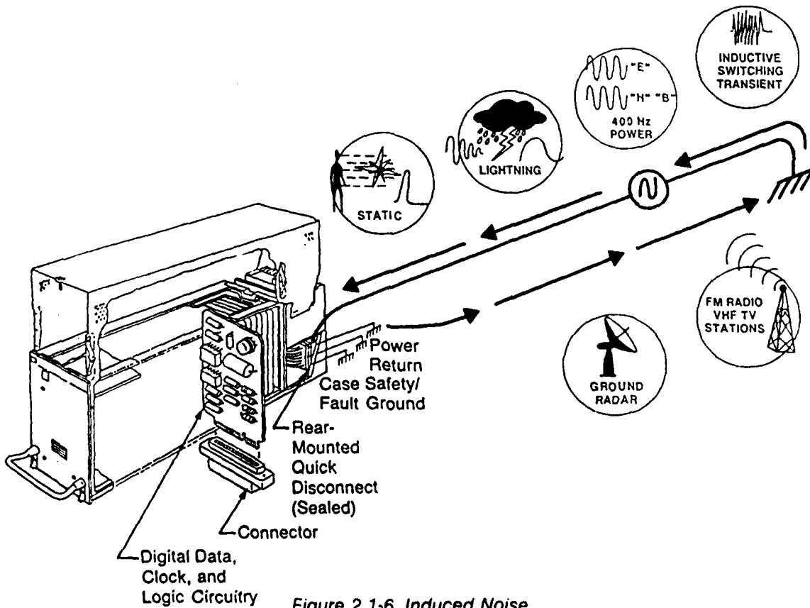
Figure 2.1-6 Induced Noise
