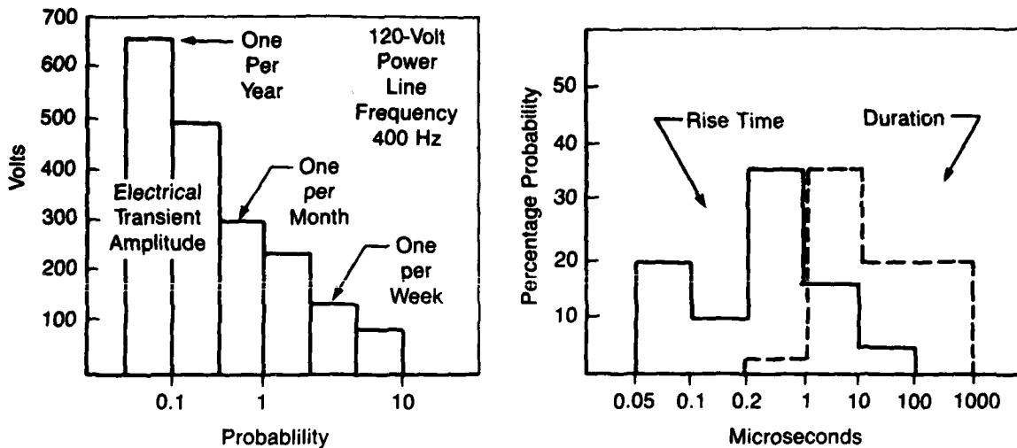
Figure 4.1-14 Electrical Transients
