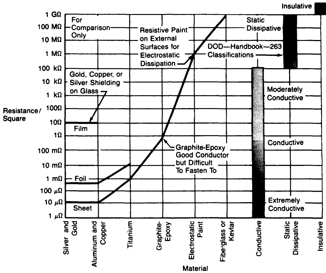
Figure 3.5-12 Material/Resistance Overview
