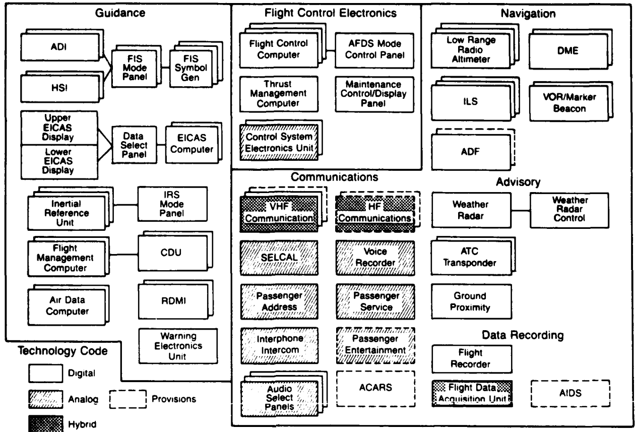
Figure 2.1-18 Flight Management Systems
