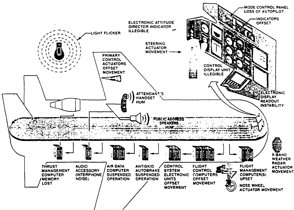
Figure 1.1-4 Electromagnetic Interference Effects
