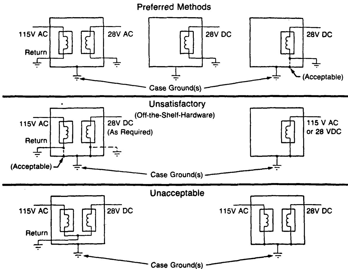
Figure 3.5-11 Power Returns
