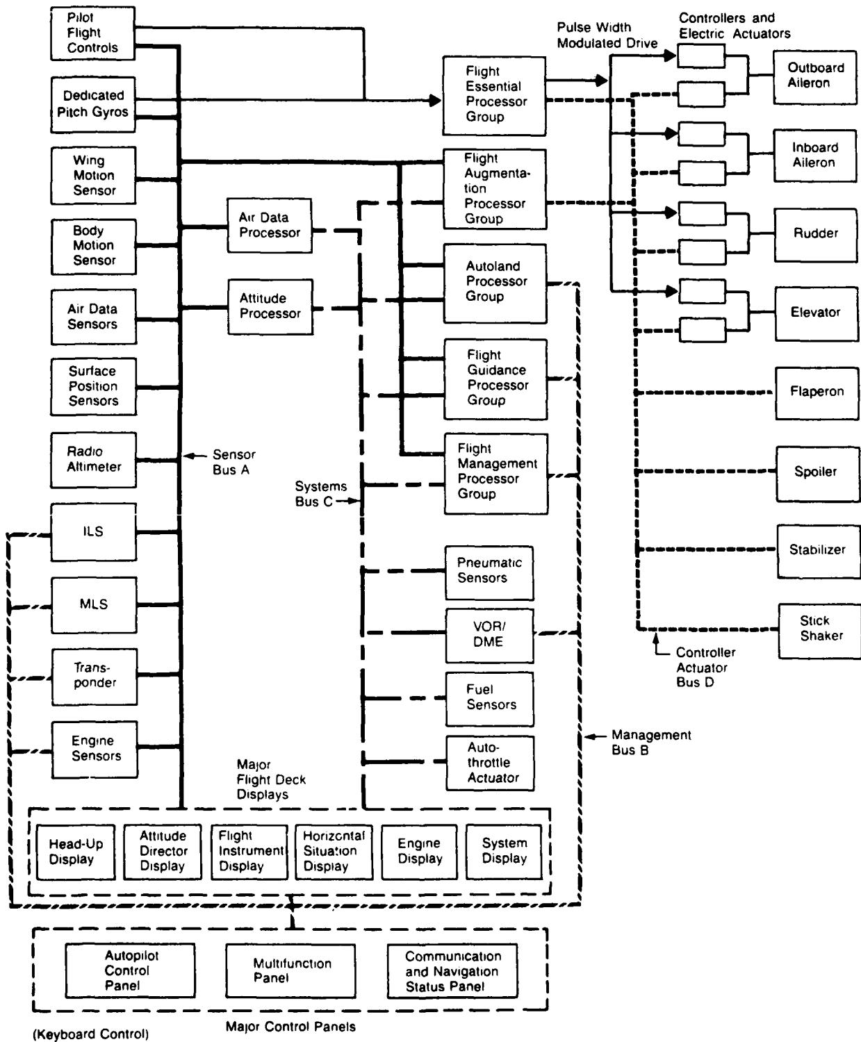
Figure 2.2-4 Hypothetical Architecture
