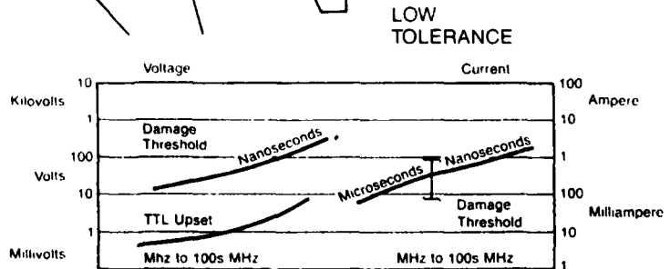
Figure 4.3-3 Trade—Digital Circuits
