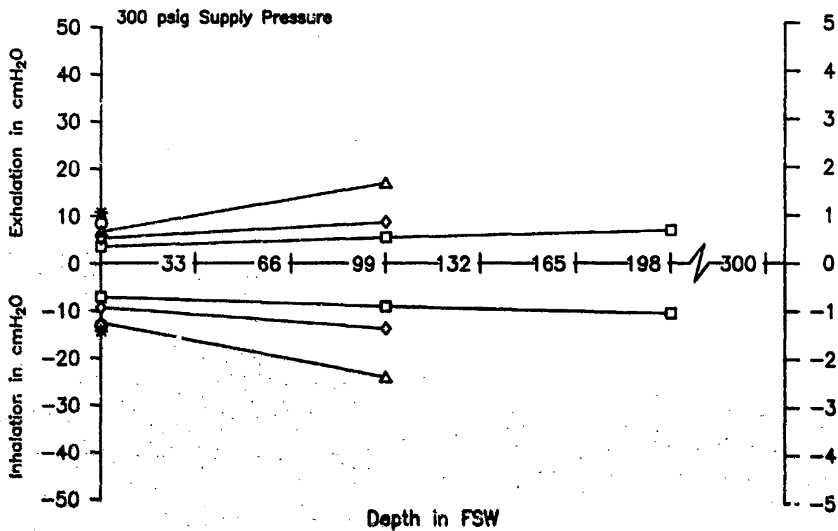
Breathing Resistance vs. Depth
