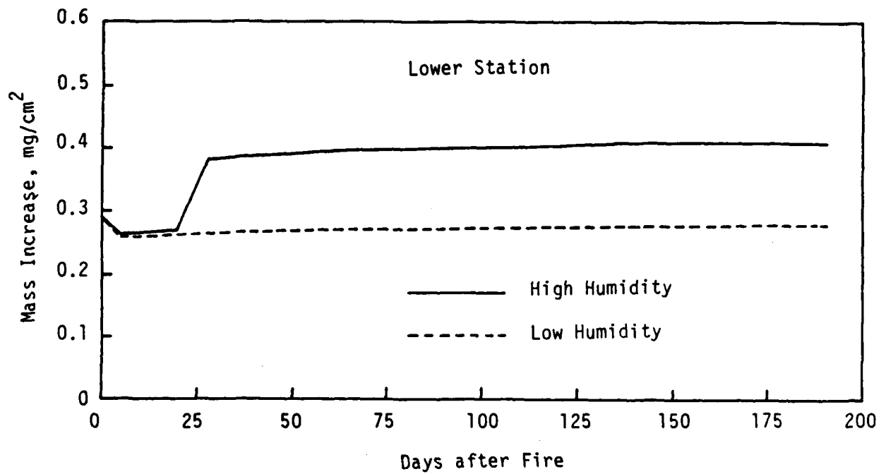
Figure 23. Mass Increases due to Corrosion for Brass for Test W-13A (Flaming).
