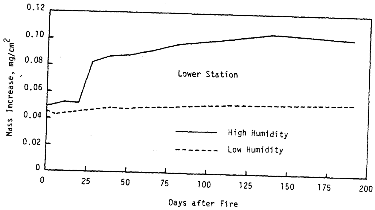
Figure 25. Mass Increases due to Corrosion for Monel 400 for Test W-13 (nonflaming).
