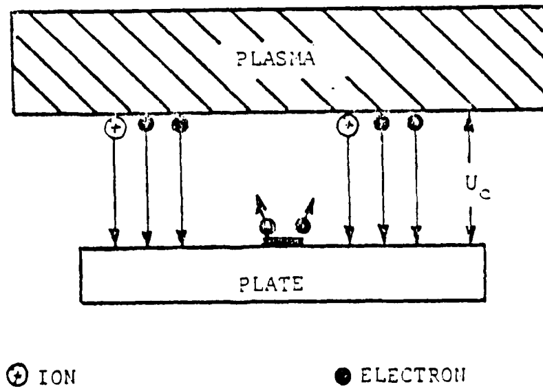
Figure 2.4 Isolated Plate with Cathode Spot.
