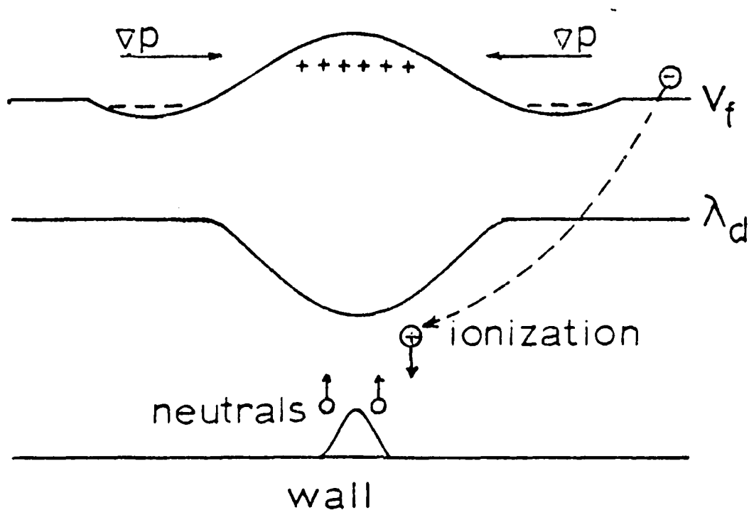
Figure 2.2 Schwirzke-Taylor Unipolar Arc Model.
