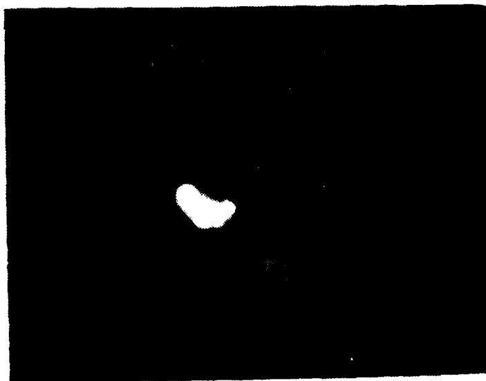
Figure 4.7 Same as above with a 90% Attenuating Filter
