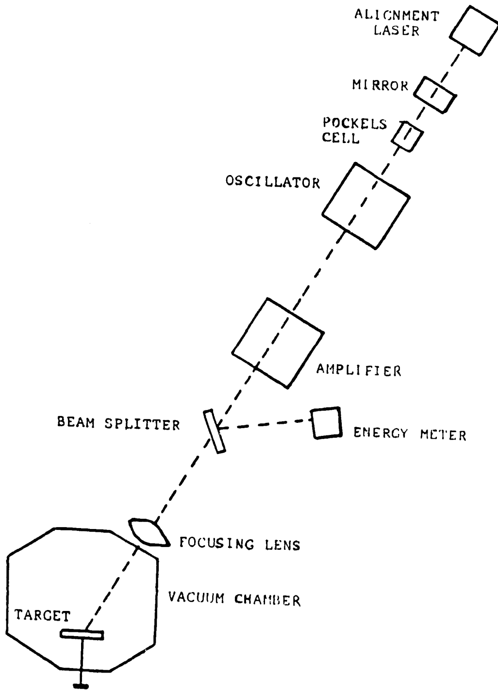
Figure 3.1 Experimental Setup.
