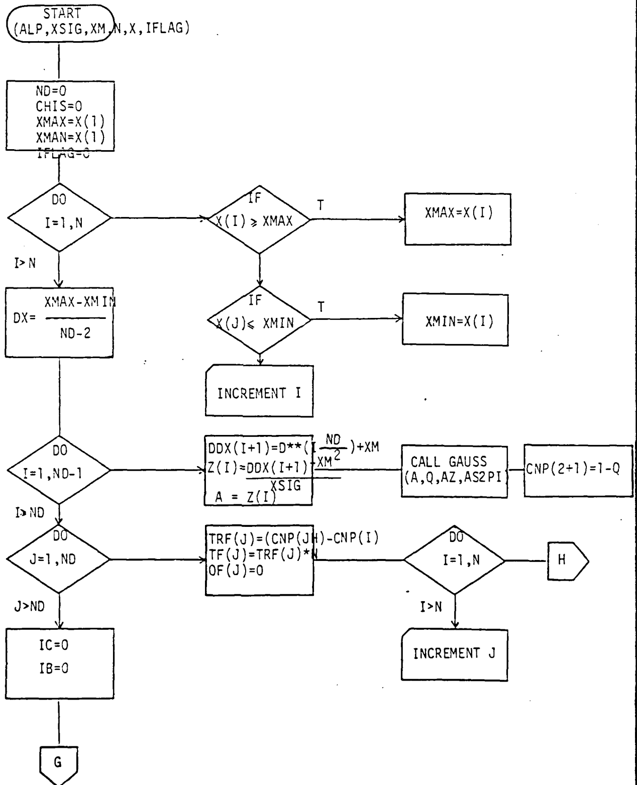
FIGURE 3 Subroutine TNORM
