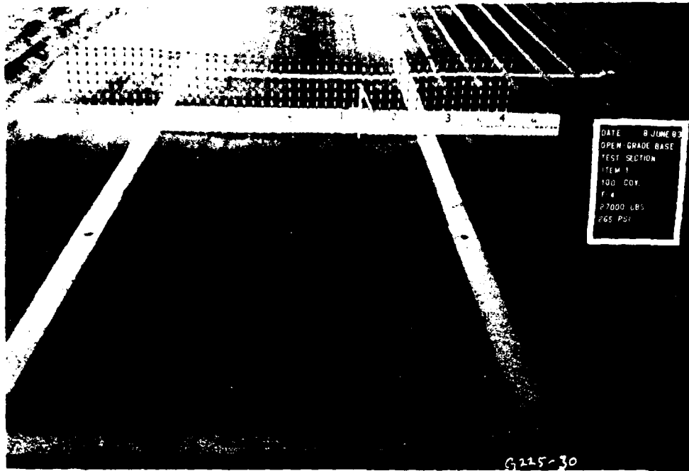
Photo 17. Rutting of Item 1 after 100 coverages
