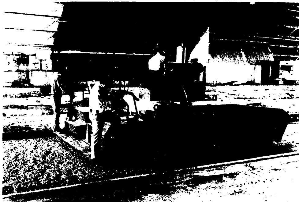
Photo 11. Placing open-graded base
