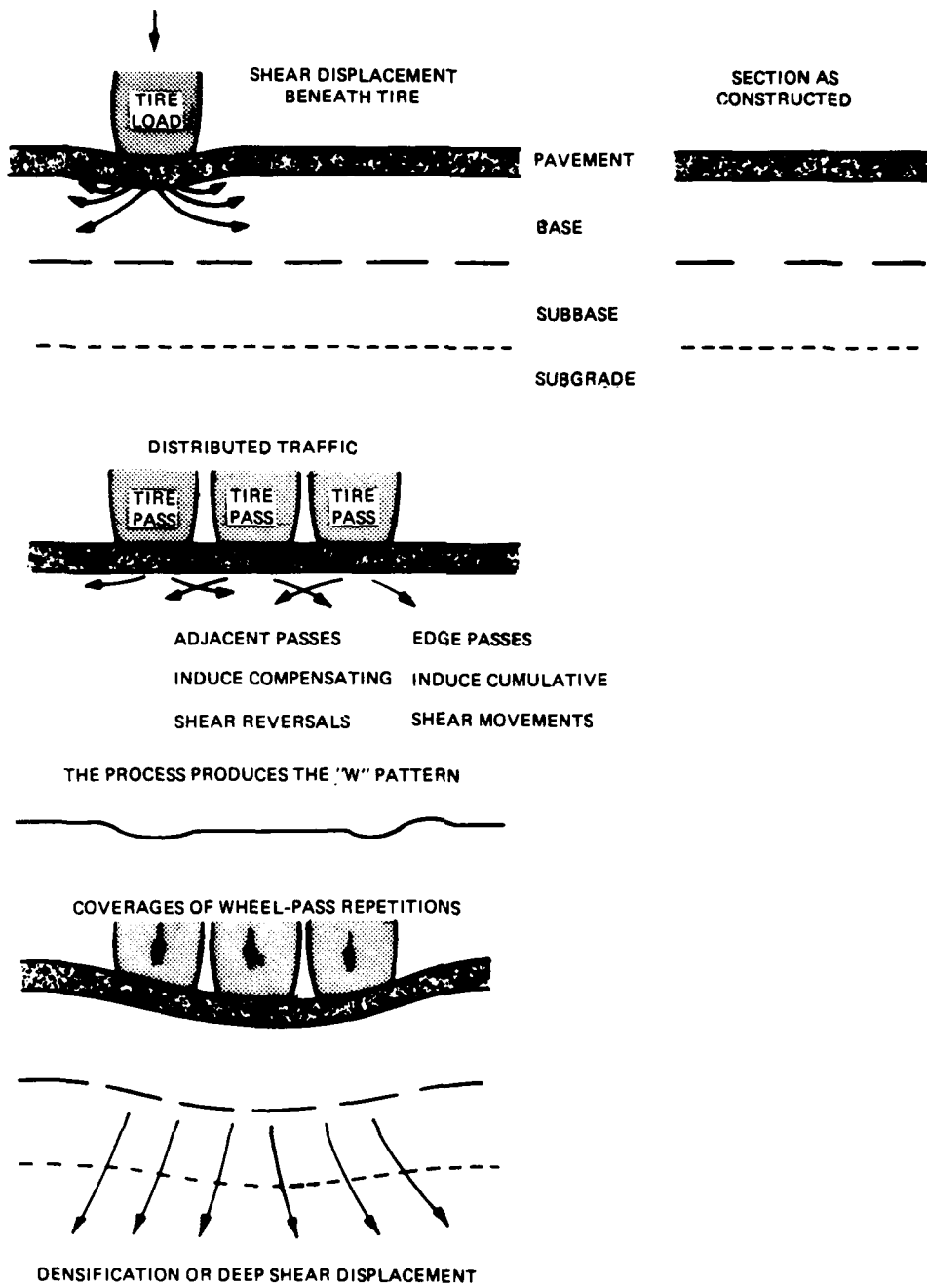
Figure 14. Schematic representation of traffic effects
