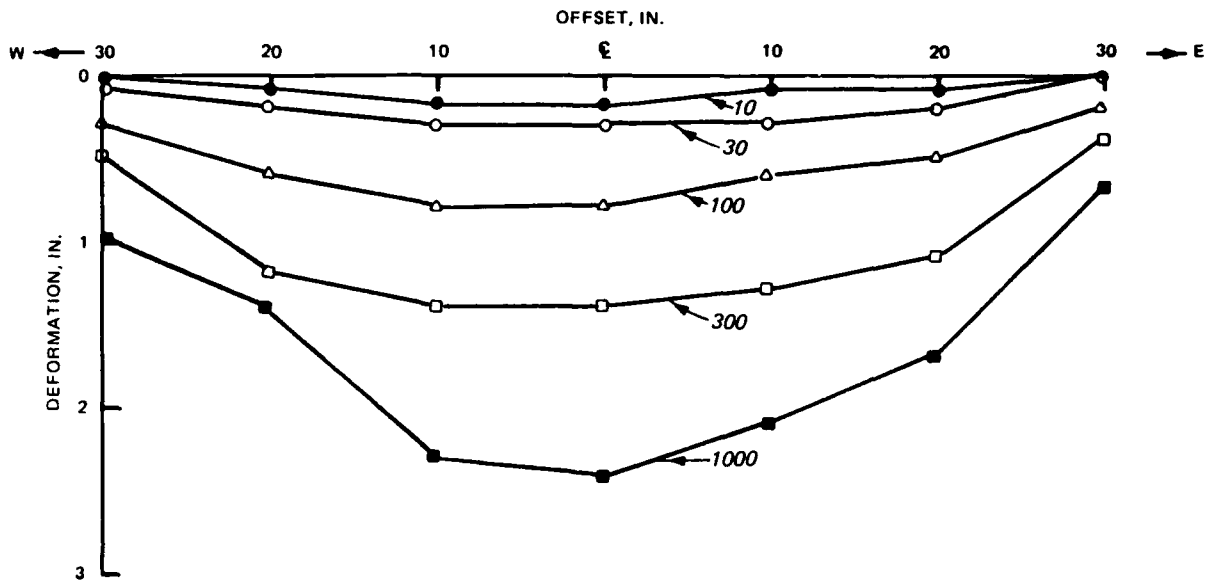
Figure 7. Cross section of Item 2 at sta 0+30
