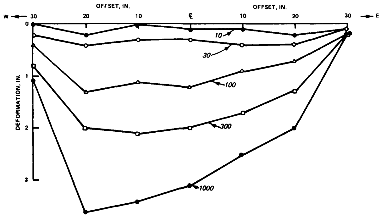
Figure 5. Cross section of Item 1 at sta 0+15
