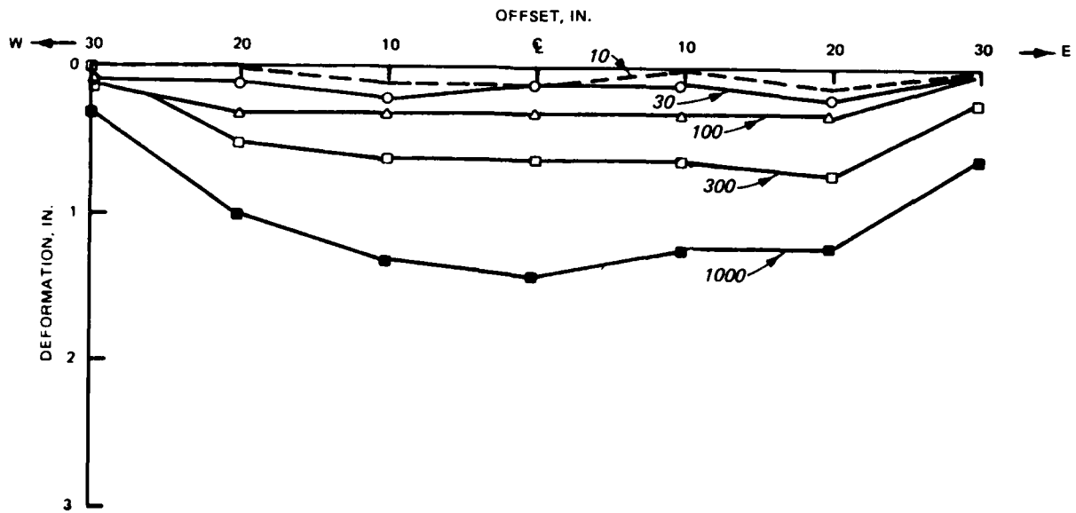
Figure 8. Cross section of Item 3 at sta 0+47.5
