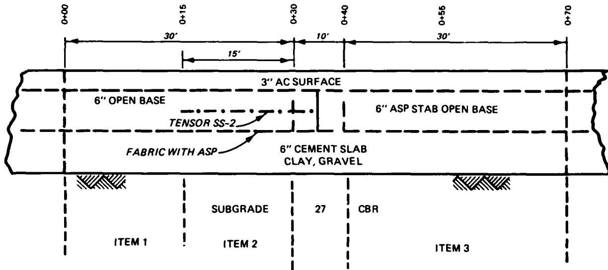
Figure 2. Typical longitudinal section
