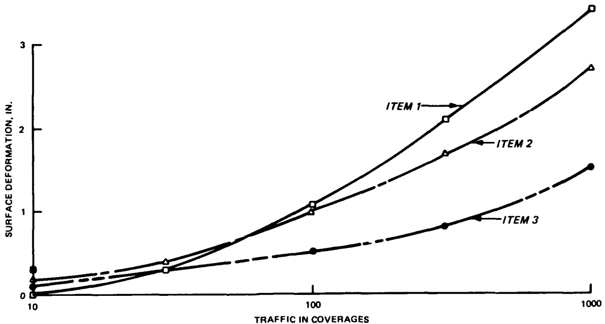
Figure 13. Maximum surface deformation as a function of traffic
