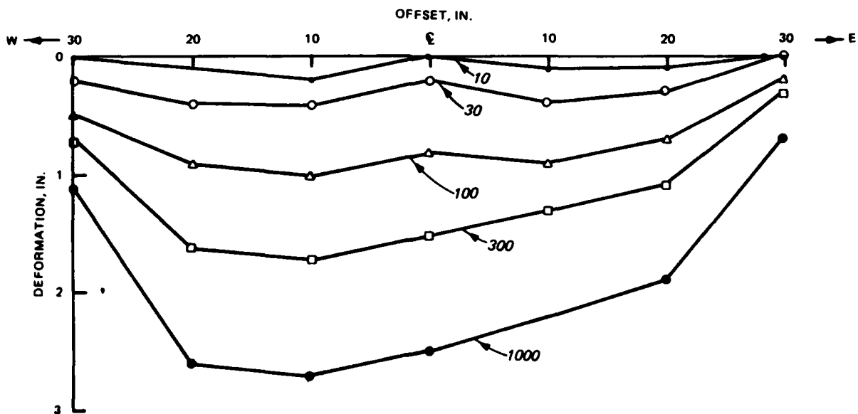
Figure 6. Cross section of Item 2 at sta 0+25
