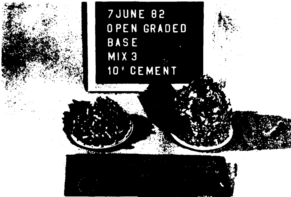
Photo 3. Broken sample of cement-stabilized aggregate (Mix 3)
