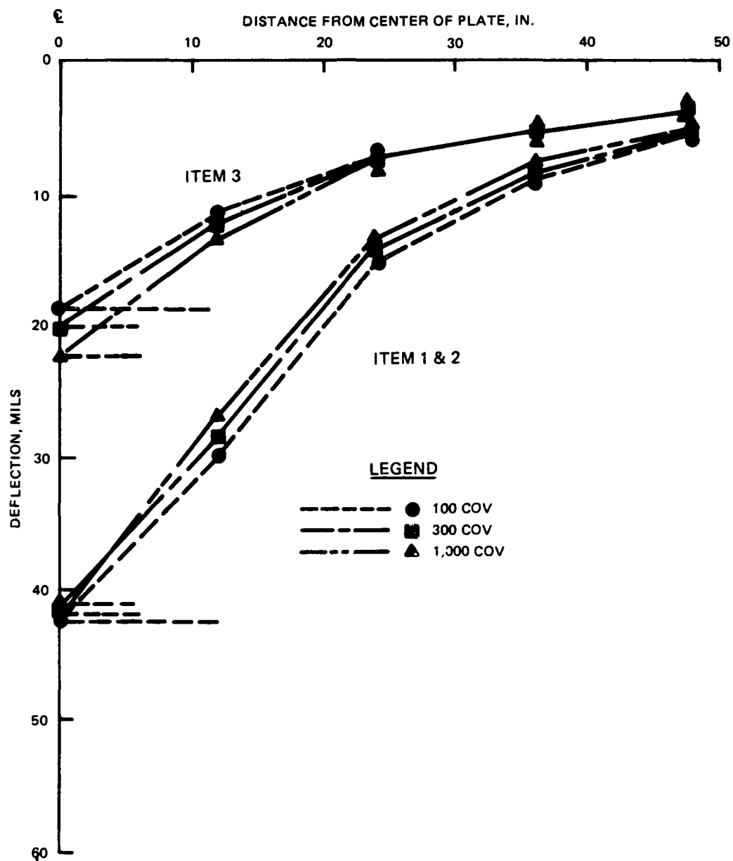
Figure 12. Deflected surface for FWD tests at coverage levels of 100, 300, and 1,000
