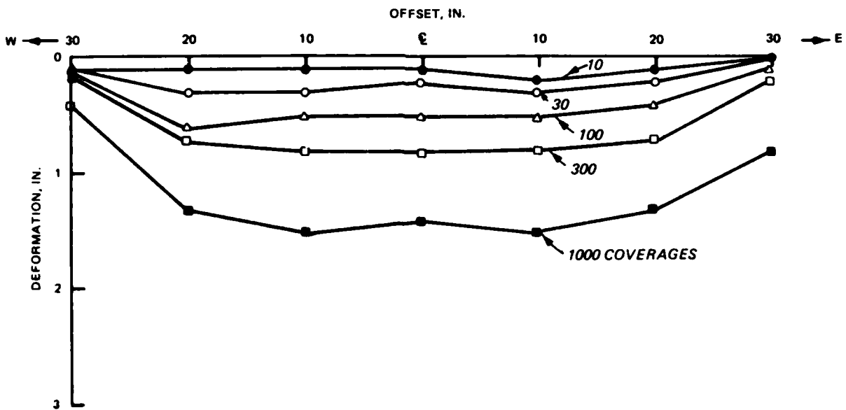
Figure 10. Cross section of Item 3 at sta 0+62.5
