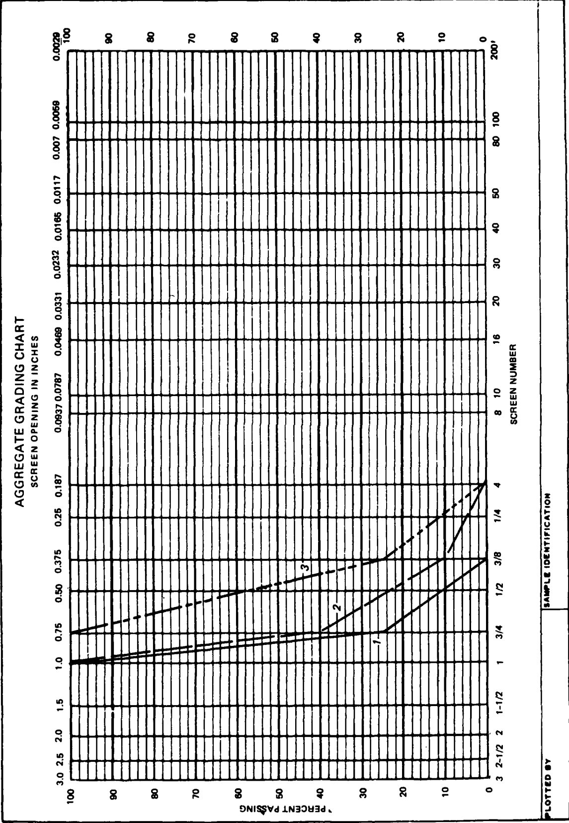
Figure 3. Gradations for open stabilized base
