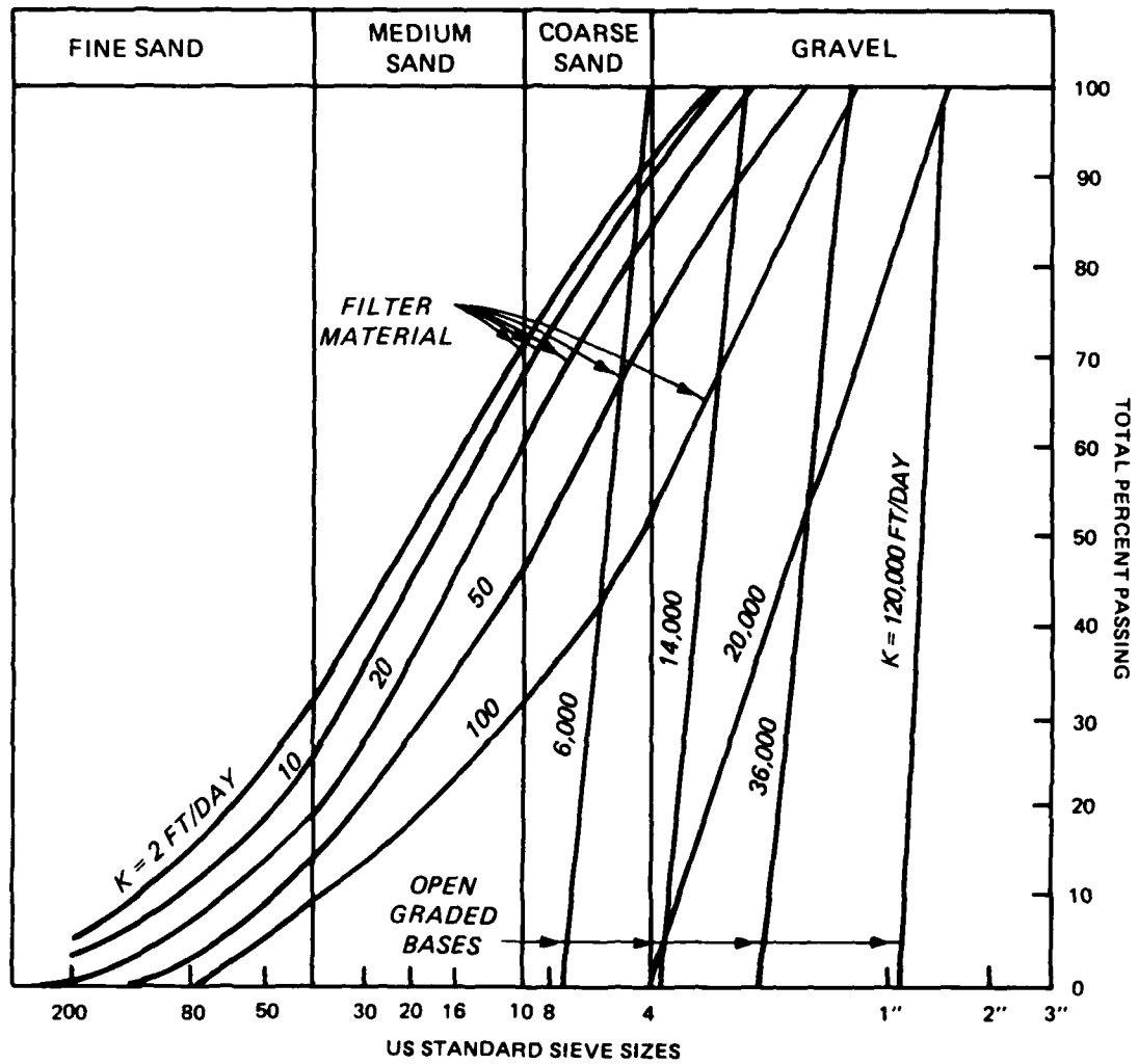
Figure A1. Typical gradations and permeabilities of open-graded bases and filter materials (From FHWA 1980a)
