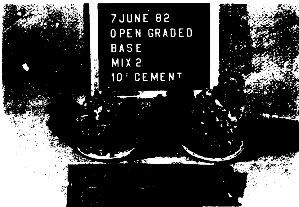
Photo 2. Broken sample of cement-stabilized aggregate (Mix 2)
