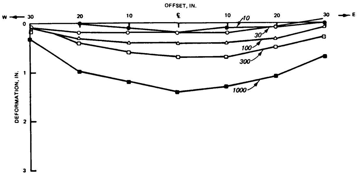
Figure 9. Cross section of Item 3 at sta 0+55
