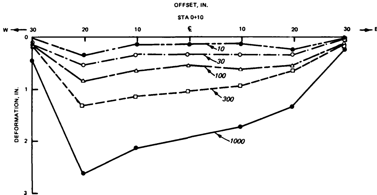
Figure 4. Cross section of Item 1 at sta 0+10
