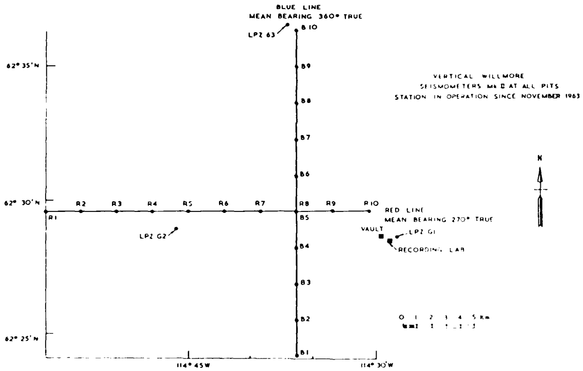
Figure 10c. Layout of the AWRE array YKA.
