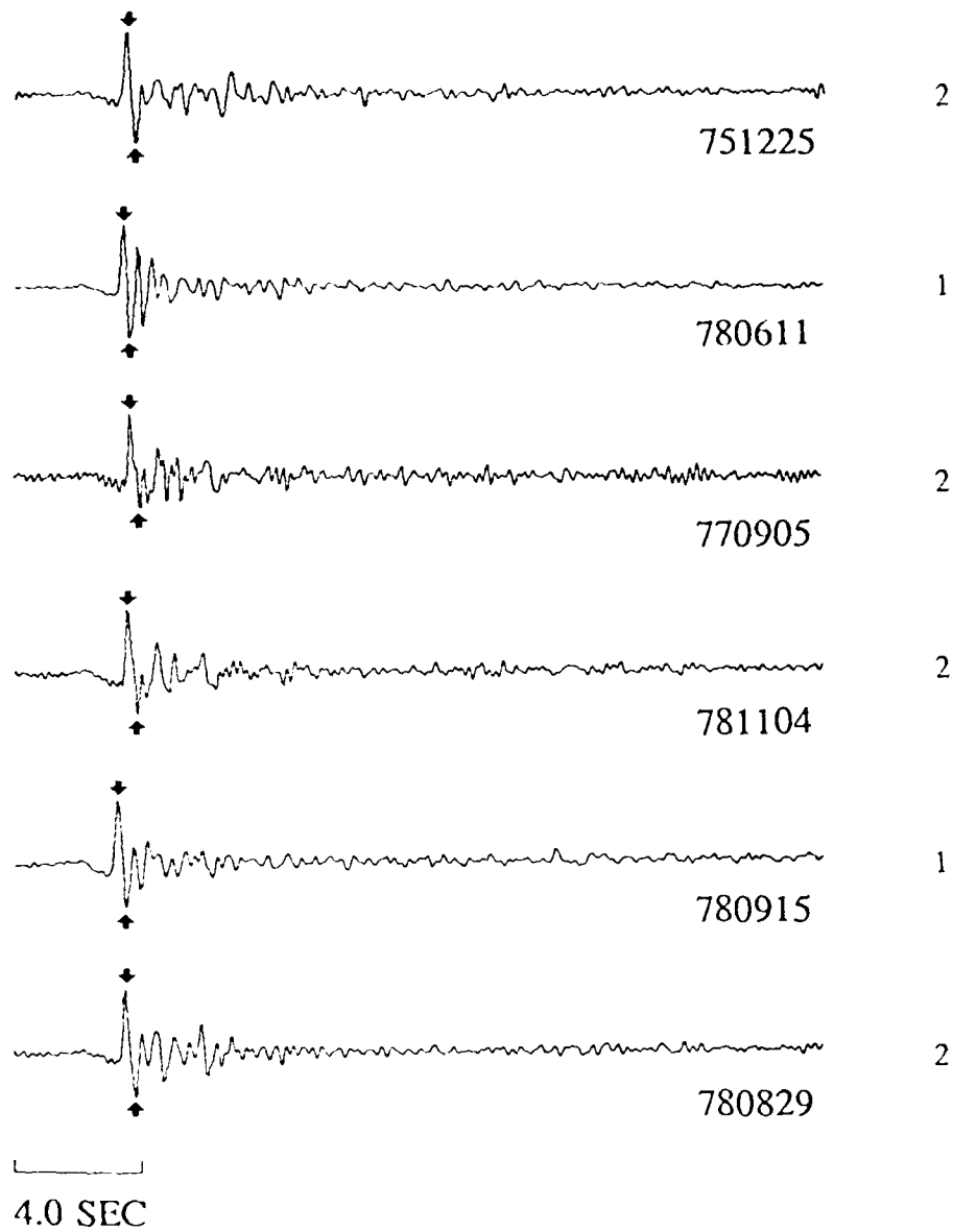
Figure 23. Source time function estimates obtained for E-EKTS explosions at WRA. A VSB wavelet has been removed in these deconvolutions. The waveform classification assigned by Marshall et al (1984) is noted to the right of each trace.
