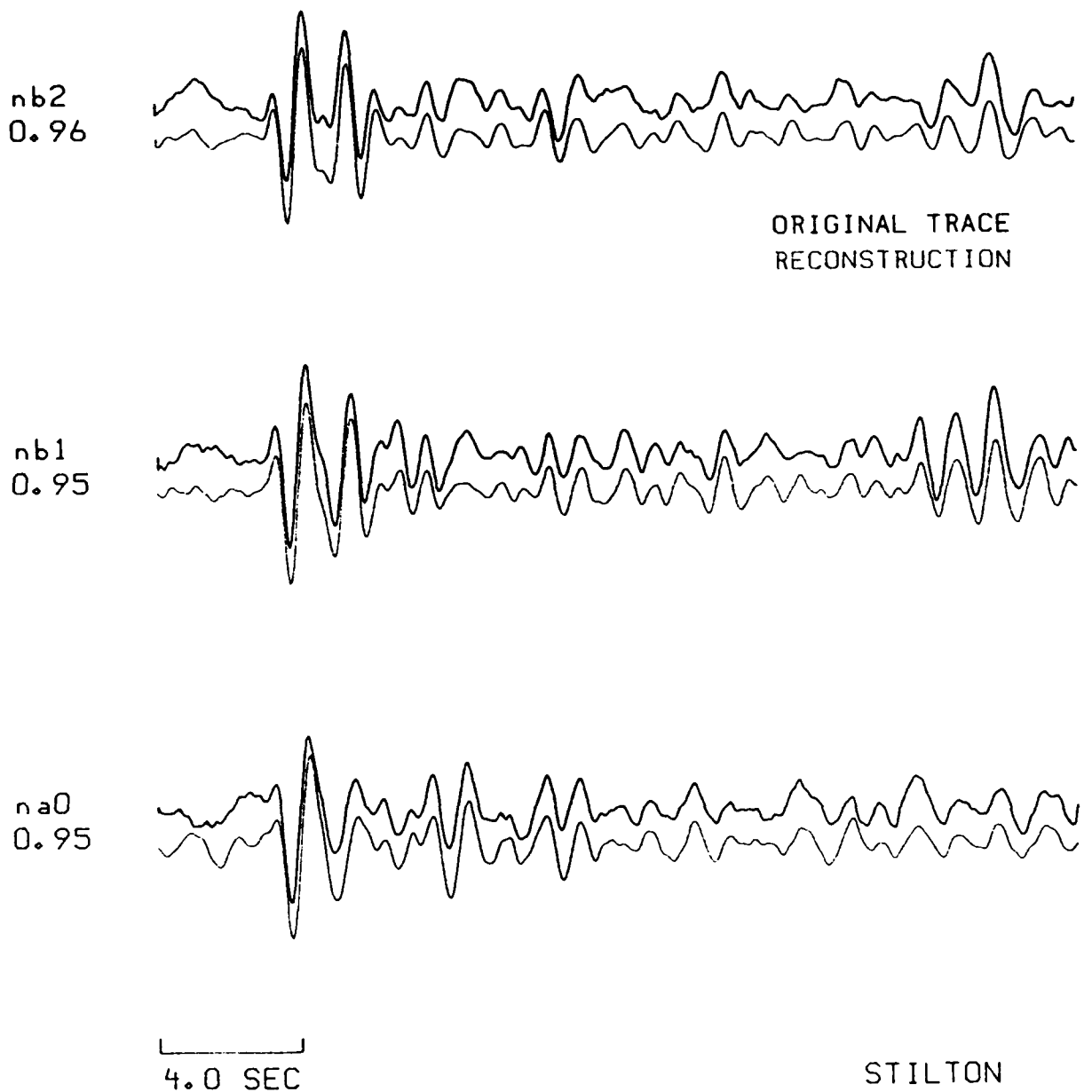
Figure 7b. Examples of trace reconstructions (bottom) and original traces (top) for the NTS event Stilton at NOR SAR for three sites. On the left side of each pair of traces is the name of the sensor and the correlation coefficient between the original and reconstructed traces.
