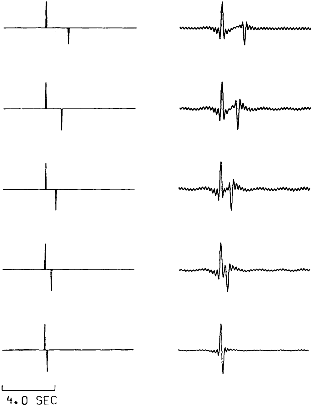
Figure 1. Band-limited deconvolution results for synthetic data. Input spike sequences for a range of pP times are shown on the left and the deconvolution output is shown on the right.
