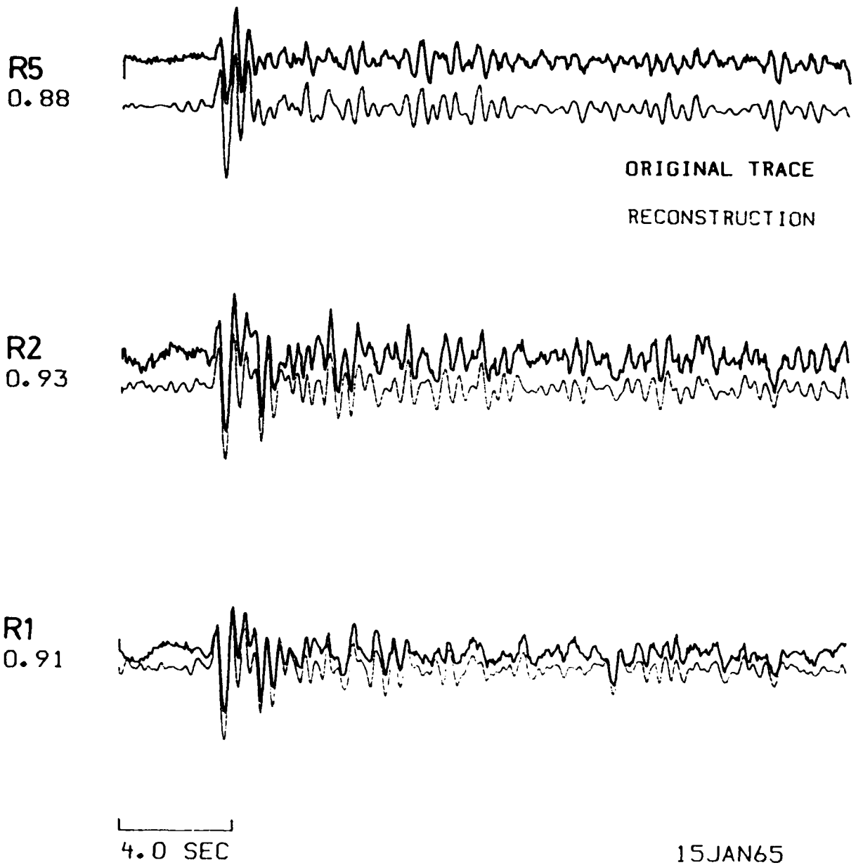
Figure 8b. Examples of trace reconstructions (bottom) and original traces (top) for the 15 January, 1965 cratering E-EKTS event at EKA for three sites. On the left side of each pair of traces is the name of the sensor and the correlation coefficient between the original and reconstructed traces.
