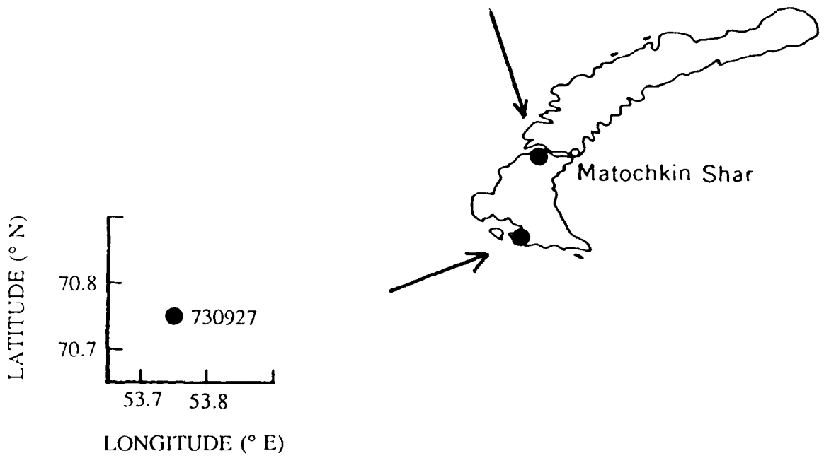
Figure 25. Locations of Novaya Zemlya events analyzed in this report
