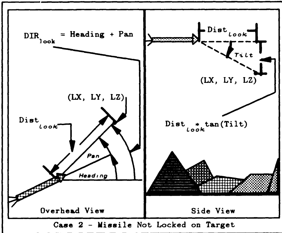
Figure 6.2 Determining the Camera's Look-at Position
