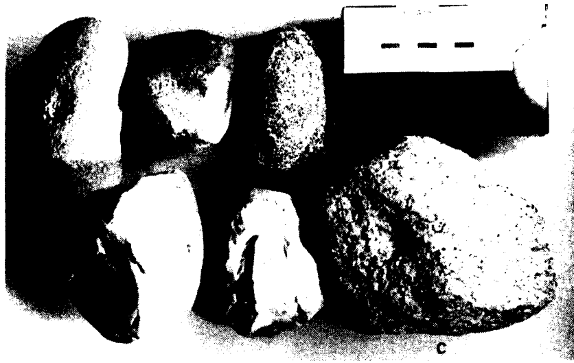
Figure 5.3: Hammerstones from the 13LA38 excavation; a,c) pitted; b) four hammers with battered edges (above igneous, below chert).
