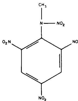
Figure B6. Tetryl.
