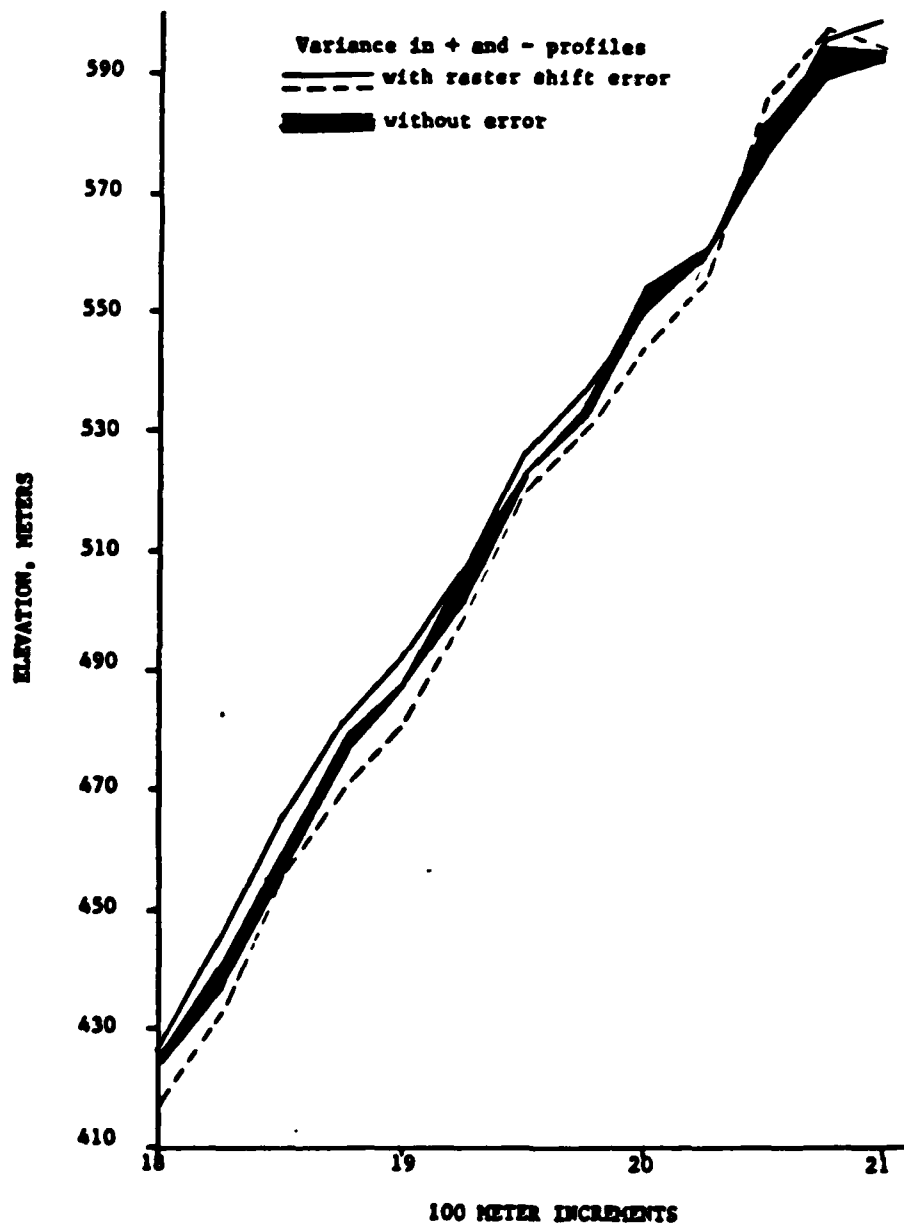
FIGURE 3. EFFECT OF RASTER SHIFT ERROR, SEGMENT B
