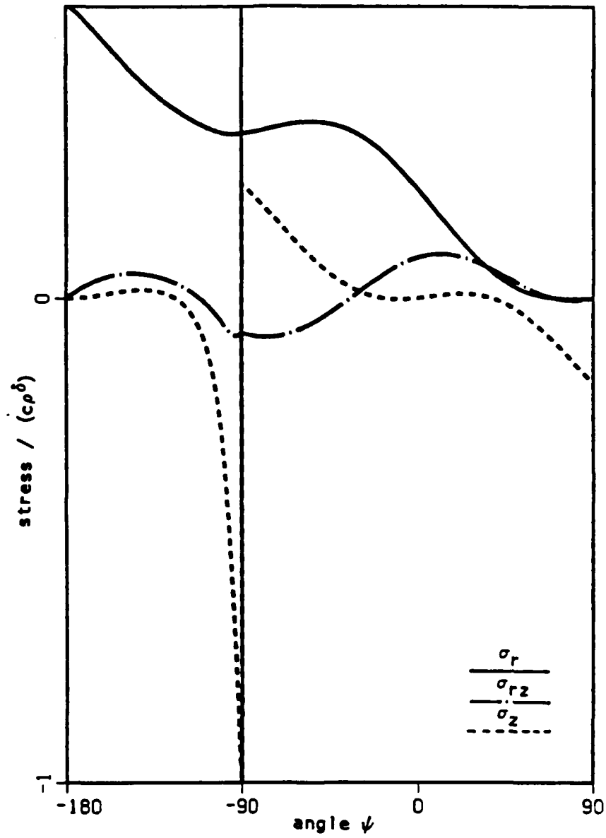
Fig.6 The normalized stresses from the first term of the eigenfunction associated with \delta_2 of Example 2
