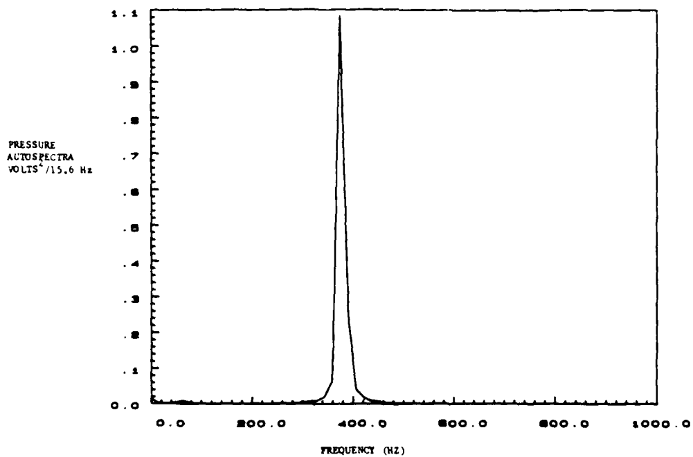
Fig. 5 Autospectrum of Pressure Fluctuations Under Acoustic Excitation at 385 Hz.
