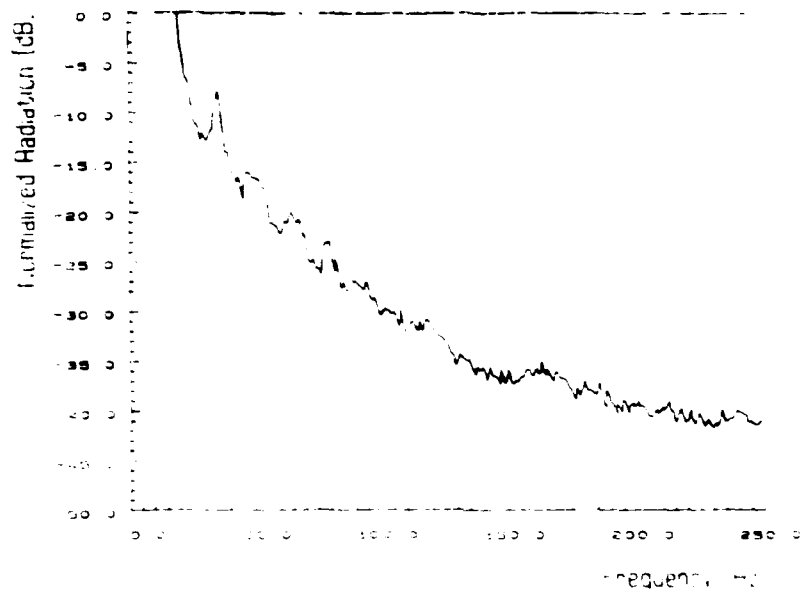
Fig. 6. Radiation Spectrum from entire Frame, in external structure.
