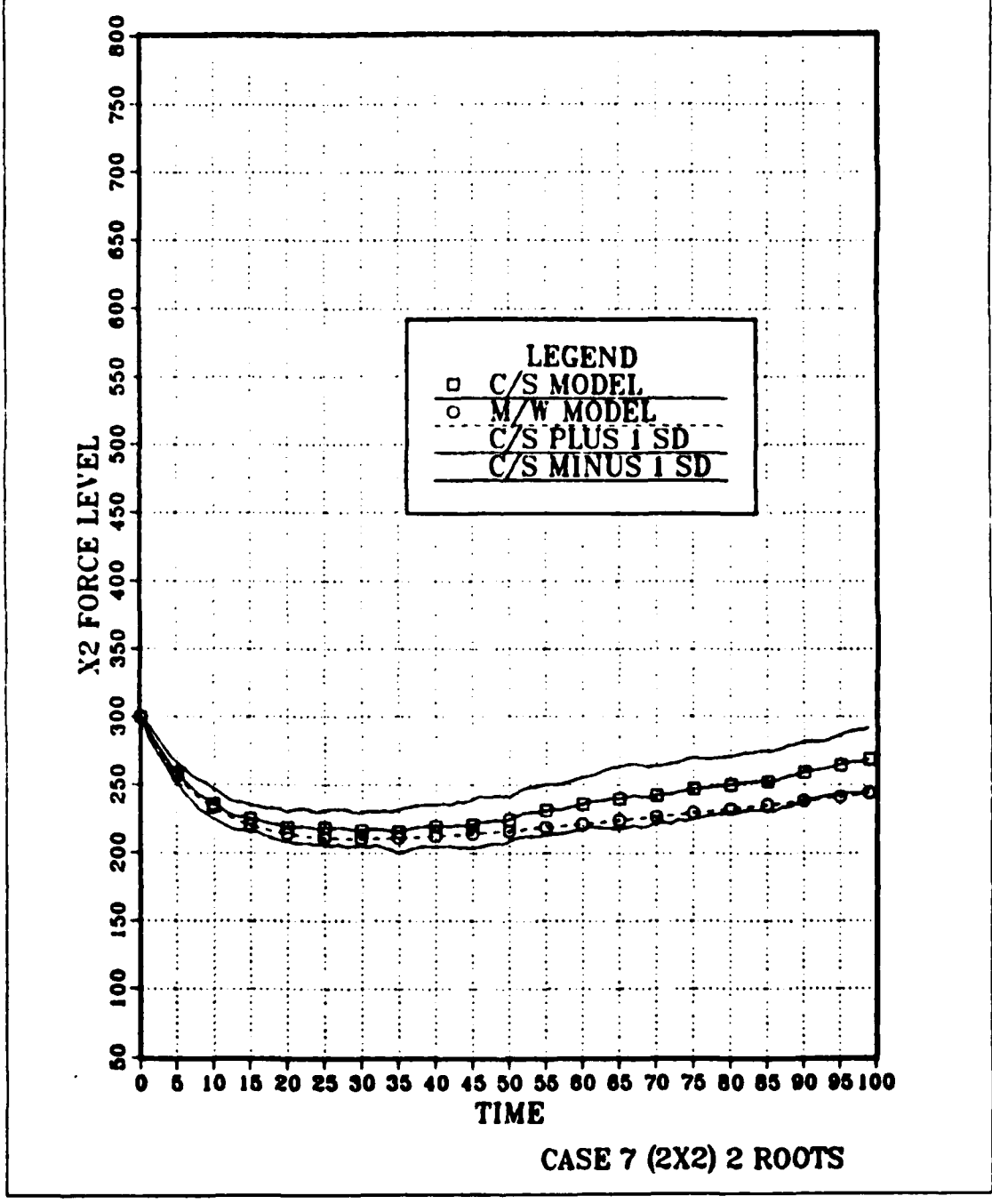
Figure E.30 X2 Force Level Trajectory Over Time For Case Seven.
