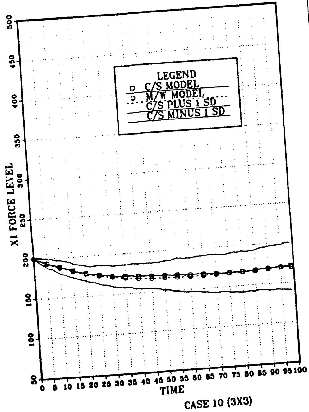
Figure 3.6 Example plot of x_1 force level trajectories.
