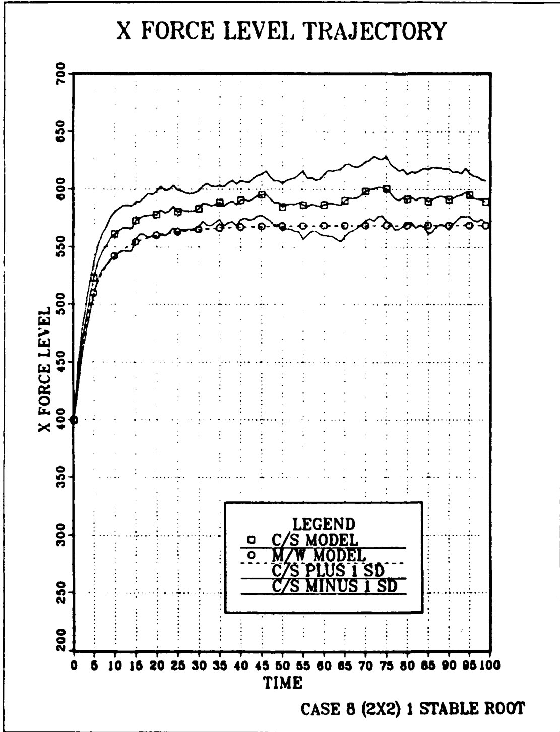
Figure E.34 X Force Level Trajectory Over Time For Case Eight.
