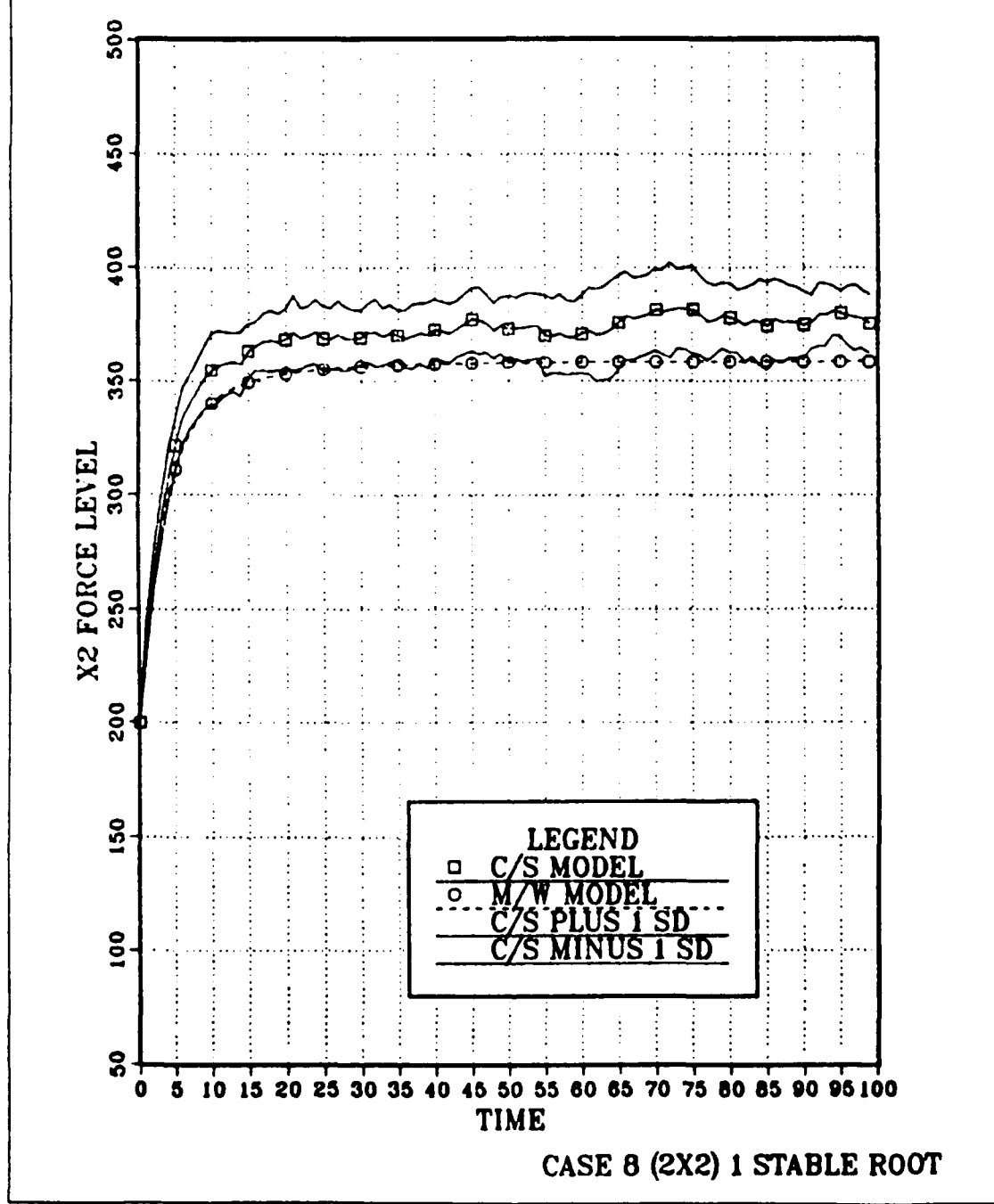
Figure E.37 X2 Force Level Trajectory Over Time For Case Eight.
