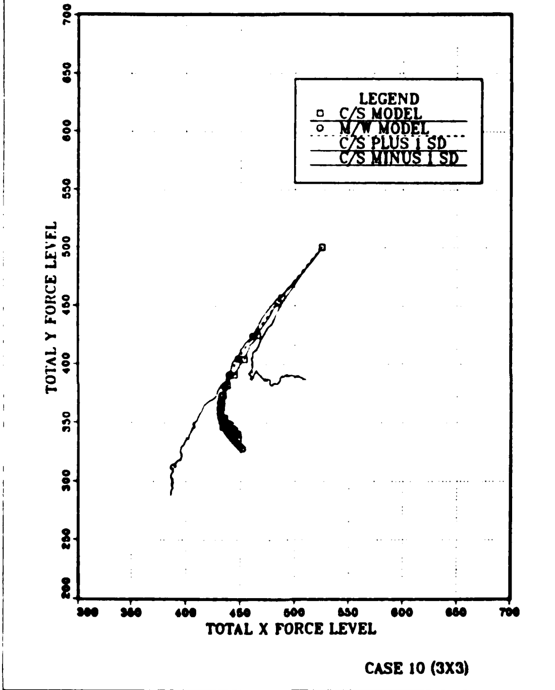
Figure 3.5 Example Total Force Level Trajectory Plot.
