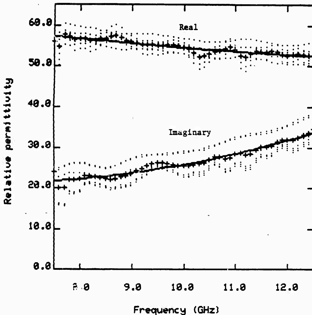
Figure 5. A plot of the relative permittivity of water. The data were taken at X-band using the HP8510 Vector Network analyser and the measurement was repeated three times with the sample repositioned between measurements. The dots are EPOST inversions of the data for both S11 and S21. The crosses result from a REFPOSTTEK analysis on the three sets of data. The line was generated by program Posttek operating on all three data sets and fitting the data to second order polynomial representatives for the frequency dependence of \epsilon' and \epsilon'' .
