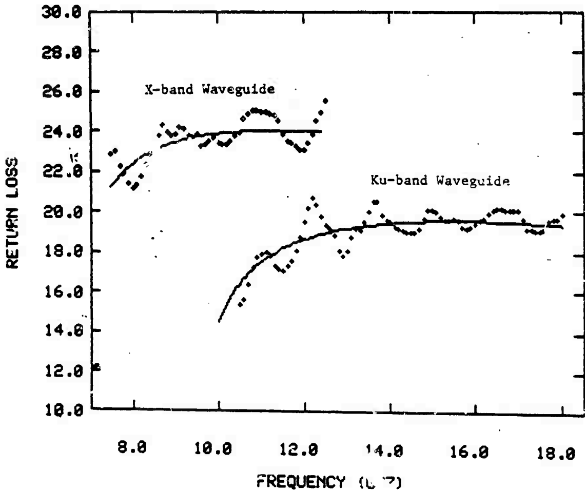
Figure 4. A plot of the measured return loss (+) and the calculated return loss for a sample of Ni substituted phthalocyanine in kevlar. The return loss measured at the two waveguide bands differ since the characteristic impedance of the waveguides are different. The calculated curve is generated by program POSTCL using a complex dielectric constant and complex conductivity found by program POSTTEK.
