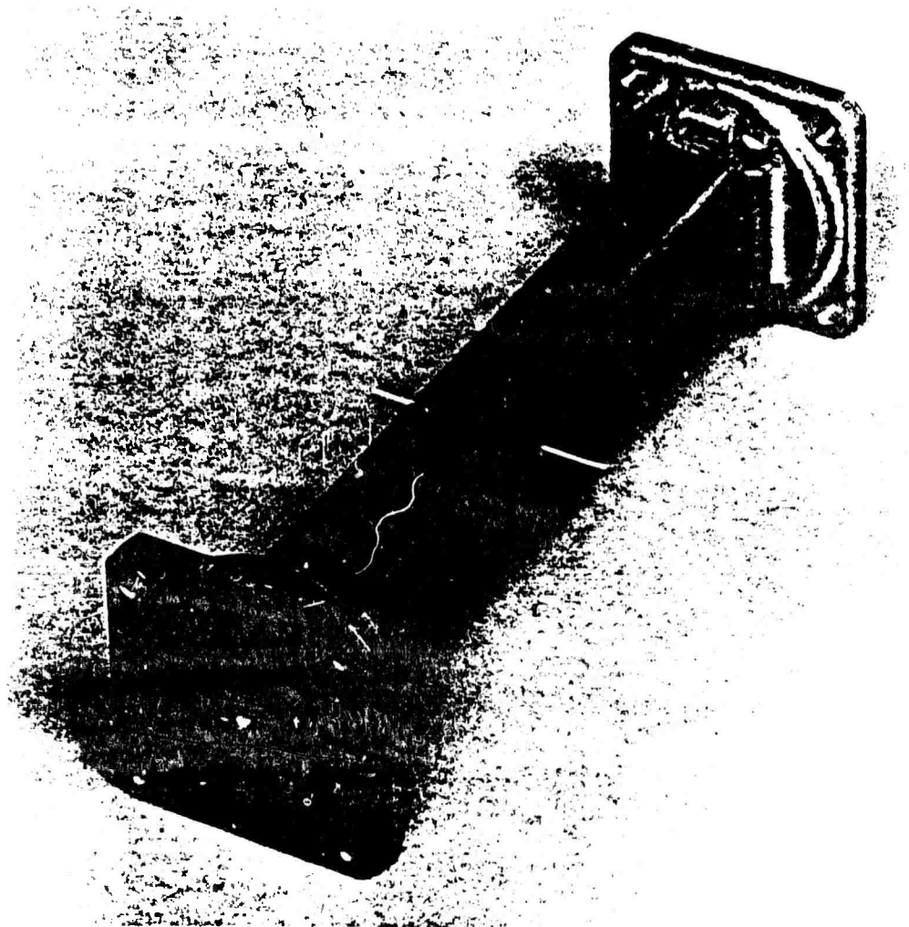
Figure 1. A simple test fixture for the dielectric-post-in-waveguide measurements at X-band.
