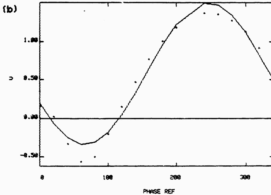
Figure 8. Plots generated by program PHASETEK (a) showing all the input phase data versus frequency and (b) a single frequency fit of the phase data versus phase shifter setting at a single frequency. In figure 8a there is one curve for each 20 degrees of phase shift. The plots are displayed in differing color and line style on a color terminal to help distinguish the various curves.
