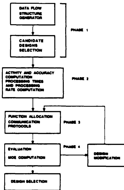
Figure 1. Design Methodology Flowchart
