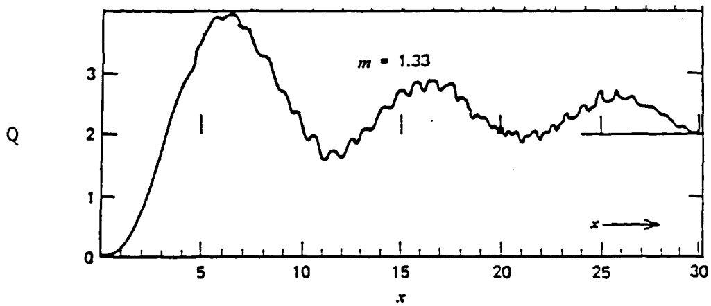
Fig. 8. Extinction curve for water spheres calculated from Mie theory (from Friedlander, 1977). Q and x are dimensionless.
