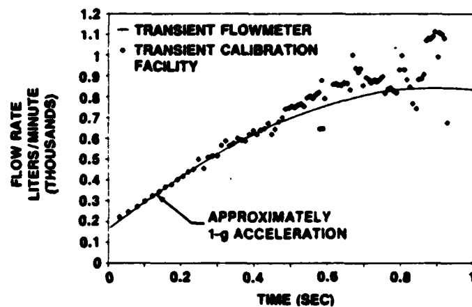
Fig. 4. Typical Transient Calibration Curve
