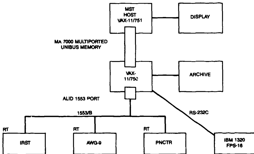
FIGURE 5. Real-Time System Hardware Architecture.
