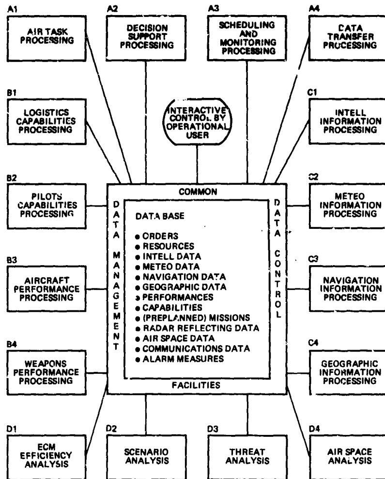
Fig. 15 Architecture of mission preparation information system
