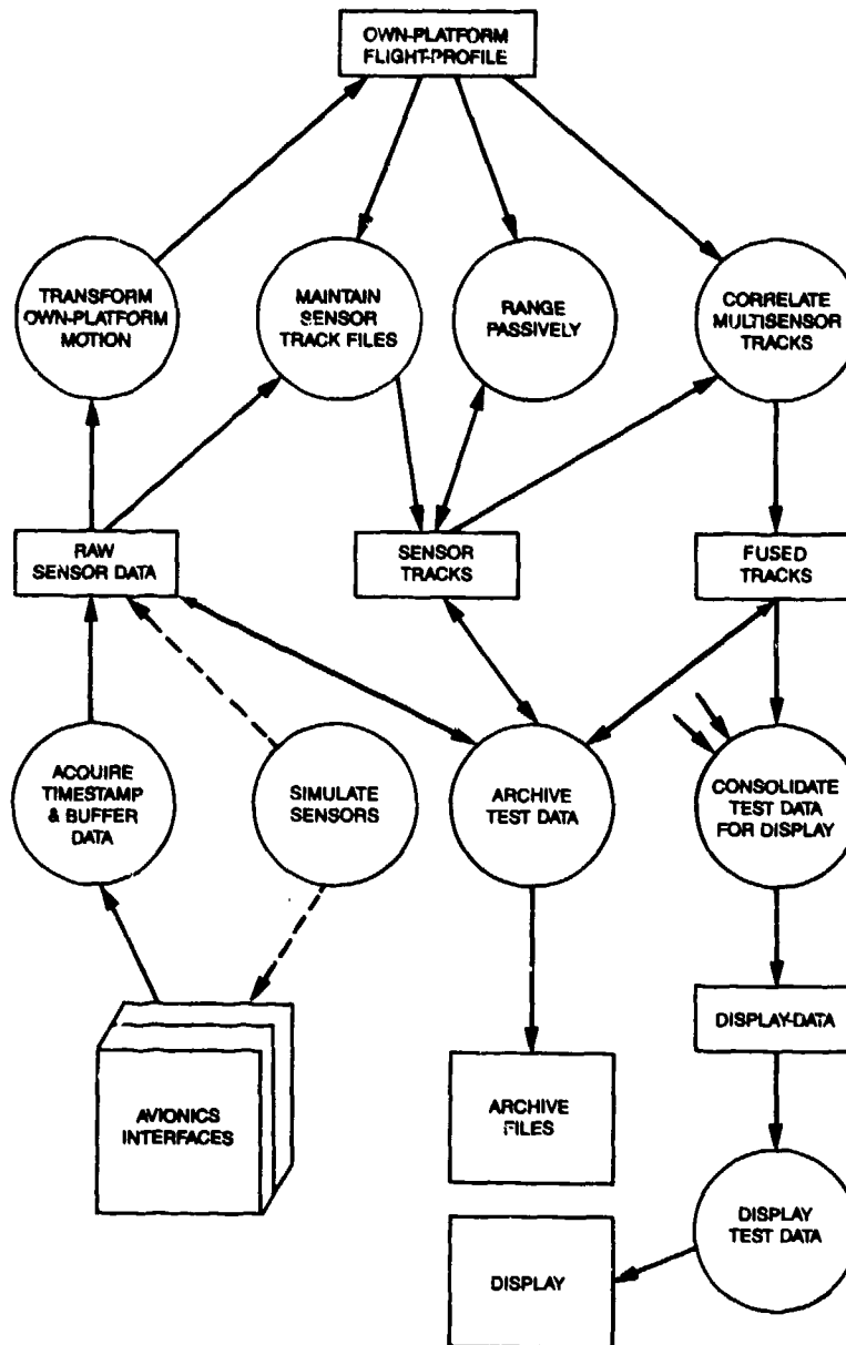
FIGURE 6. Real-Time System Software Architecture.
