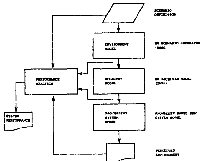
Figure 4 EVALUATION SYSTEM
