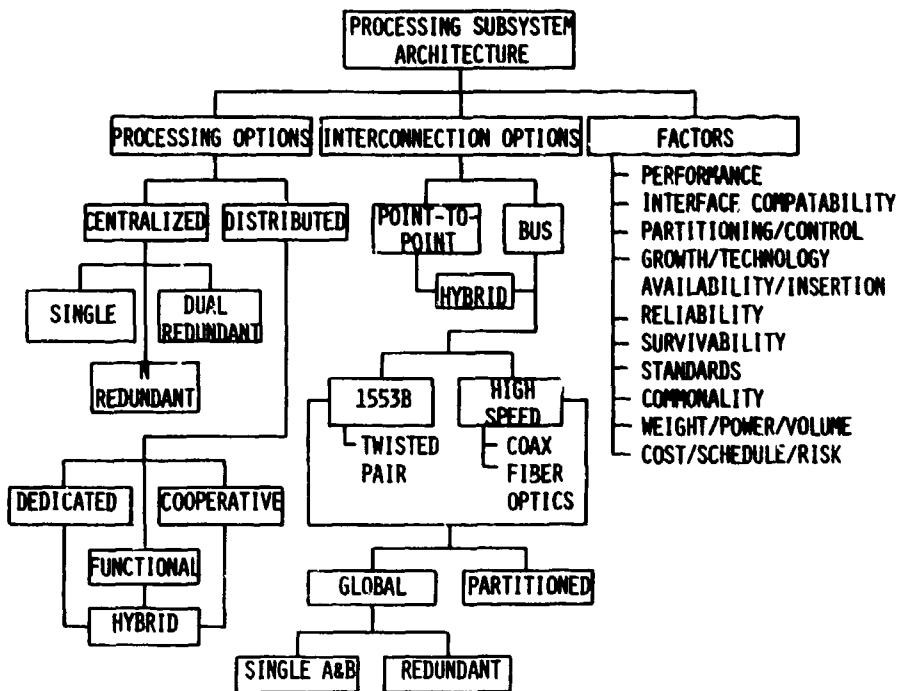
Figure 2. Design Considerations/Trade-Offs
