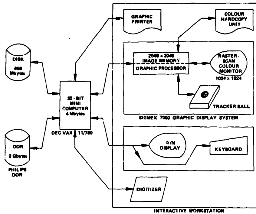
Fig. 13 Current CAMPAL configuration at Royal Netherlands Air Force Base
