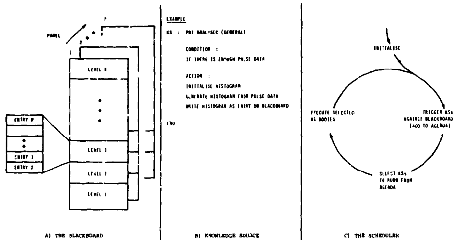
FIGURE 2 BLACKBOARD ELEMENTS
