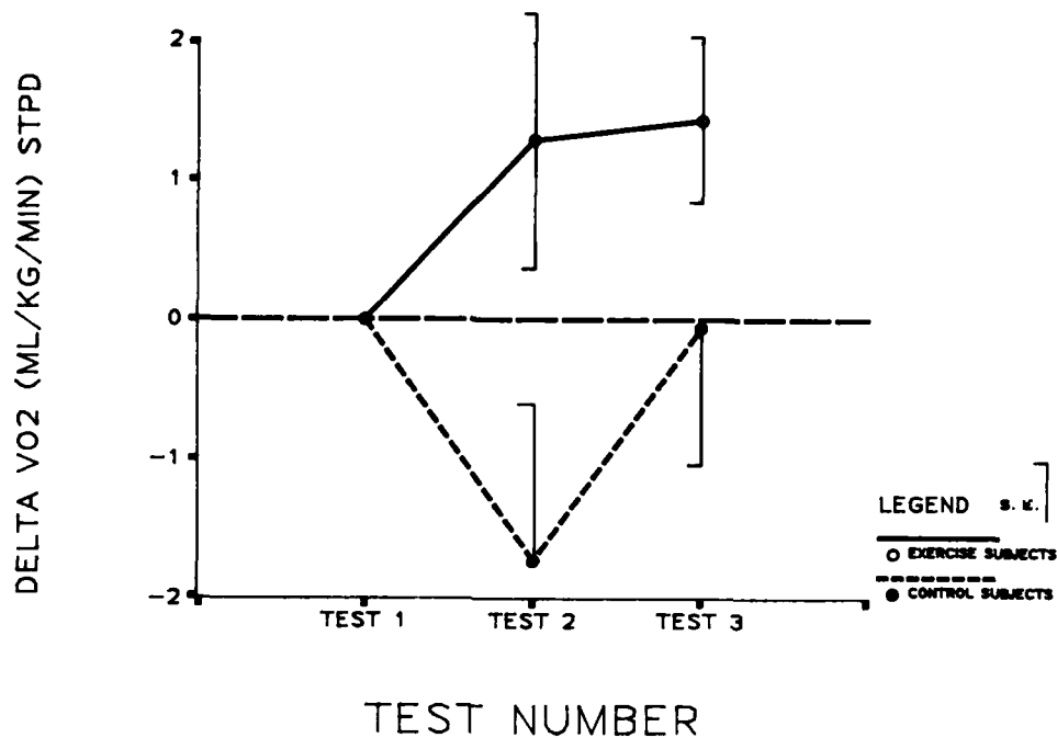
Figure 2. Mean maximal oxygen uptake ( \text{ml}\cdot\text{kg}^{-1}\cdot\text{min}^{-1} ) changes (delta scores) for the exercise (N=15) and control (N=15) groups between tests 1 and 2 and 1 and 3. The vertical bars represent the standard error of the means.
