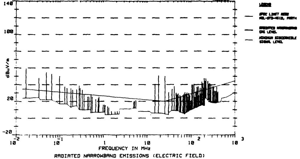
FIG 27 - STANDARD MODEL 1100 GRID COMPUTER RADIATED NARROWBAND EMISSIONS (ELECTRIC) DISPLAY PANEL FOLDED DOWN
