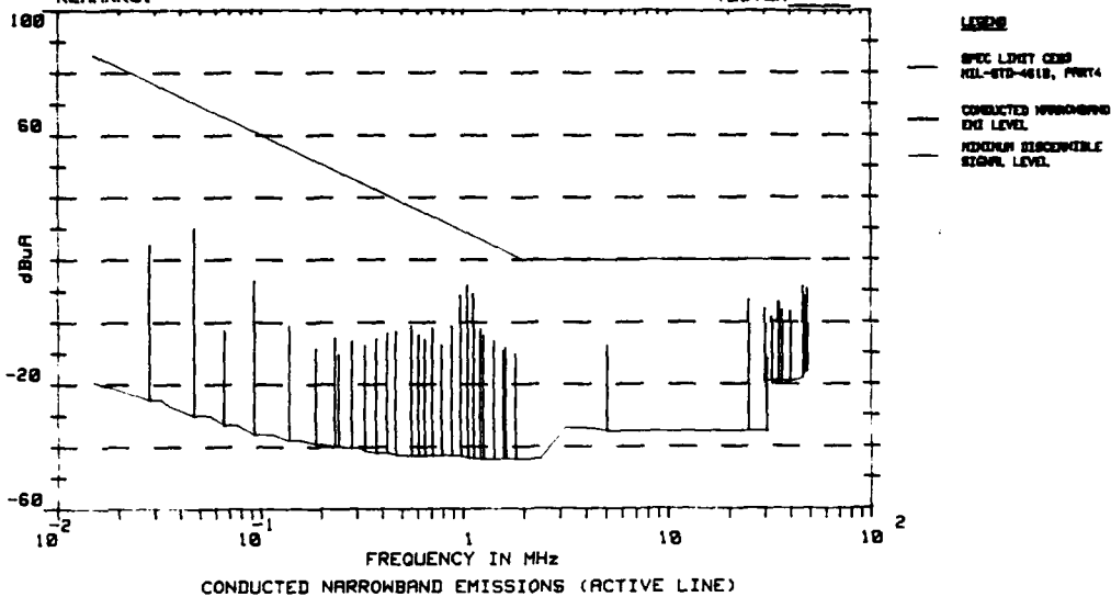
FIG 19 - STANDARD MODEL 1100 GRID COMPUTER CONDUCTED NARROWBAND EMISSIONS (ACTIVE LINE)
