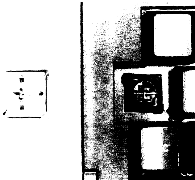
FIG 14 - TAB KEY FAILURE OF TEMPEST MODEL 1107 GRID FROM FREE FALL TEST DEF STAN 07-55 PART 2 SECTION 1/1 TEST A9
