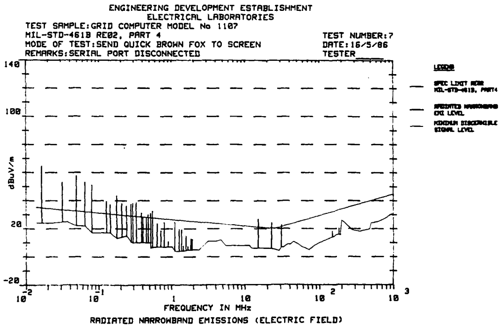
FIG 26 - TEMPEST MODEL 1107 GRID COMPUTER RADIATED NARROWBAND EMISSIONS (ELECTRIC) SERIAL CABLE DISCONNECTED
