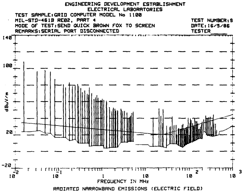
FIG 25 - STANDARD MODEL 1100 GRID COMPUTER RADIATED NARROWBAND EMISSIONS (ELECTRIC) SERIAL CABLE DISCONNECTED
