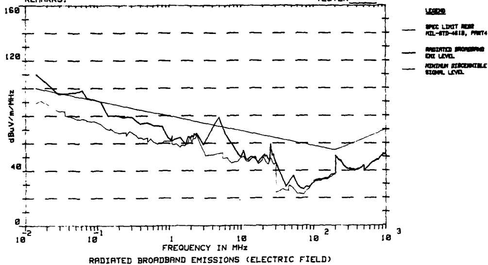
FIG 29 - TEMPEST MODEL 1107 GRID COMPUTER RADIATED BROADBAND EMISSIONS (ELECTRIC)
