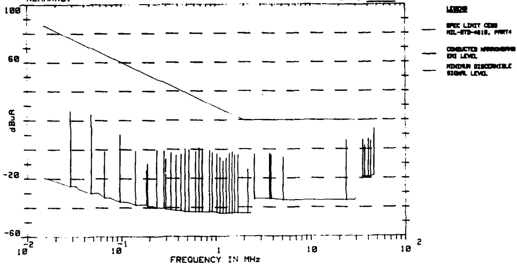
CONDUCTED NARROWBAND EMISSIONS (NEUTRAL LINE)
