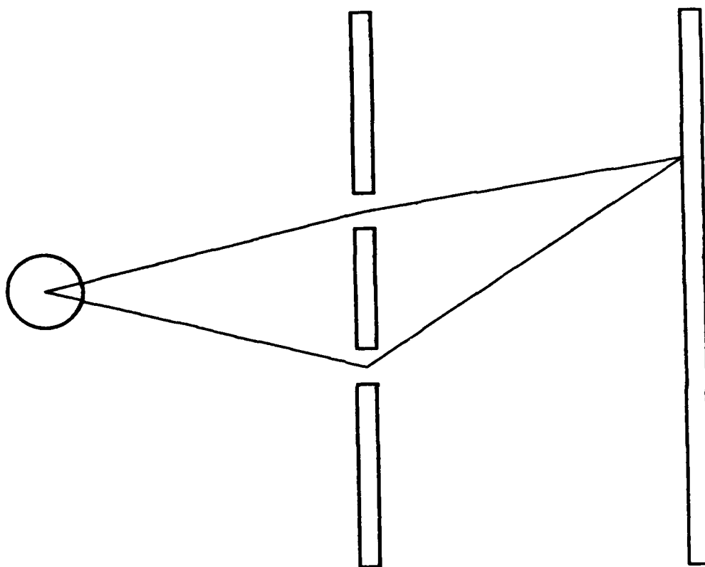
Figure 5: 2 slit experiment setup.
