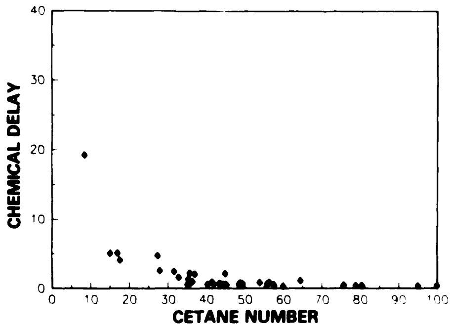
Figure 18. Chemical ignition delay versus cetane number for all fuels at 482°C
