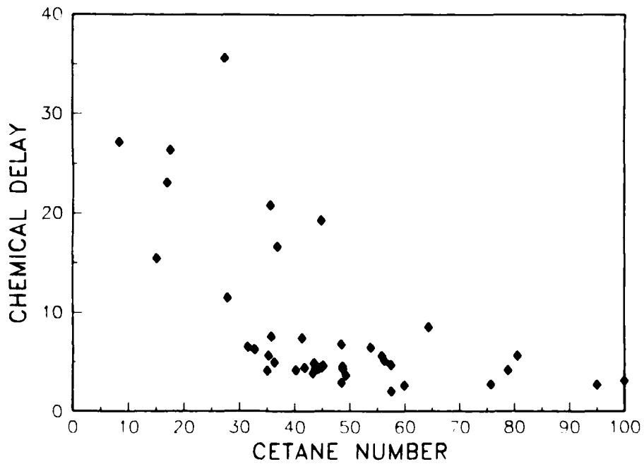
Figure 10. Chemical ignition delay versus cetane number for all fuels at 371°C
