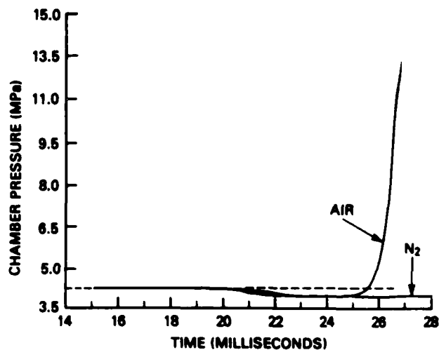
Figure 6. Pressure-time records, 50/50 blend of hexadecane and heptamethylnonane in both air and nitrogen
