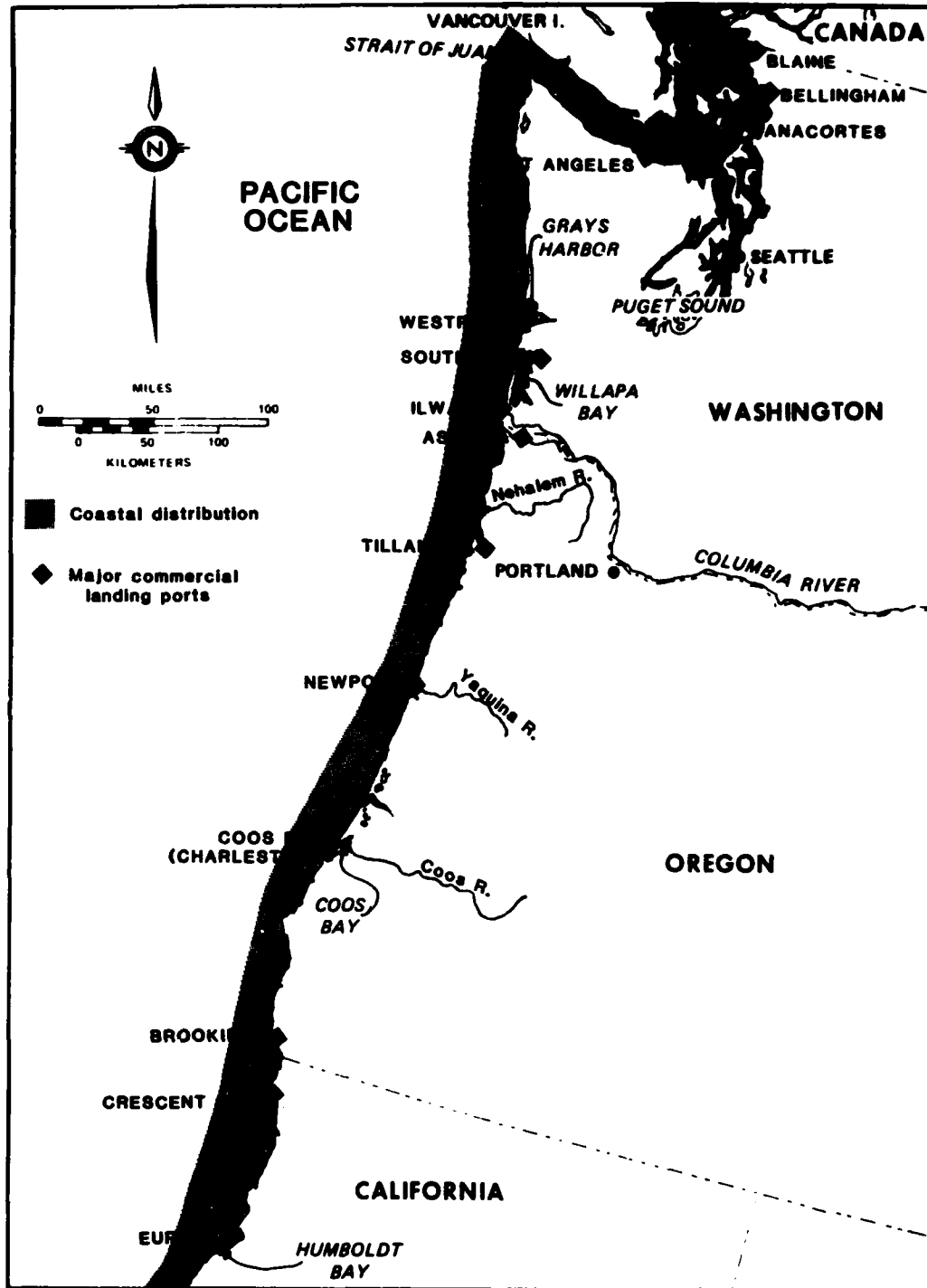
Figure 2. Distribution of the Dungeness crab in the Pacific Northwest.
