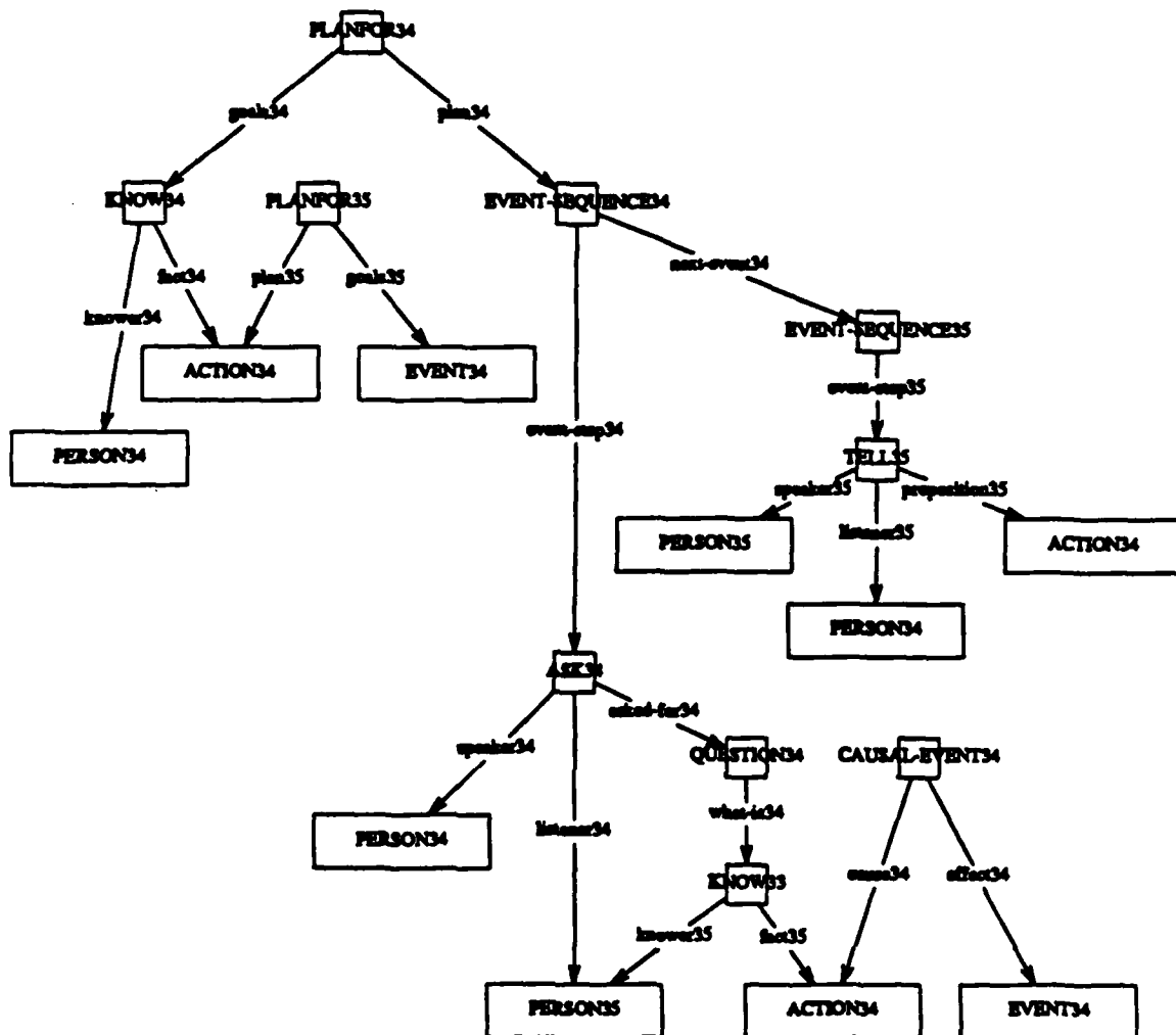
Figure 11 A plan for knowing is to ask if the hearer knows.
