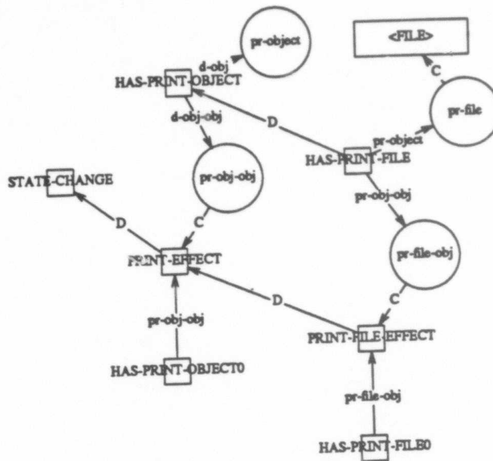
Figure 6 Relational constraint on PRINT-FILE-EFFECT.
