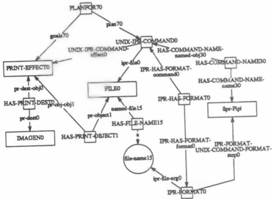
Figure 27 Output from UCPlanner
