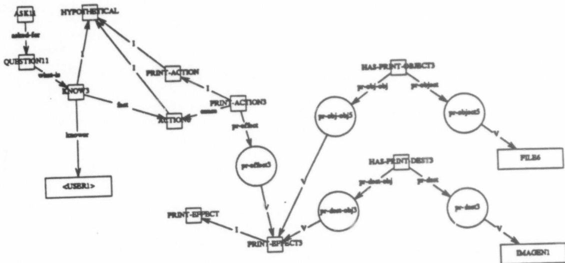
Figure 2 ALANA's output for "Do you know how to print a file on the Imagen?"
