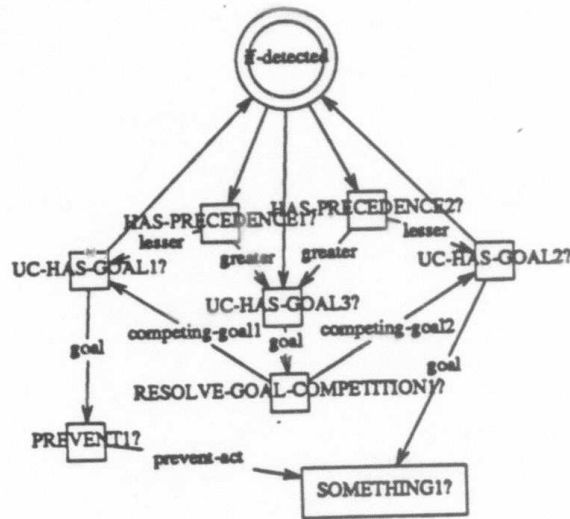
Figure 17 If-detected demon for detecting goal conflicts.
