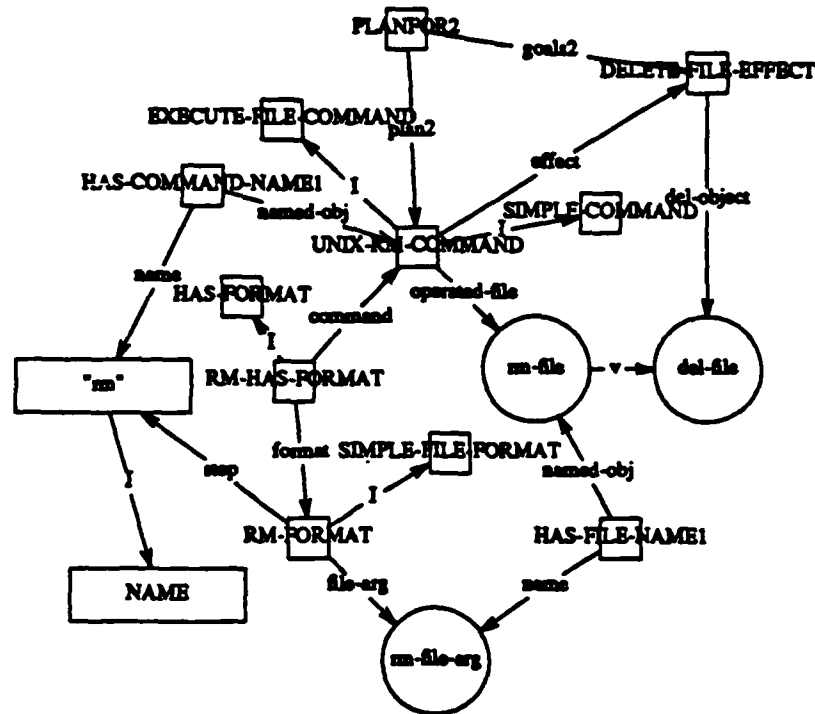
Figure 24 Representation of plan to delete a file by using the rm command
