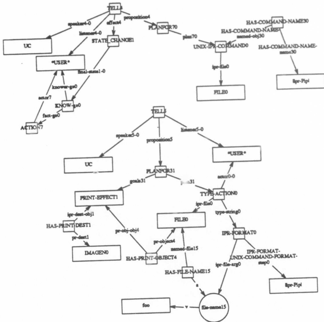
Figure 29 The output of UExpress.
