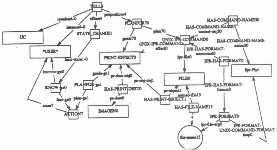
Figure 28 The input to UCEXpress.
