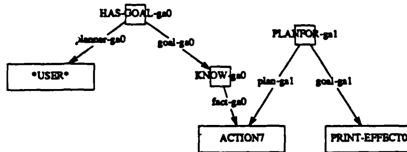
Figure 13 PAGAN output
