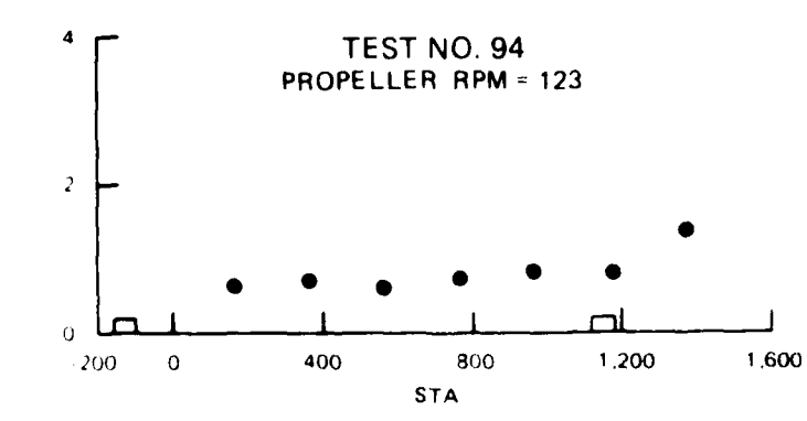
SPEED ALONG LOCK CHAMBER TESTS 91 - 94
