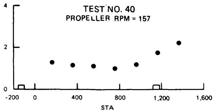
SPEED ALONG LOCK CHAMBER TESTS 37 - 40
