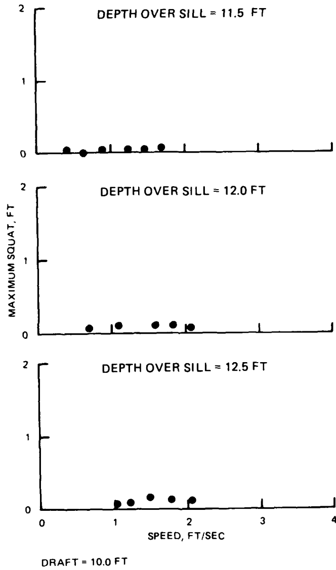
Figure 24. Maximum squat versus constant speed for entering loaded tow being pulled by towing mechanism
