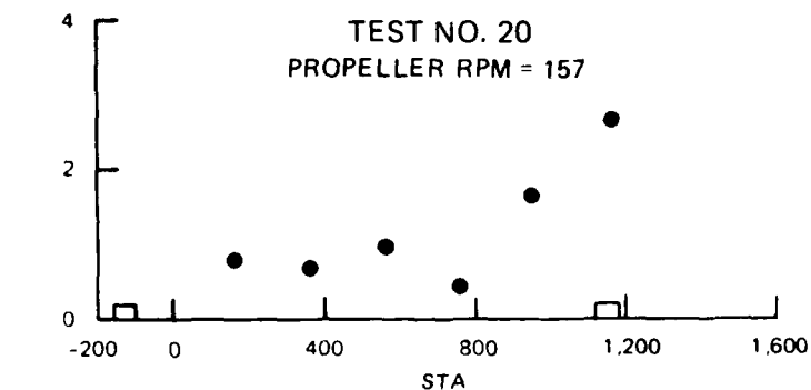
SPEED ALONG LOCK CHAMBER TESTS 17 - 20
