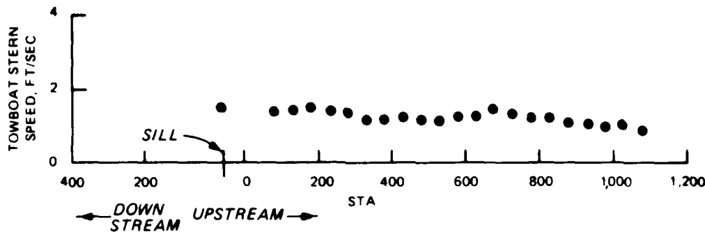
Figure 9. Tow speed, Paul Legeay , downbound exiting
