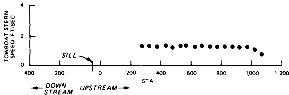
Figure 10. Tow speed, David McAllister , downbound exiting
