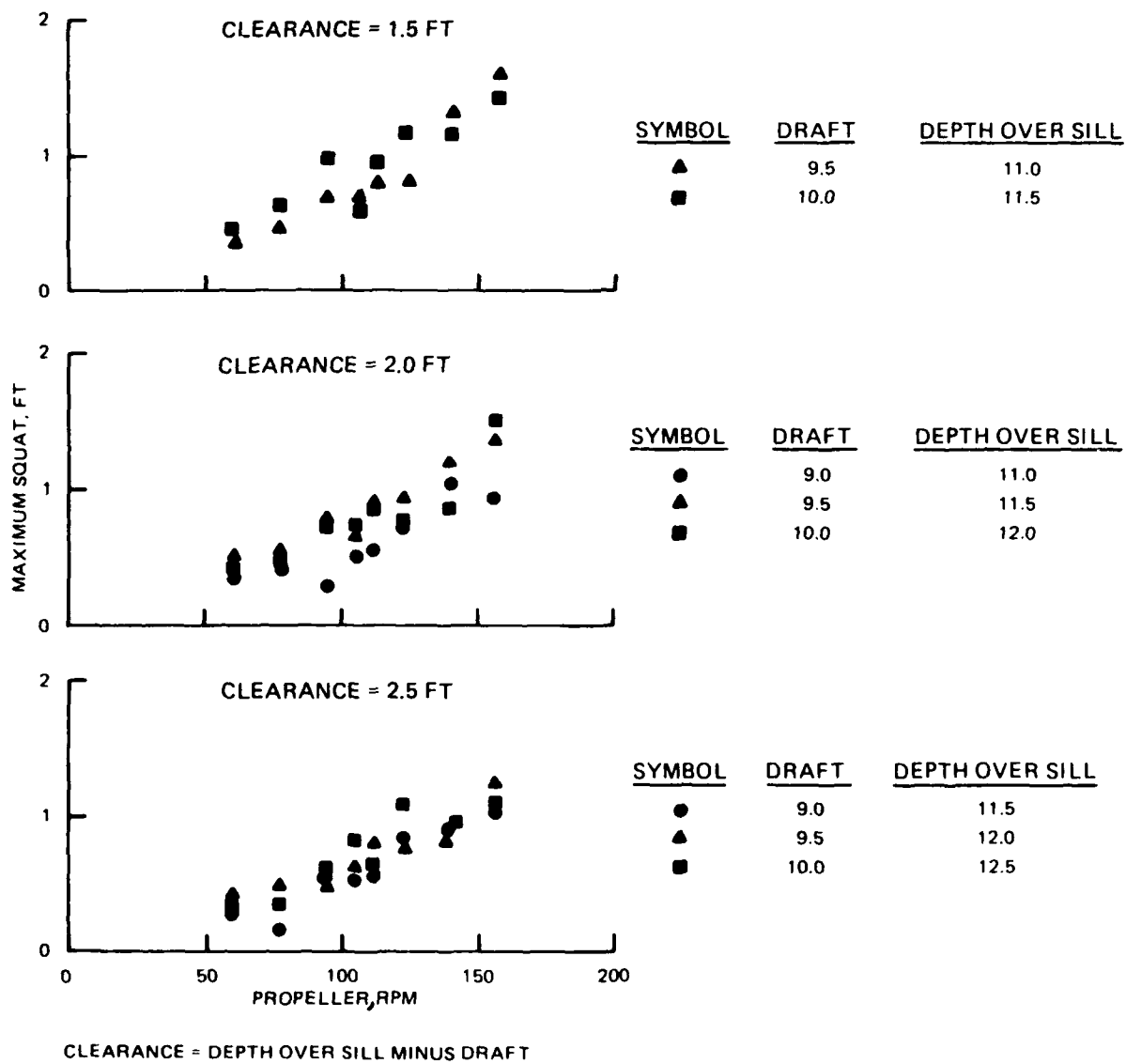
Figure 21. Maximum squat versus propeller speed for entering loaded self-propelled tow
