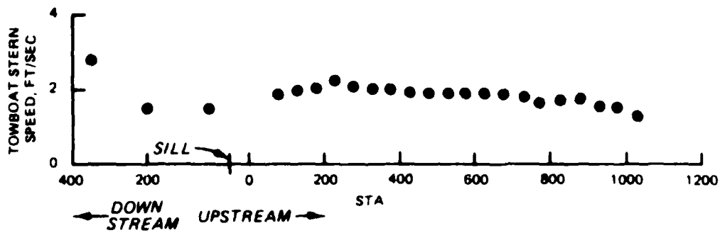
Figure 11. Tow speed, Louis Meece , downbound exiting
