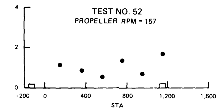
SPEED ALONG LOCK CHAMBER TESTS 49 - 52
