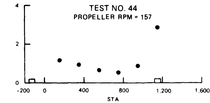
SPEED ALONG LOCK CHAMBER TESTS 41 - 44
