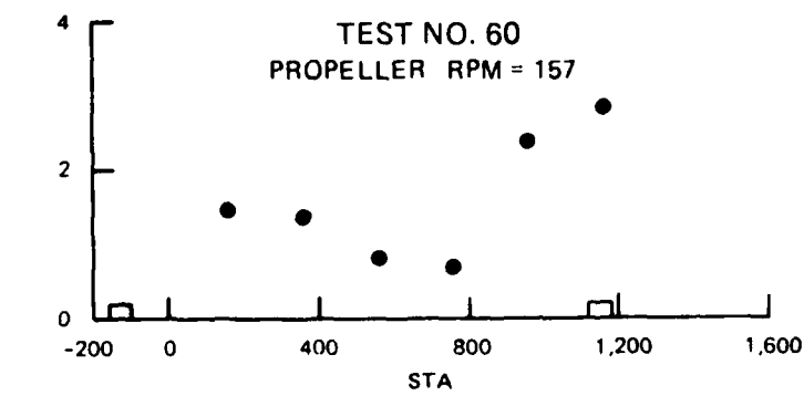
SPEED ALONG LOCK CHAMBER TESTS 57 - 60
