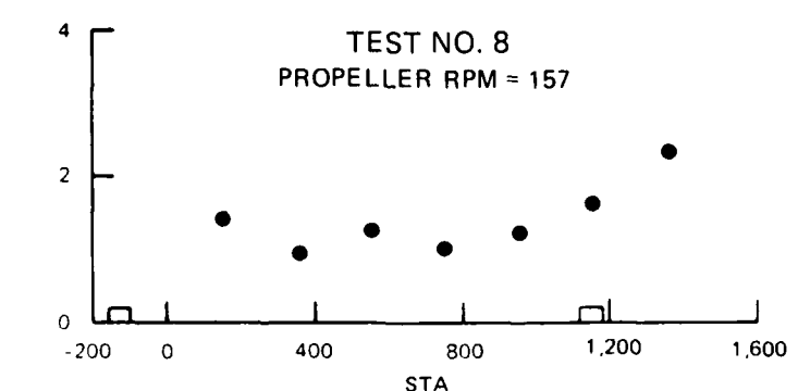
SPEED ALONG LOCK CHAMBER TESTS 5 - 8
