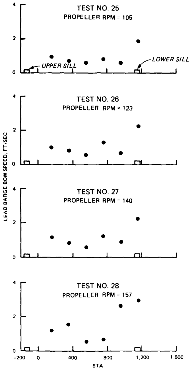
SPEED ALONG LOCK CHAMBER TESTS 25 - 28
