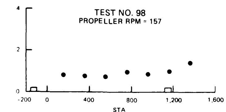
SPEED ALONG LOCK CHAMBER TESTS 95 - 98
