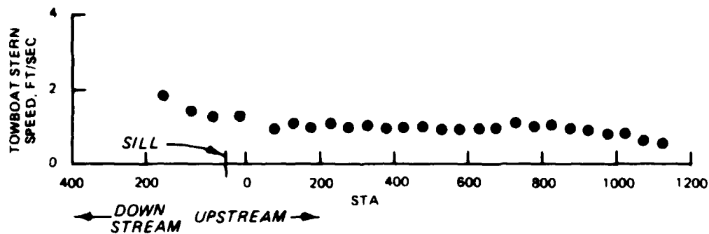
Figure 12. Tow speed, William Pitt , downbound exiting
