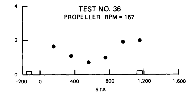
SPEED ALONG LOCK CHAMBER TESTS 33 - 36
