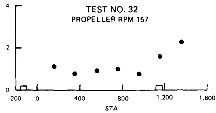
SPEED ALONG LOCK CHAMBER TESTS 29 - 32
