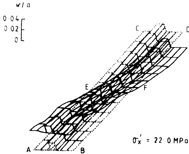
FIG 8 Long Panel (a = 3500 mm): Computed Deformation Showing Local Buckling Caused by Secondary Compression
