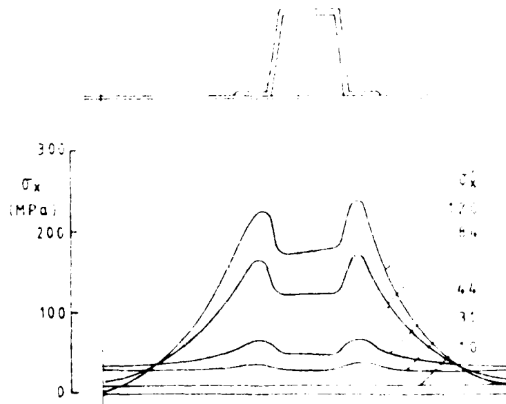
FIG 10 Compressive Stress Distributions Across Shell Laminate Showing Reduced Effective Width
