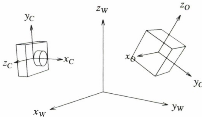
Fig.3.4. Traditional Definition of Positions and Orientations.
