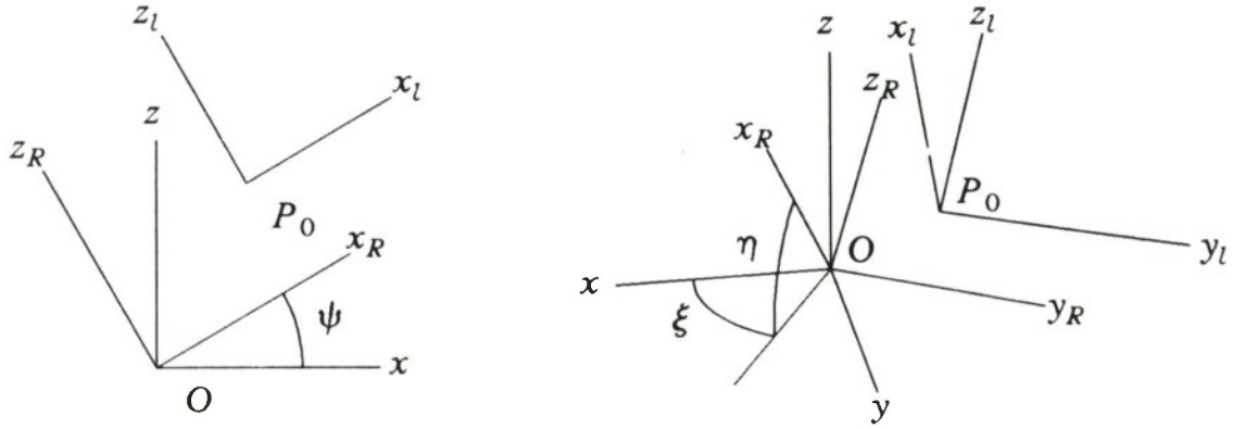
Fig.3.3. Global, Rotated and Local Systems of Axes
