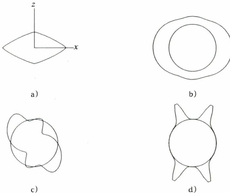
Fig.5.4. 2-D Curve and Polar plots of 2-D Transforms. a) Superconic with exponent 1.2, b) Support Transform, c) Tangential Component of Vector Support Transform, d) Curvature Transform.
