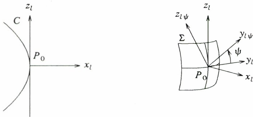
Fig.3.9. Local Axes for the definition of Curvatures in 2-D and 3-D.
