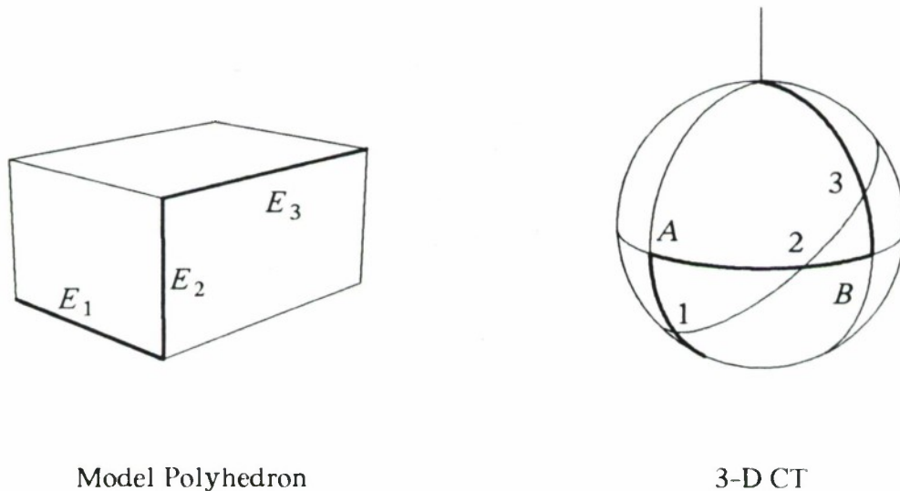
Fig.8.19. Three Model Edges and the corresponding CT arcs
