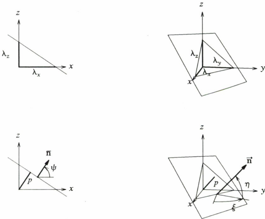
Fig.3.2. Tangential Coordinates.
