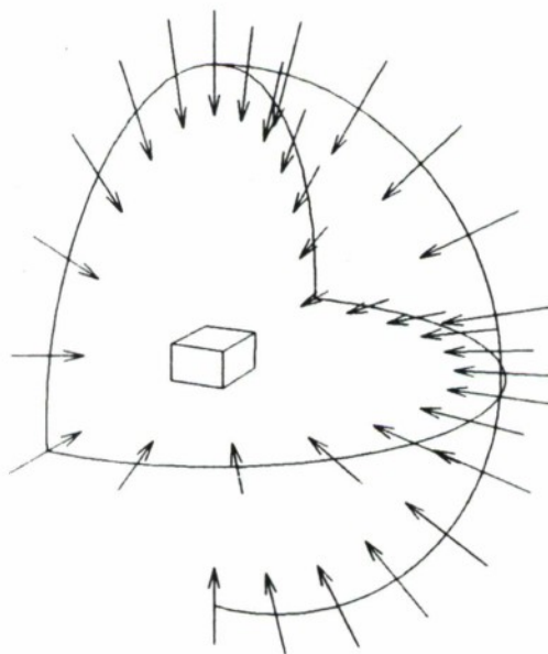
Fig.8.17. A sufficient set of viewing directions for reconstruction with the CT.
