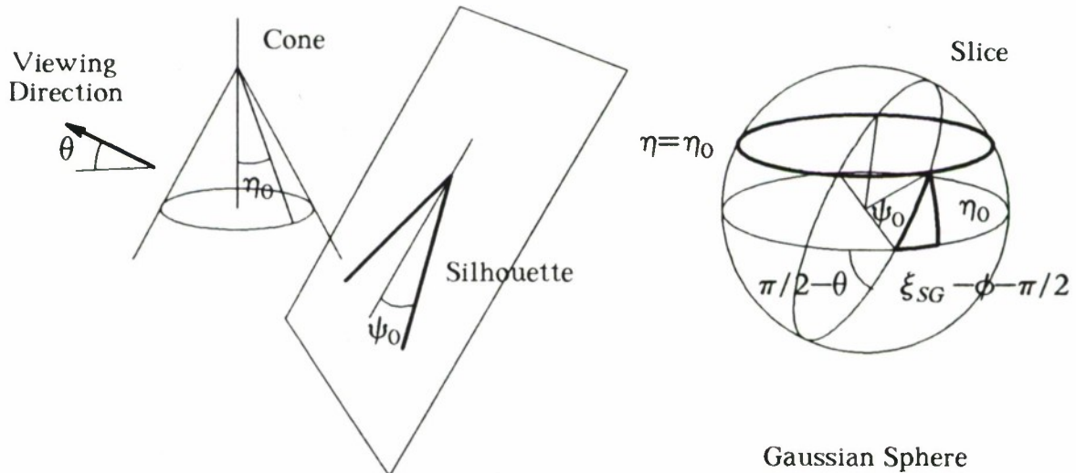
Fig.4.8. Silhouette of the Cone and Gaussian Sphere.
