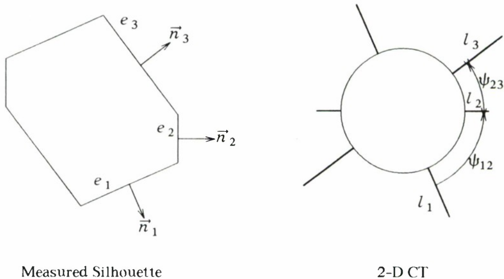
Fig.8.18. Three Silhouette Edges and the corresponding CT
