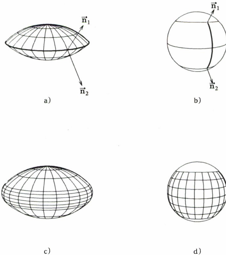
Fig.7.5. Surface with a Curved Edge a) Surface with sharp edge. b) Gaussian image of a point on the edge. c) Surface with smooth edge. d) Gaussian image of smooth edge.
