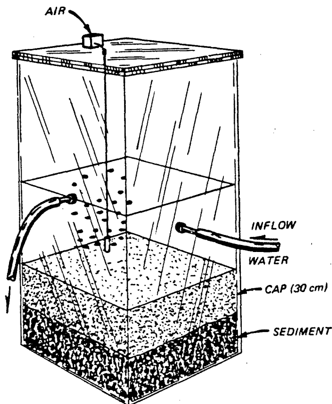
Figure 2. Large-scale reactor units used for verification tests
