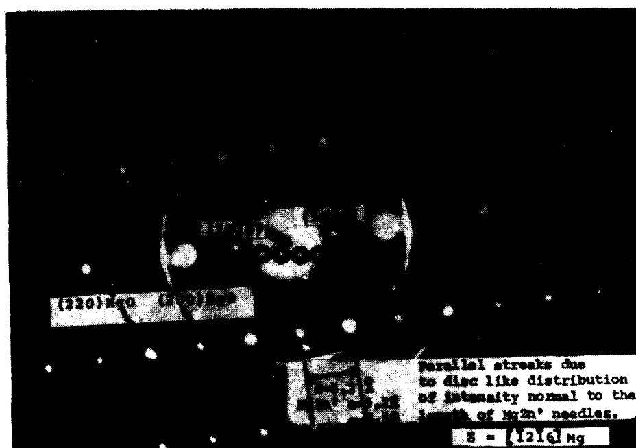
Figure 13. Electron diffraction pattern of MgZn' precipitates showing the reciprocal lattice planes parallel to the basal plane of the the magnesium.
