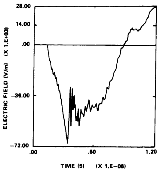
Figure 18. Electric field measured at 10 meters (from oscilloscope trace).
