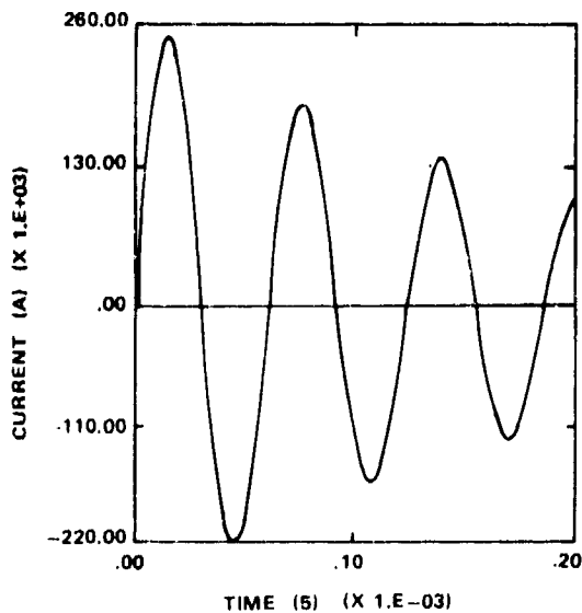
Figure 15. Injection current waveform for peak current, direct strike tests.
