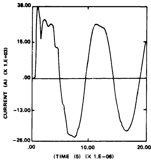
Figure 13. Direct strike current waveforms.
