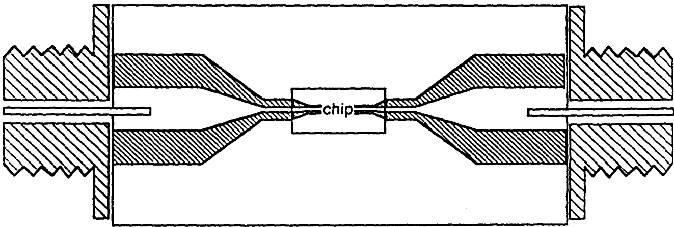
test fixture
