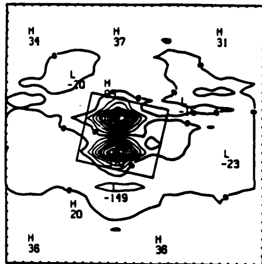
Figure 8 Typical error estimate of the u velocity (dimensionless \times 10^4 ). The estimate has been normalized by |U|_{\text{max}} = 27 \text{ m/sec} .
