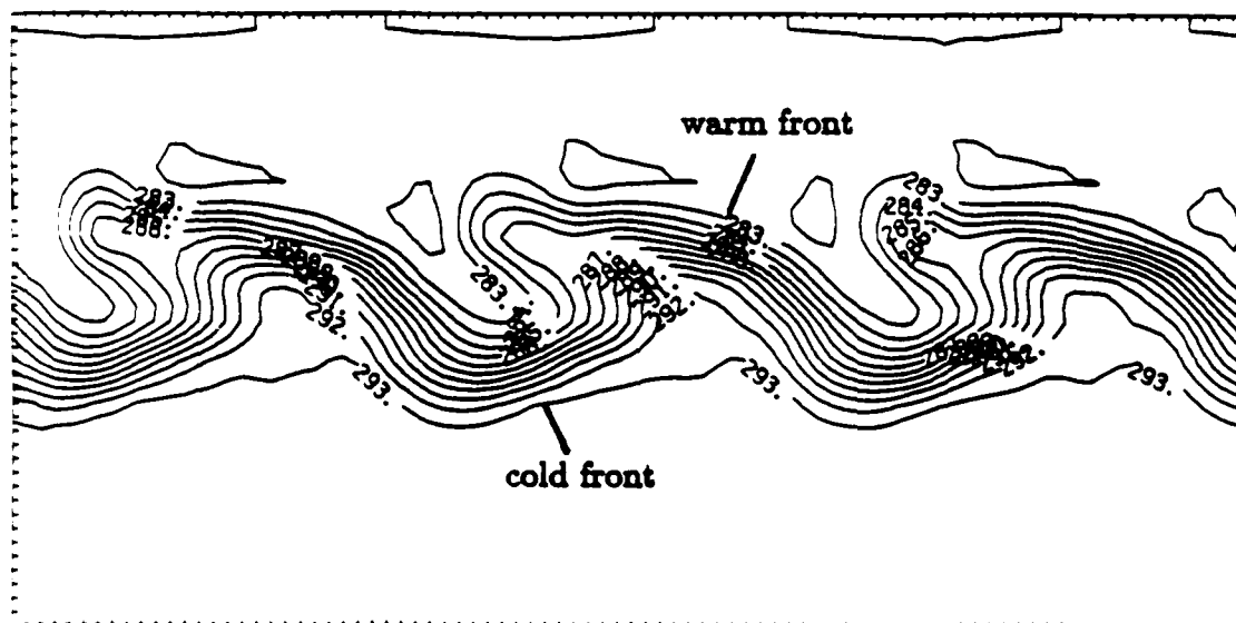
Figure 10 Temperature ( K ) on the \sigma = 0.9 surface at t = 0 . . Locations of the warm and cold fronts are shown.
