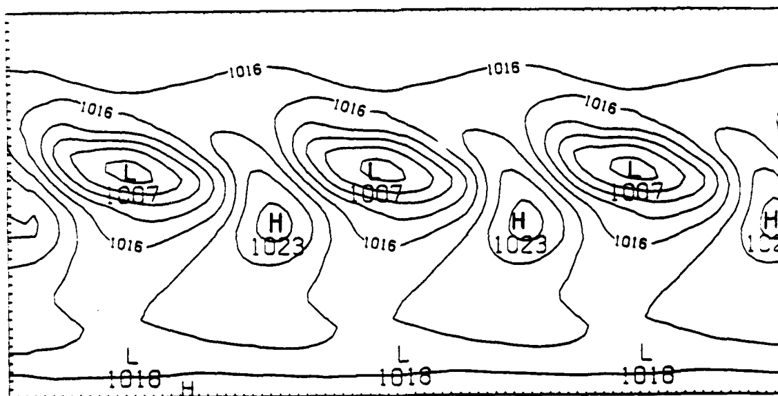
Figure 12 Surface pressure (millibars) for the baroclinically unstable wave at t = 0 .
