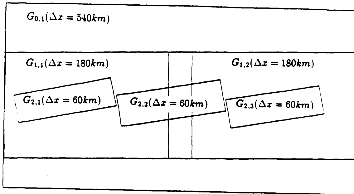
Figure 1 Adaptive run with two levels of refinement. G_0 is the coarse grid, G_1 fine and G_2 finer resolution grids.
