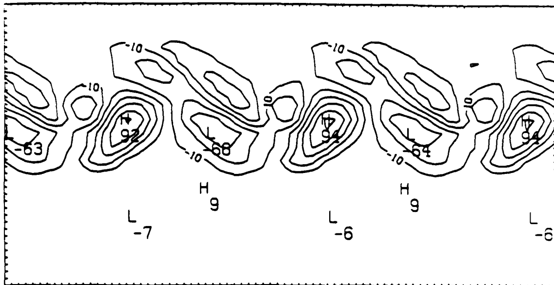
Figure 17 Truncation error estimate using equation 2.2 for the u velocity field at t = 72 hours on the \sigma = 0.3 surface. The estimate has been normalized by dividing by U = 10m/sec (dimensionless, \times 10^6 ).
