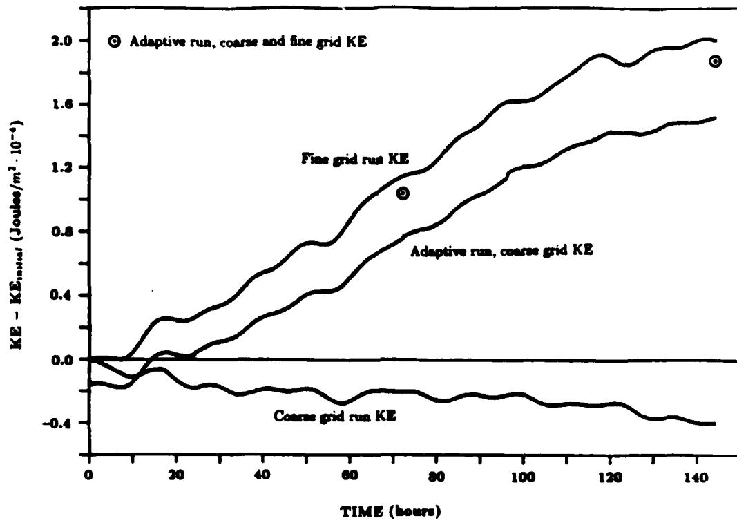
Figure 16 Horizontally averaged kinetic energy.
