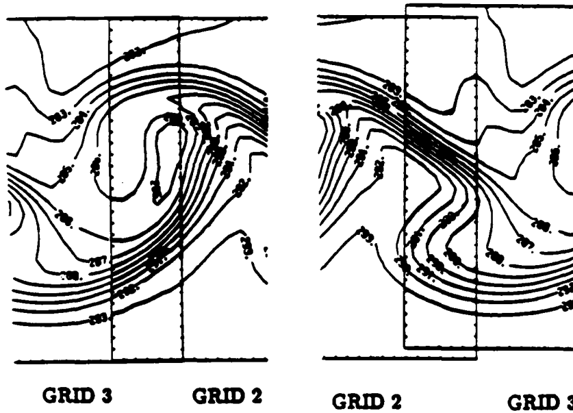
Figure 15 Temperature ( K ) on the \sigma = 0.9 surface at T = 72 hours for adaptive fine grids 3 (top), and the overlaps between fine grids 2 and 3 (bottom). The fine grids overlap in the center of the domain and also at the edges of the domain because of the periodic boundary conditions. The solutions agree in the overlap.
