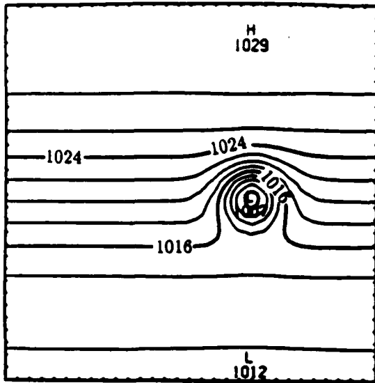
Figure 5 Initial conditions for the barotropic cyclone. Surface pressure is in millibars. Winds travel counterclockwise around the low pressure. The cyclone is advected towards the left by a zonal wind.
