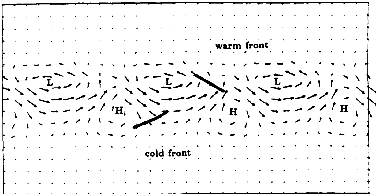
Figure 11 Velocity vectors on the \sigma = 0.9 surface at t = 0 . . Note the positions of the warm and cold fronts (shown in Figure 10) and the positions of the surface pressure highs and lows (shown in Figure 12) with respect to the wind fields.
