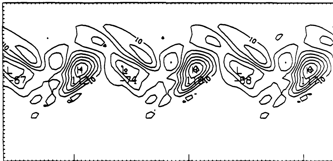
Figure 18 Truncation error estimate computed from the formulas in appendix 1 (dimensionless, \times 10^6 ). Normalized and nondimensionalized by multiplying by \Delta t / (\pi U) .
