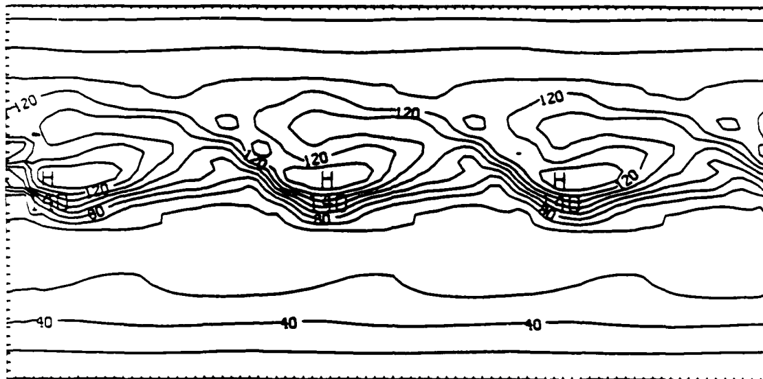
Figure 9 Absolute vorticity ( 10^{-6} \text{sec}^{-1} ) on the \sigma = 0.5 surface for the baroclinically unstable wave at t = 0 . of the adaptive run.
