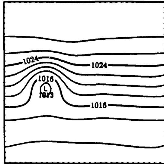
Figure 6 Cyclone after 3 days with the integration carried out on the coarse grid with \Delta x = 180 \text{ km}
