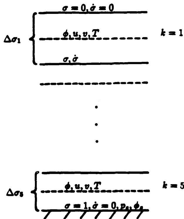
Figure 4 Vertical structure of the finite difference grid in the sigma ( \sigma ) coordinate system for a 5 level model.
