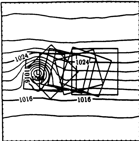
Figure 7 Cyclone after 3 days using adaptive model. There is only a single fine grid in the region at any time. \Delta x_{\text{coarse}} = 180 \text{ km} , \Delta x_{\text{fine}} = 60 \text{ km} . Fine grids used in the calculation are displayed.
