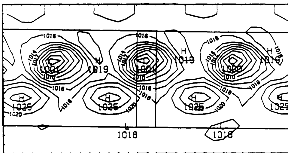
Figure 13 Surface pressure in millibars at T = 72 hours. Location of the fine grids in the adaptive calculation at T = 72 hours are shown in the adaptive coarse grid plot.
