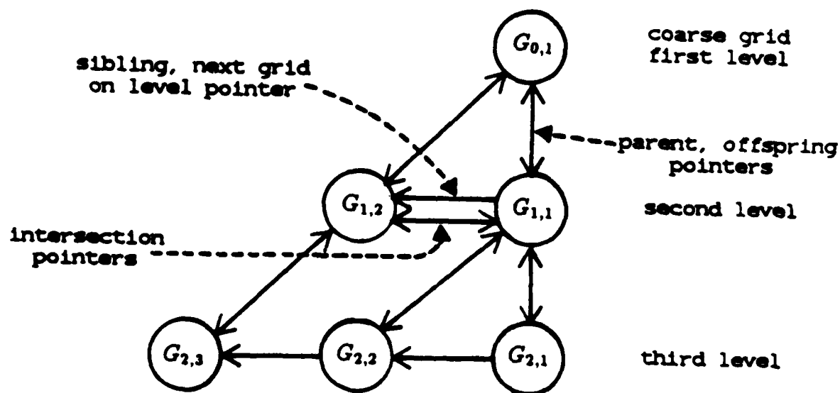
Figure 2 Tree for grids of Figure 2. Included are some of the pointers listed in the text.
